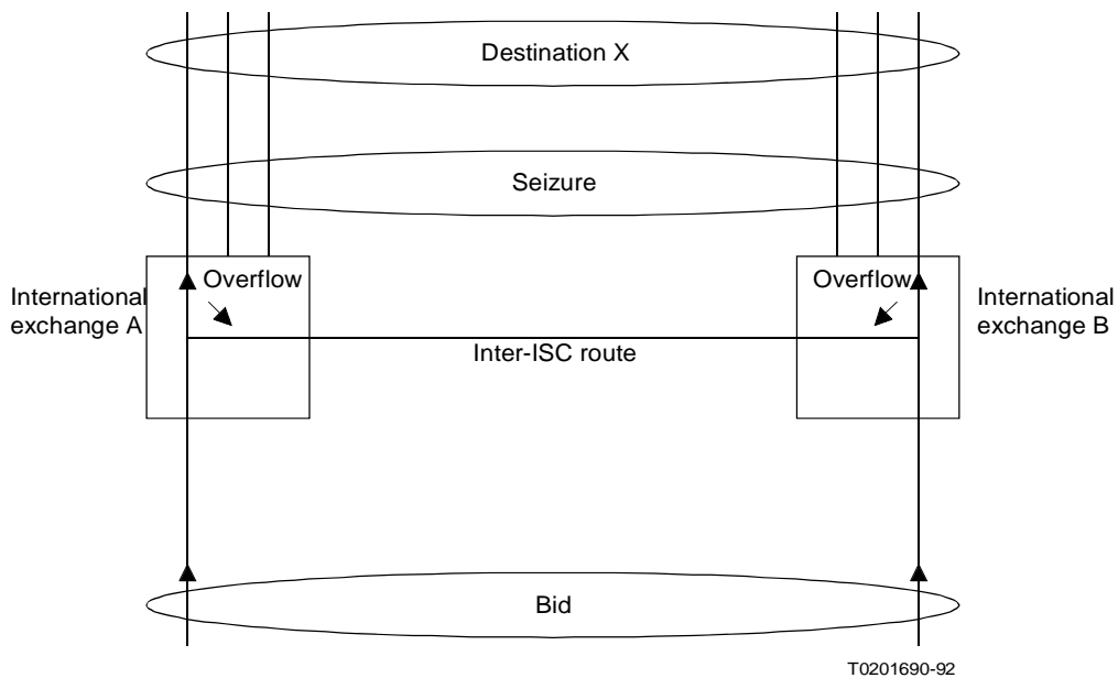
FIGURE 2/E.503 Example of multi-ISC operation
