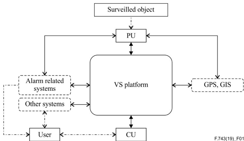
Figure 1 – VSS model
