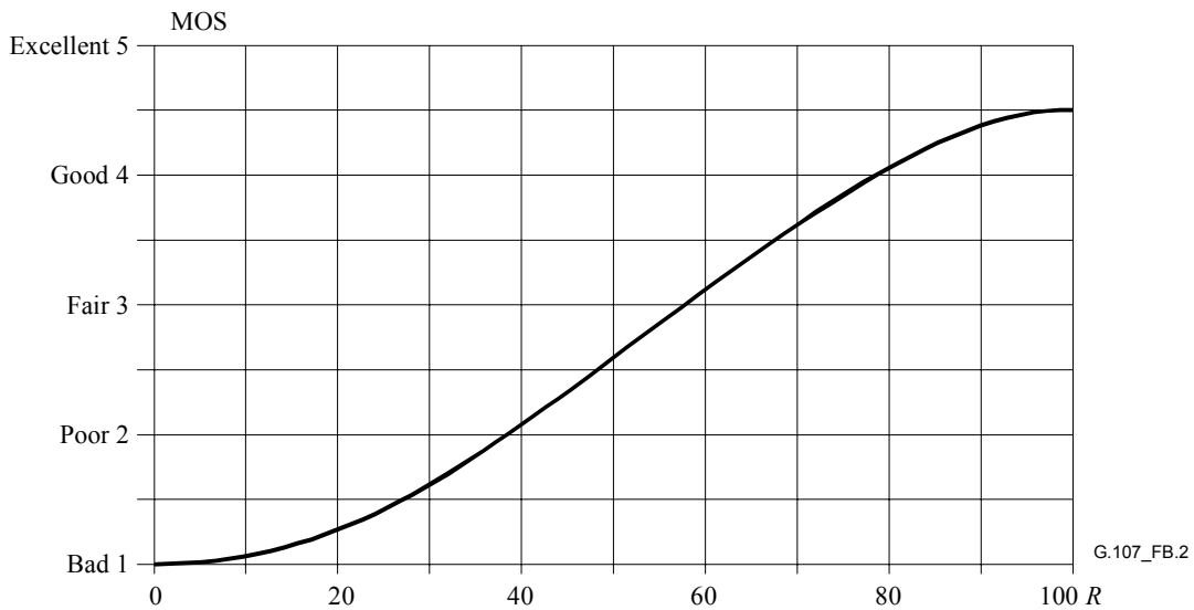
Figure B.2/G.107 – MOS_{CQE} as function of rating factor R
