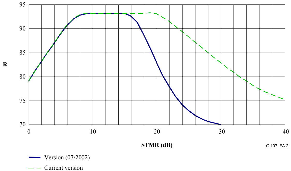
Figure A.2/G.107 – Comparison of R vs STMR for the current and the previous versions of the E-model algorithm
