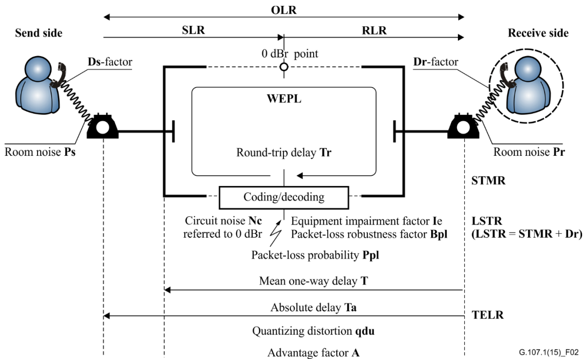
Figure 2 – Reference connection of the WB E-model
