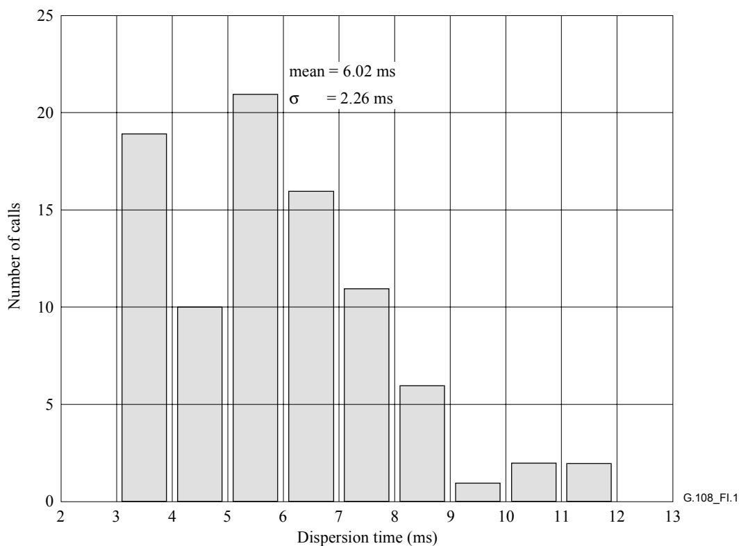
Figure I.1/G.108.2 – Histogram of dispersion time for long-distance calls
