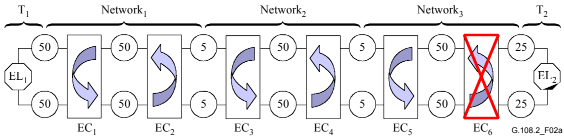
Figure 2a/G.108.2 – Example of connection via three concatenated networks including a cellular network
