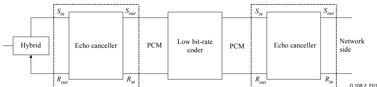
Figure 1/G.108.2 – Low bit-rate coder between tandem cancellers
