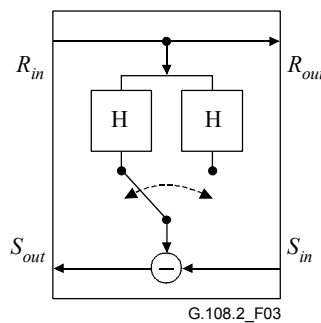
Figure 3/G.108.2 – Possible implementation of echo canceller with two independent H echo path estimators
