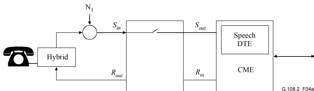
Figure 4a/G.108.2 – Speech detector/echo control device interaction
