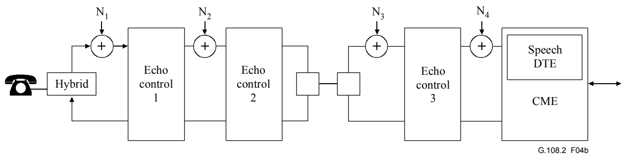
Figure 4b/G.108.2 – Multiple echo control devices in a CME network configuration
