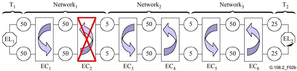
Figure 2b/G.108.2 – Example of connection via three concatenated networks including a private network
