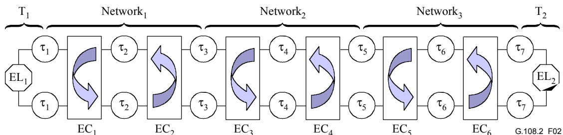
Figure 2/G.108.2 – Reference connection for tandem ECs
