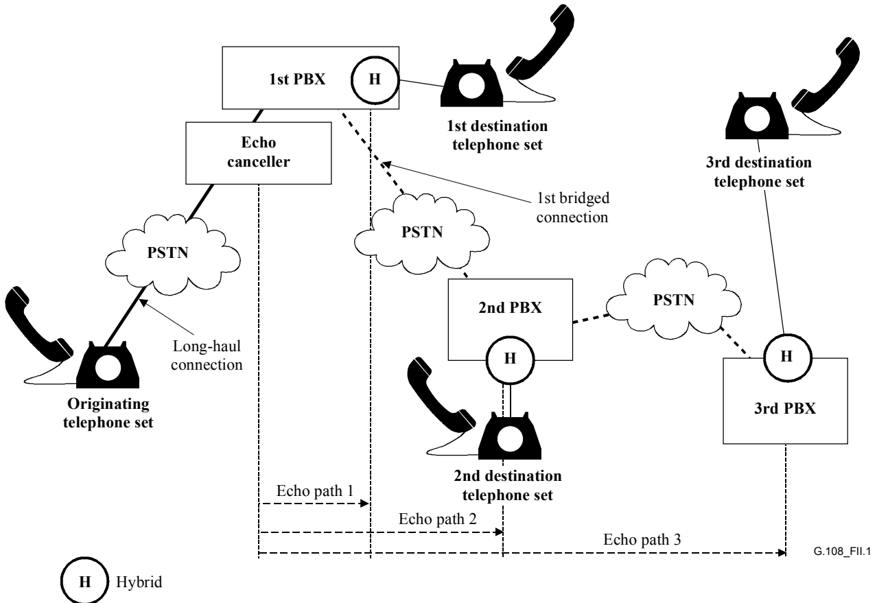
Figure II.1/G.108.2 – Multiple tails in a typical bridged telephone call
