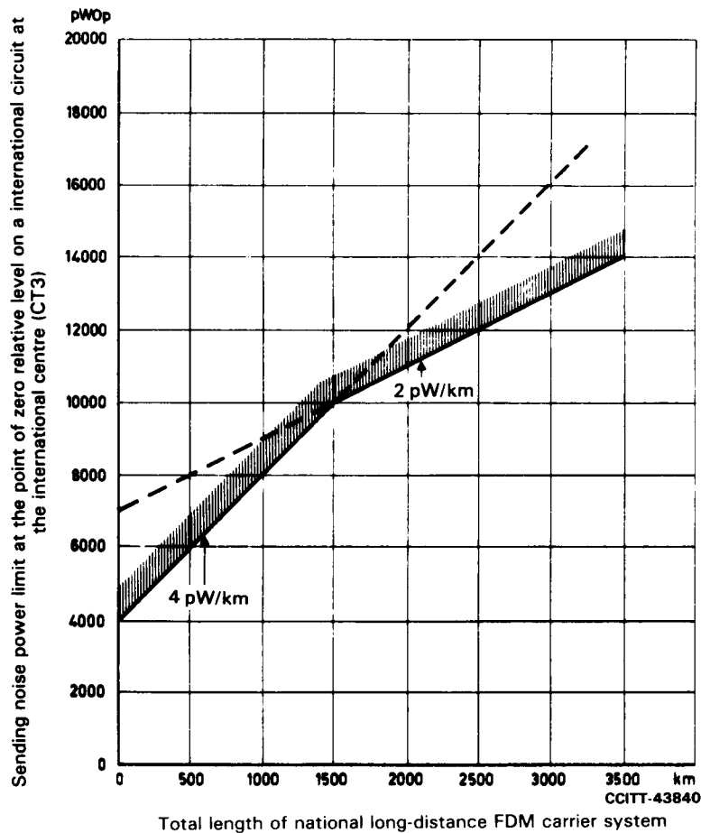
FIGURE A-2/G.123
