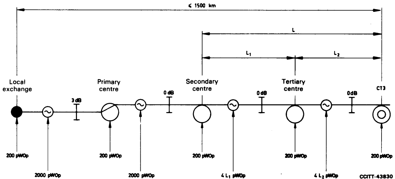
FIGURE A-1/G.123
