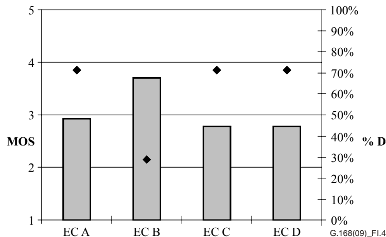
Figure I.4 – Results from conversational tests , overall quality MOS and % D (rhombus) for the 4 echo cancellers, ERL 7 dB, room noise level 40 dB(A), corresponding level –61 dBm0
