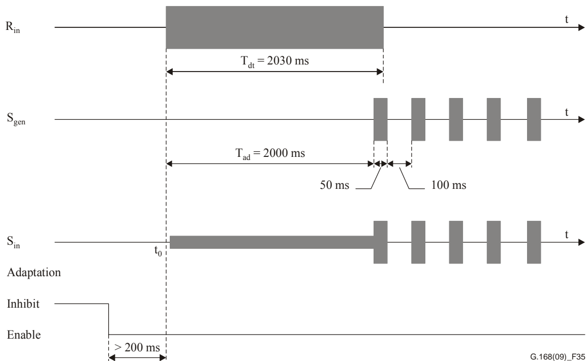
Figure 35 – Test timing version 2: a 'typical' DTMF reaction and an almost instantaneous removal of the dial tone upon detection of the first DTMF digit by the system
