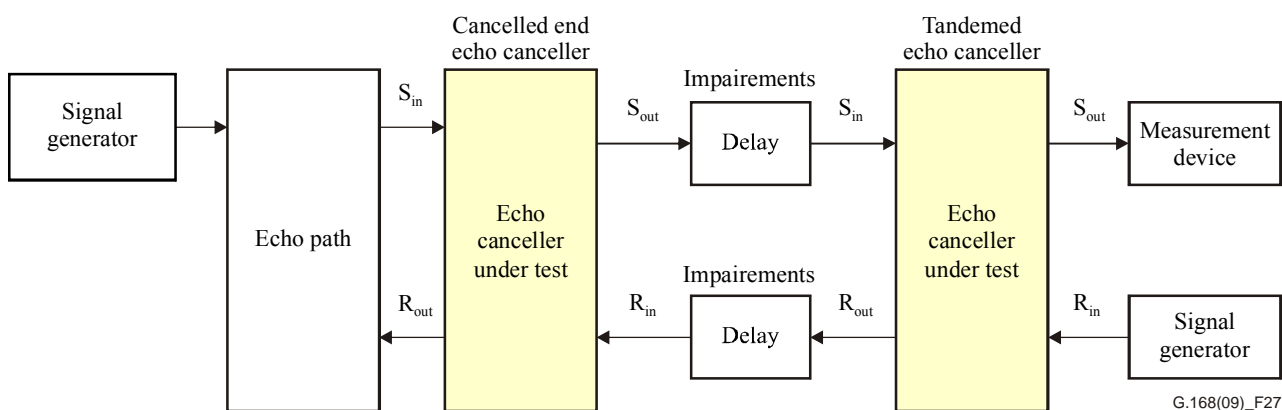
Figure 27 – Test No. 11 configuration
