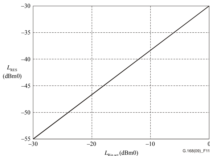
Figure 11 – Relationship between receive input level ( L_{\text{Rin,act}} ) and residual echo level ( L_{\text{RES}} ) with NLP disabled
