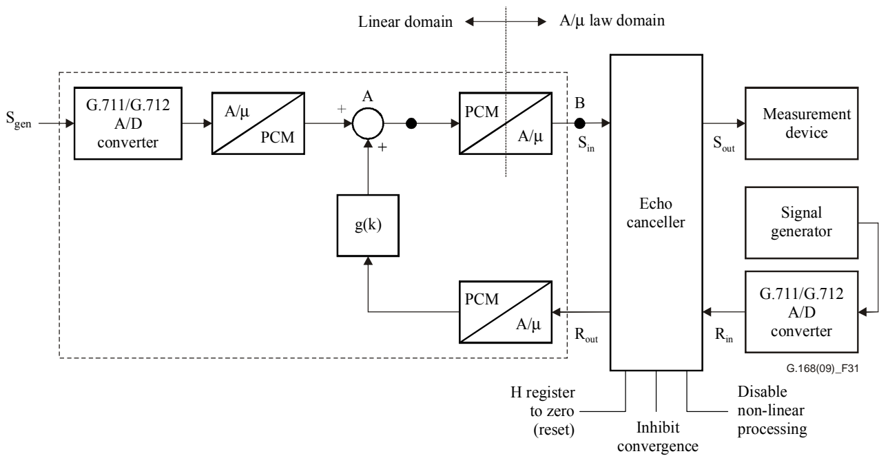
Figure 31 – Test configuration for S_{in} PCM offset test
