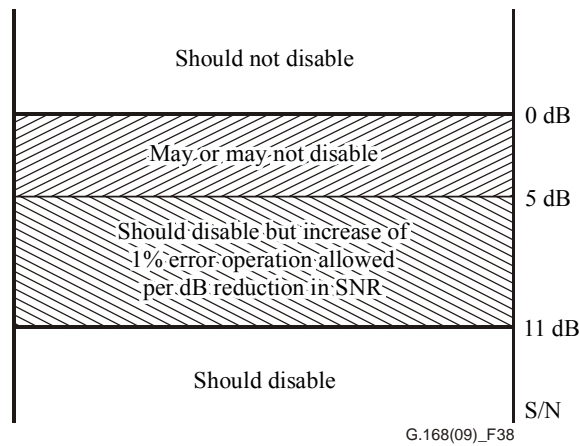
Figure 38 – Guardband and noise tolerance requirements
