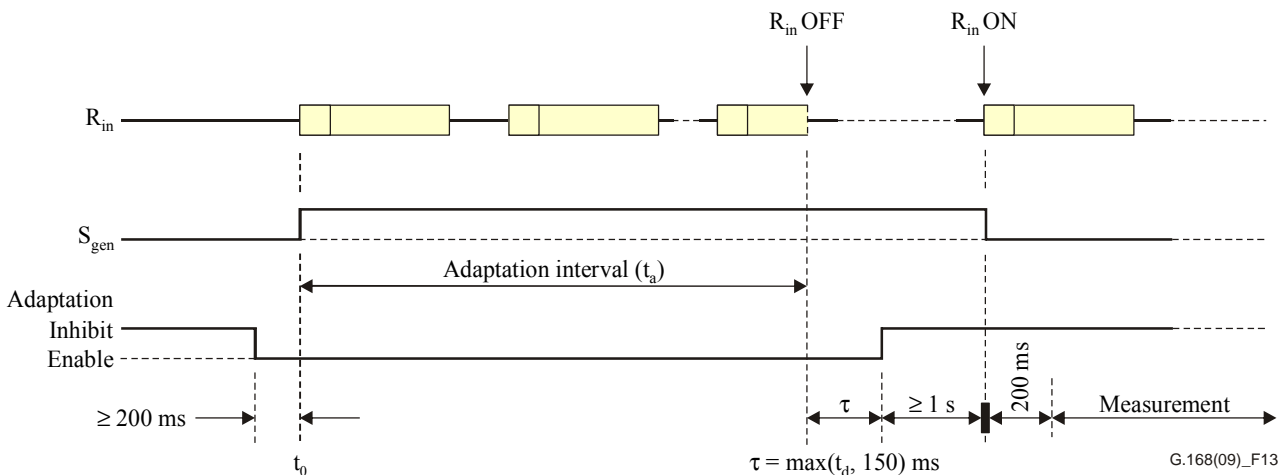
Figure 13 – Test No. 2C signal and time relationships
