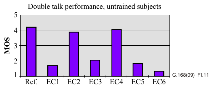
Figure I.11 – Results from listening-only tests, untrained subjects, double talk performance MOS, ERL 24 dB, receive level –15 dBm0, double talk level –30 dBm0
