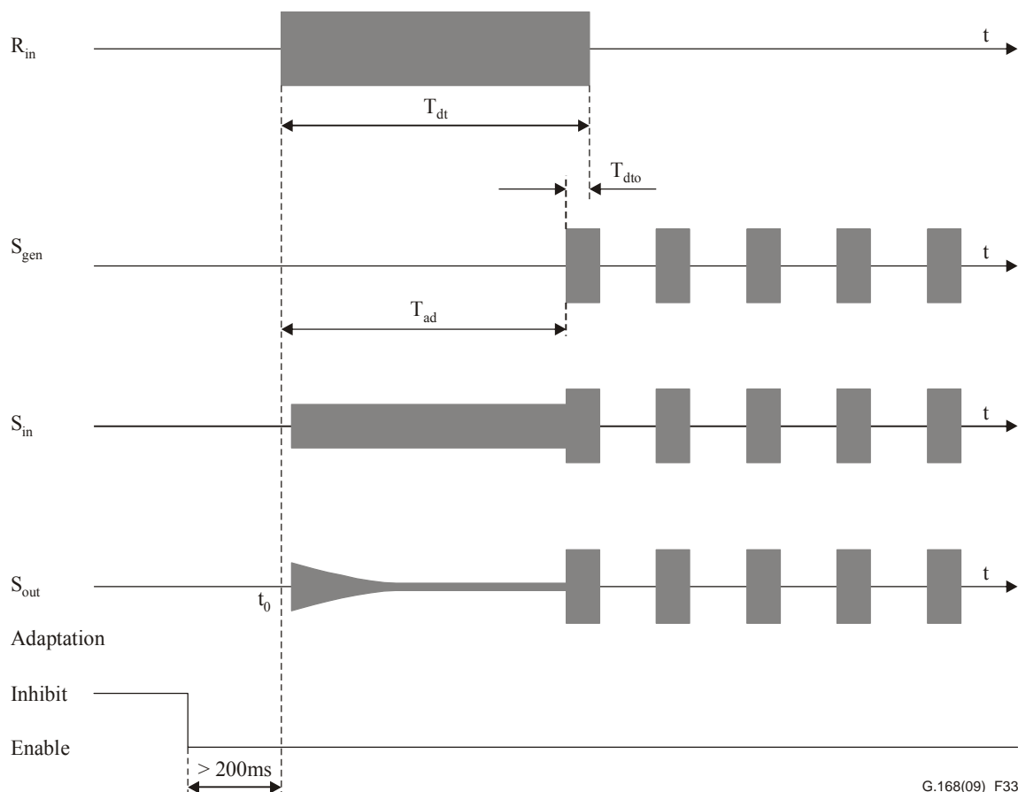
Figure 33 – Illustration of requirements for DTMF transparency in the presence of dial tone
