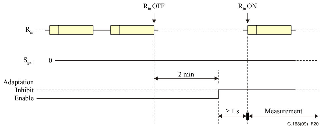
Figure 20 – Test No. 4 signal and time relationships
