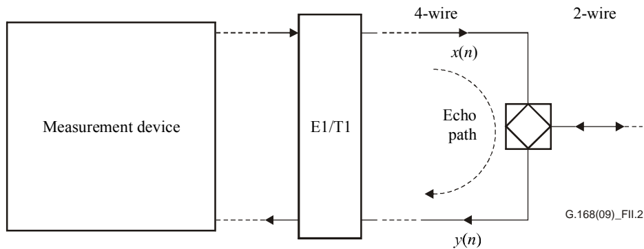
Figure II.2 – Block diagram of intrusive measurement set-up
