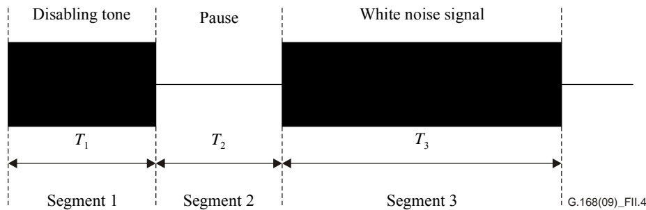
Figure II.4 – Test signal for echo-path measurement
