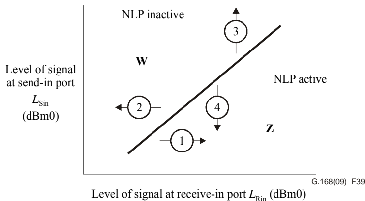
Figure 39 – NLP operating regions
