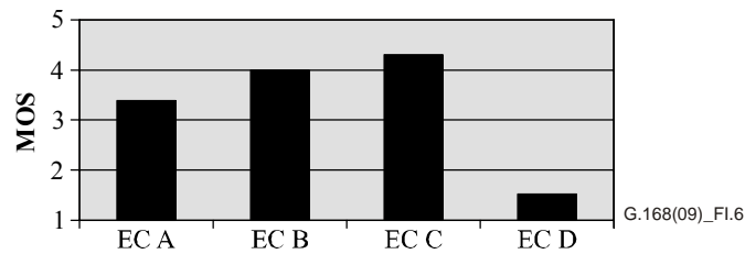
Figure I.6 – Results from talking and listening tests , MOS, disturbance caused by echoes, digital echo path, ERL 6 dB, no cancelled end background noise, NLP disabled
