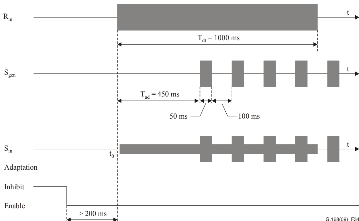
Figure 34 – Test timing version 1: 'fast' DTMF reaction and a 'slow' removal of the dial tone
