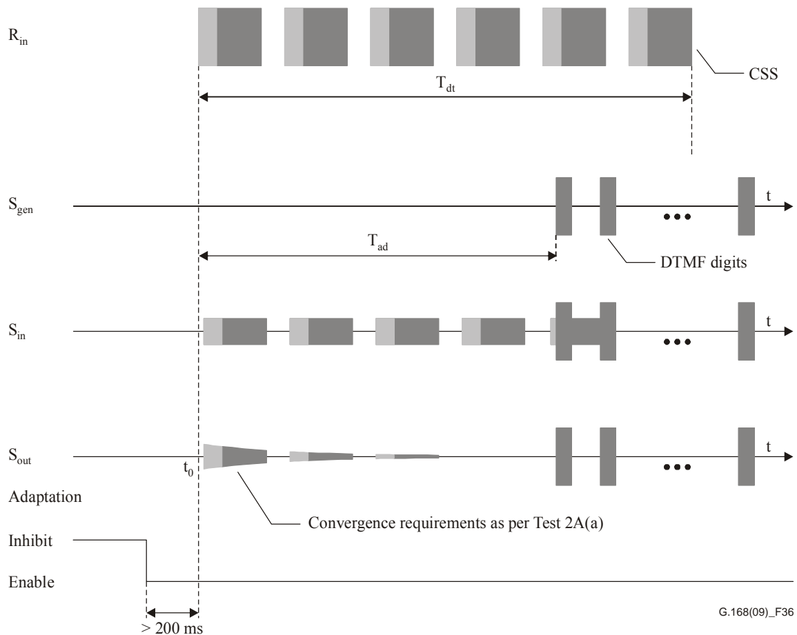
Figure 36 – Illustration of requirements for DTMF transparency in the presence of CSS
