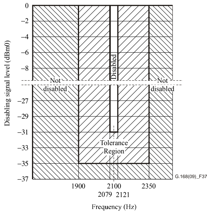
Figure 37 – Required disabling band characteristics
