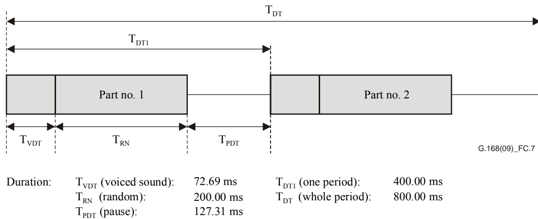
Figure C.7 – Composite source signals to simulate double talk (schematic)
