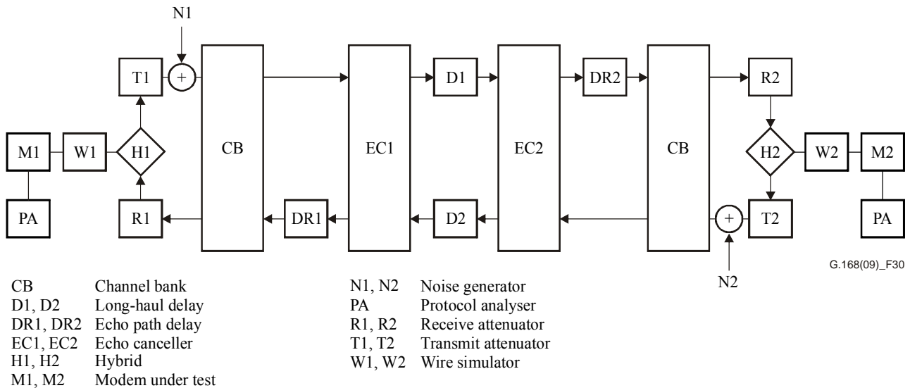
Figure 30 – Test No. 14 configuration
