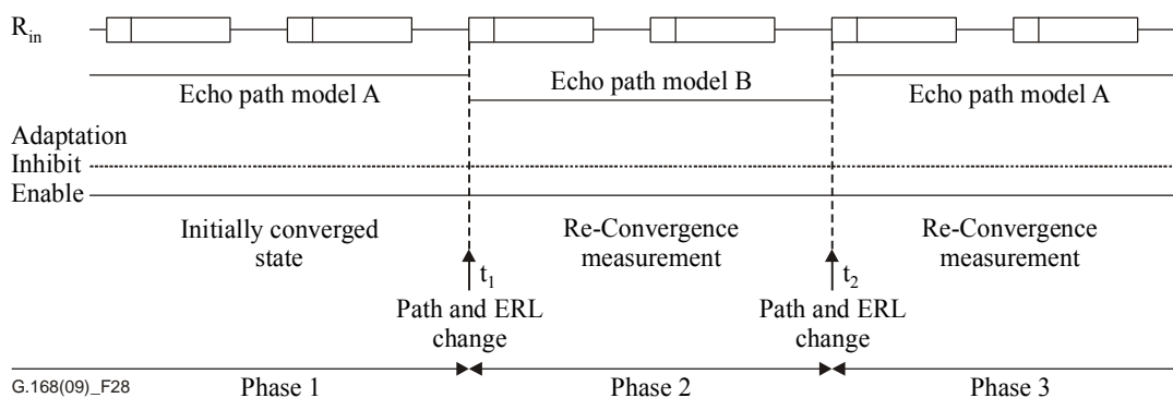
Figure 28 – A conversation scenario with acoustic echo
