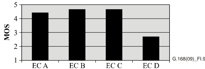
Figure I.9 – Results from talking and listening tests , MOS, disturbance caused by audible switching, digital echo path, ERL 6 dB, background noise –55 dBm0, NLP enabled
