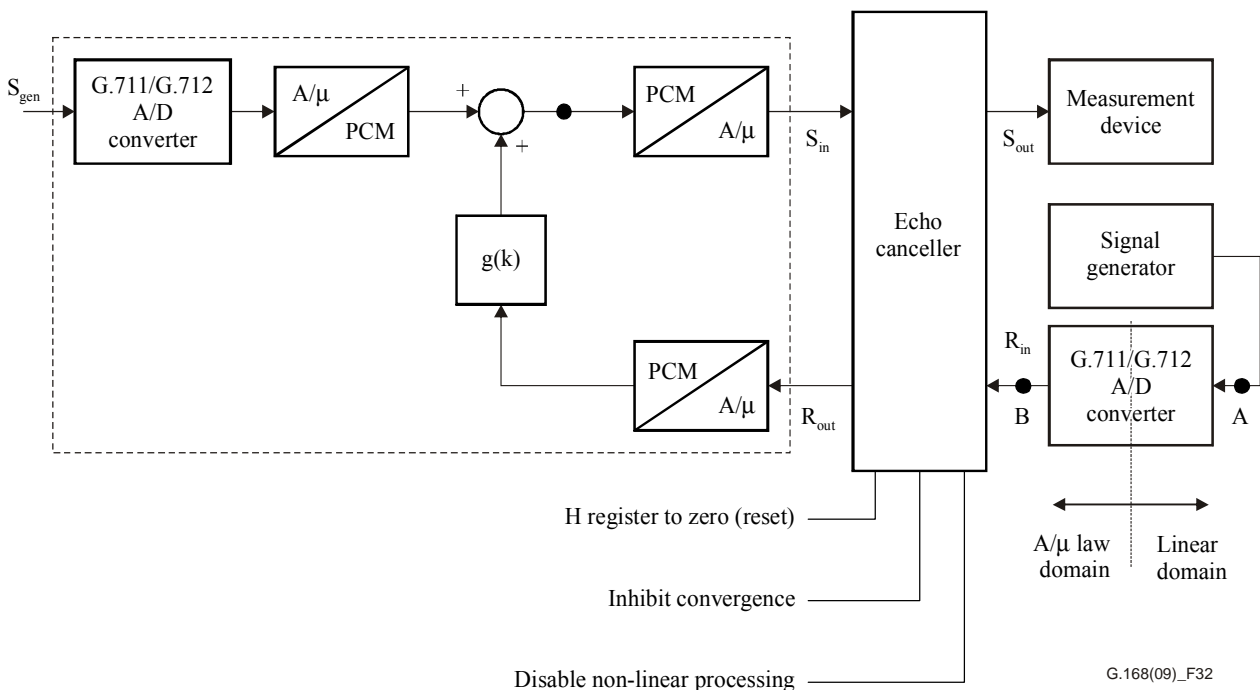
Figure 32 – Test configuration for R_{in} PCM offset test
