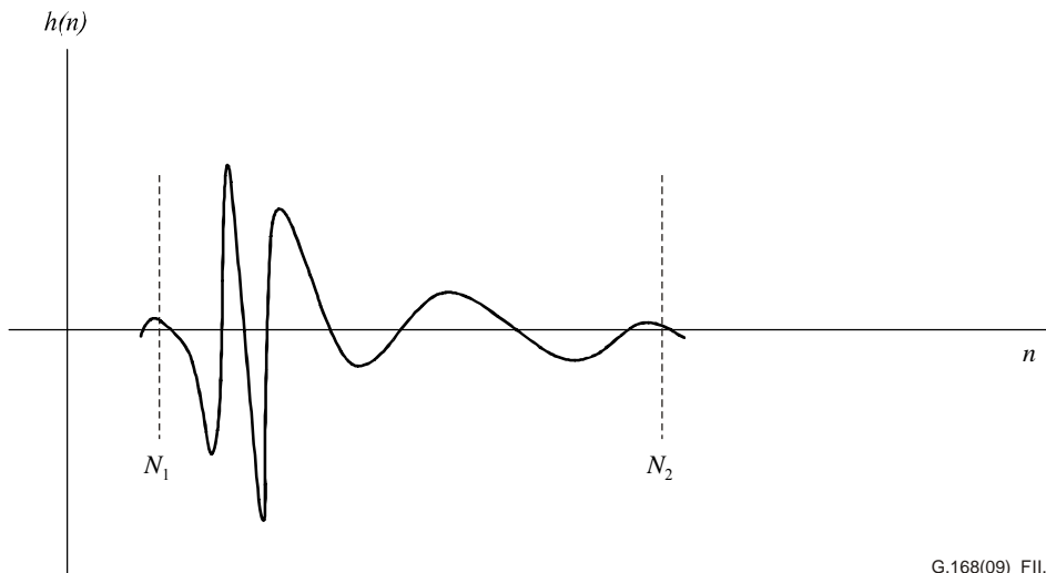
Figure II.5 – Echo-path truncation for dispersion time estimate
