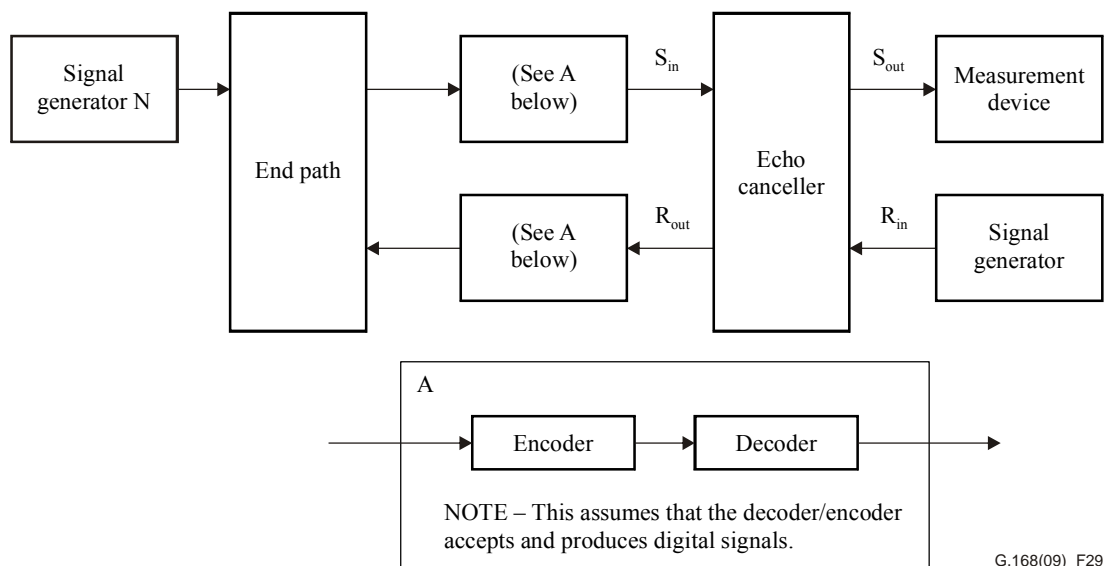
Figure 29 – Test No. 13 configuration
