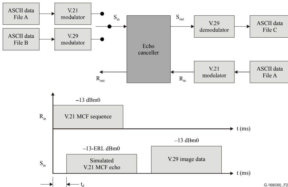
Figure 26 – Cancellor operation during page transmission and page breaks
