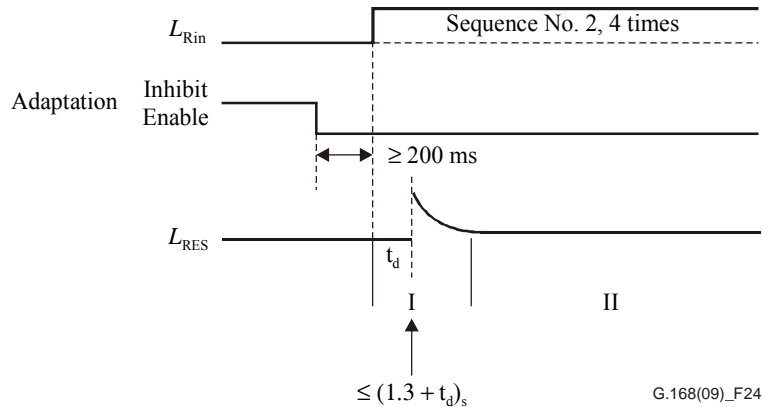
Figure 24 – Test No. 10B signal and time relationships
