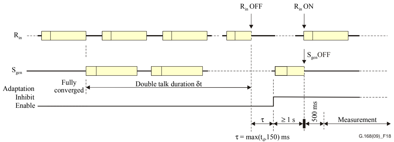
Figure 18 – Test No. 3B signal and time relationships
