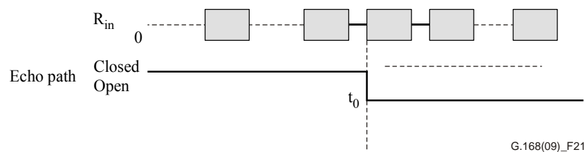
Figure 21 – Test No. 5 signal and time relationships
