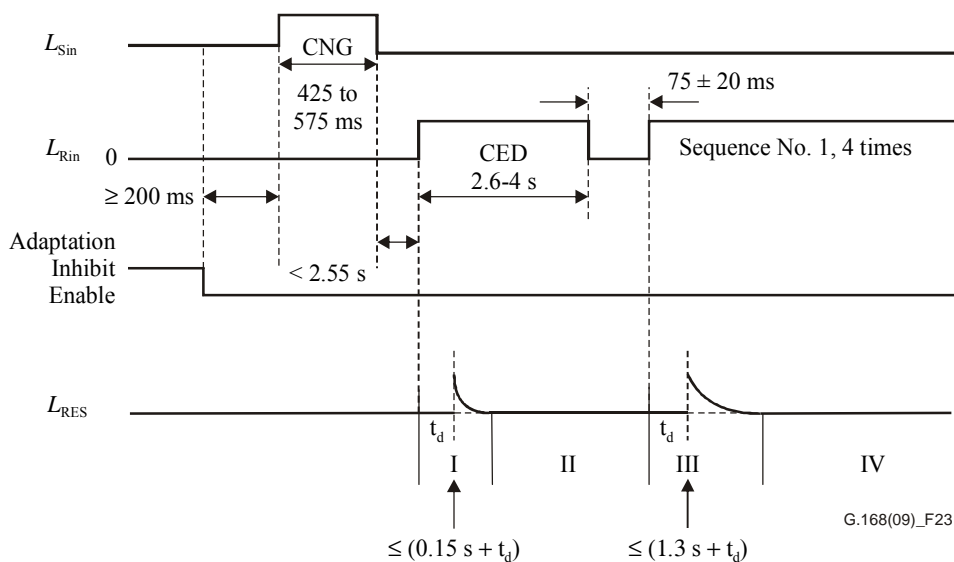
Figure 23 – Test No. 10A signal and time relationships
