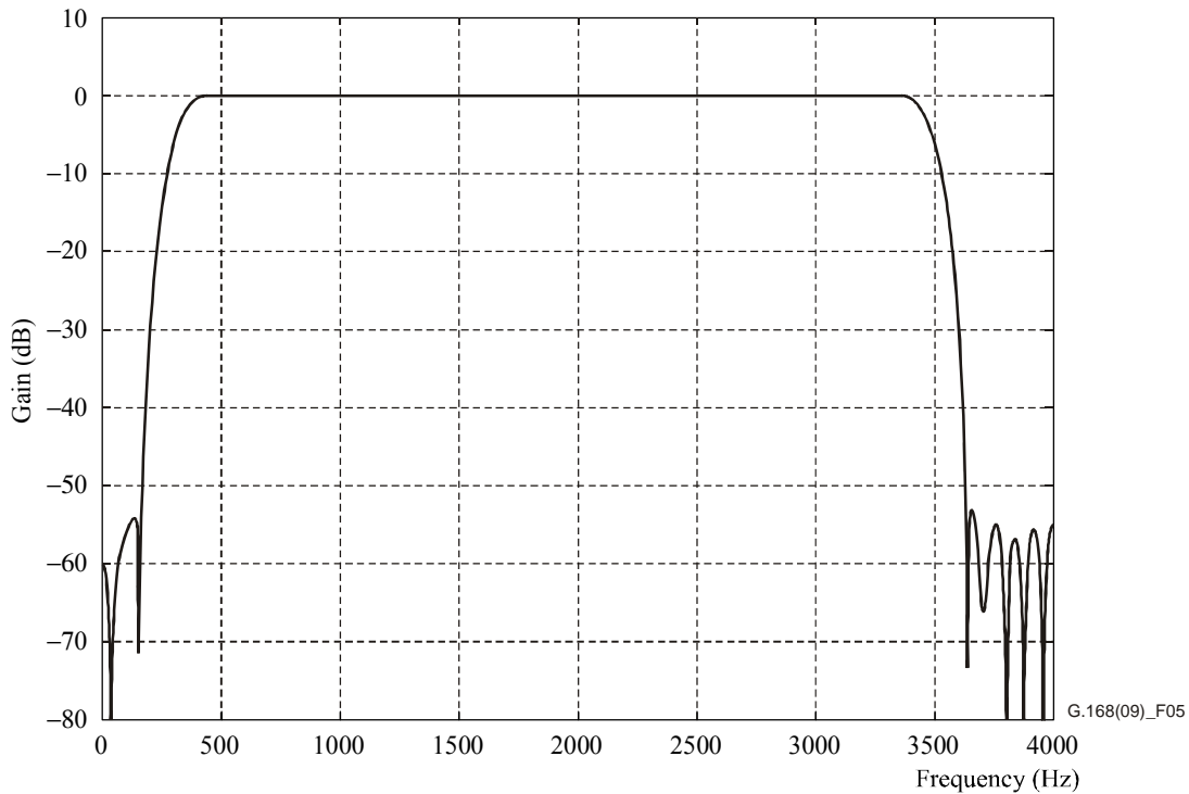
Figure 5 – Magnitude response of frequency weighting network
