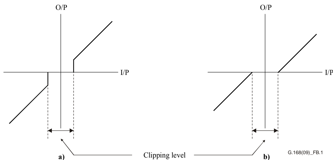
Figure B.1 – Two examples of idealized centre clipper transfer function
