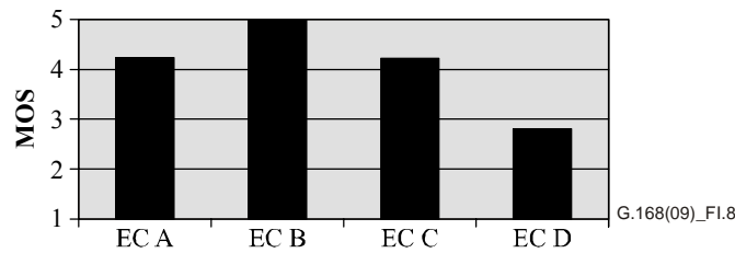
Figure I.8 – Results from talking and listening tests , MOS, disturbance caused by echoes, digital echo path, ERL 6 dB, background noise –55 dBm0, NLP enabled
