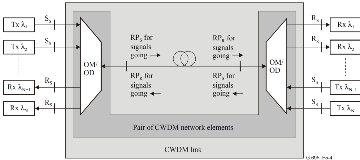
Figure 5-4/G.695 – "Black Link" approach for bidirectional applications
