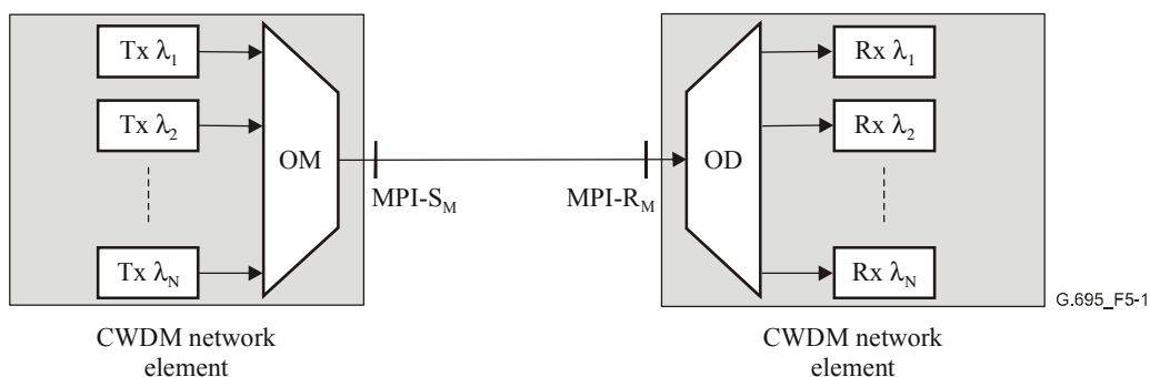
Figure 5-1/G.695 – "Black-box" approach
