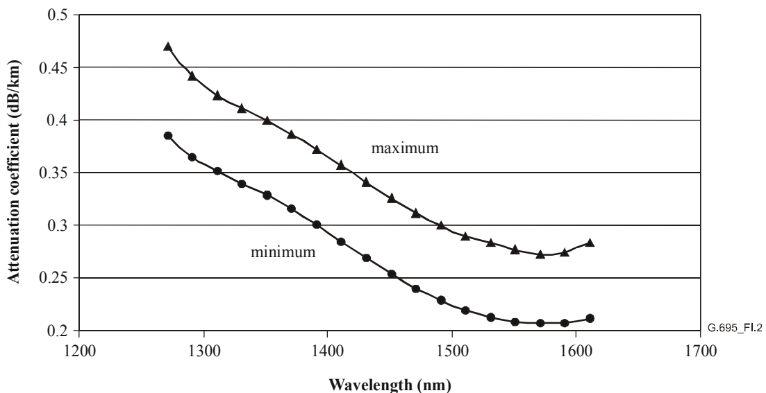
Figure I.1/G.695 – Assumed attenuation coefficient values for G.652.A and B cable
