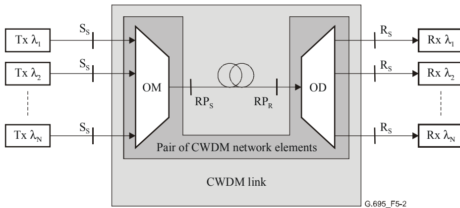
Figure 5-2/G.695 – "Black-link" approach
