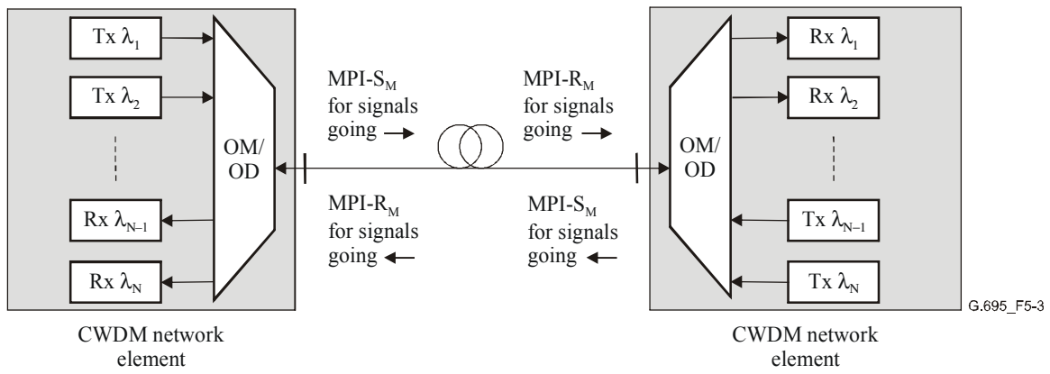
Figure 5-3/G.695 – "Black Box" approach for bidirectional applications
