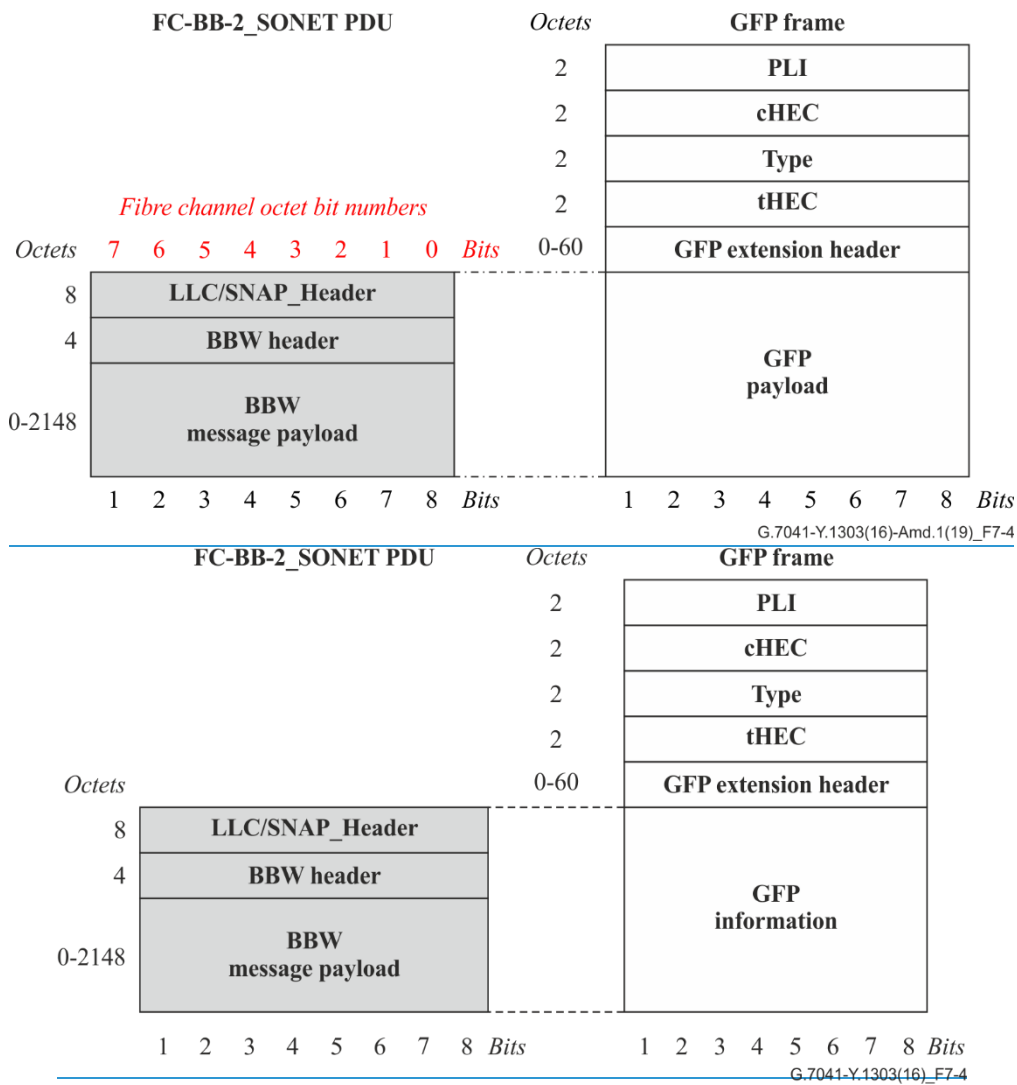
Figure 7-4 – Fibre channel broadband-2 SONET (FC-BBW_SONET) and GFP frame relationships
