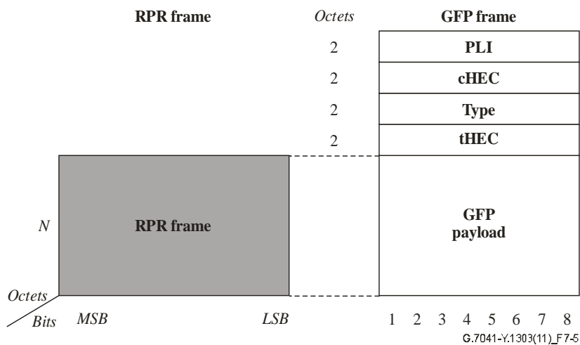
Figure 7-5 – RPR and GFP frame relationships
