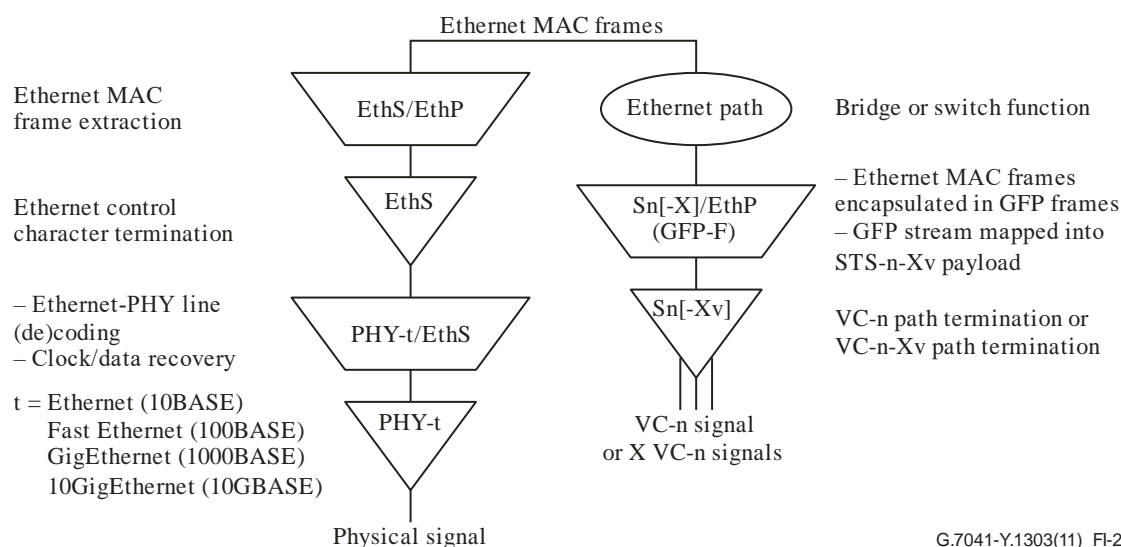
Figure I.2 – Ethernet tributary interface port using GFP-F mapping in an SDH network element
