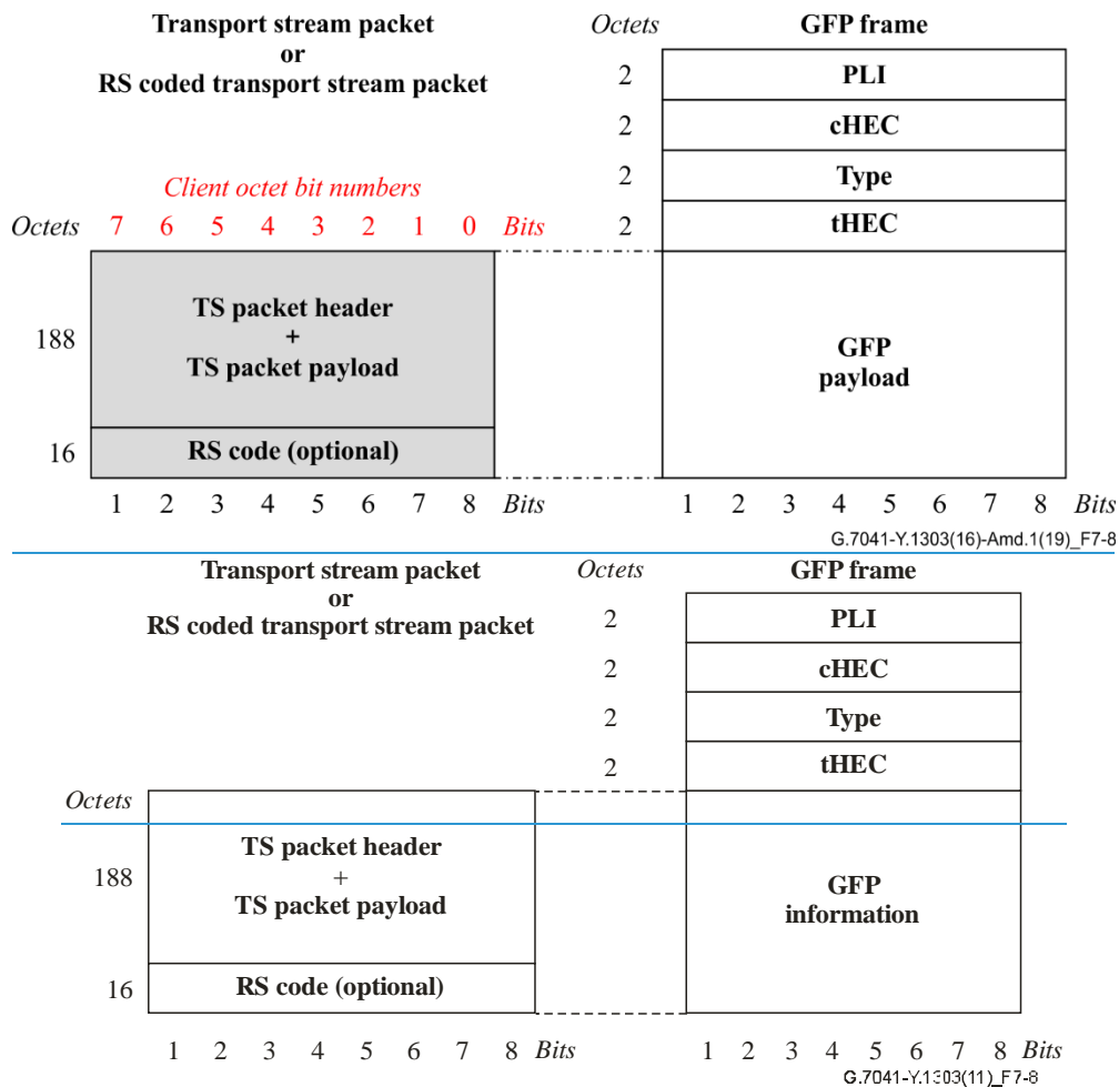
Figure 7-8 – TS packet and GFP frame relationships
