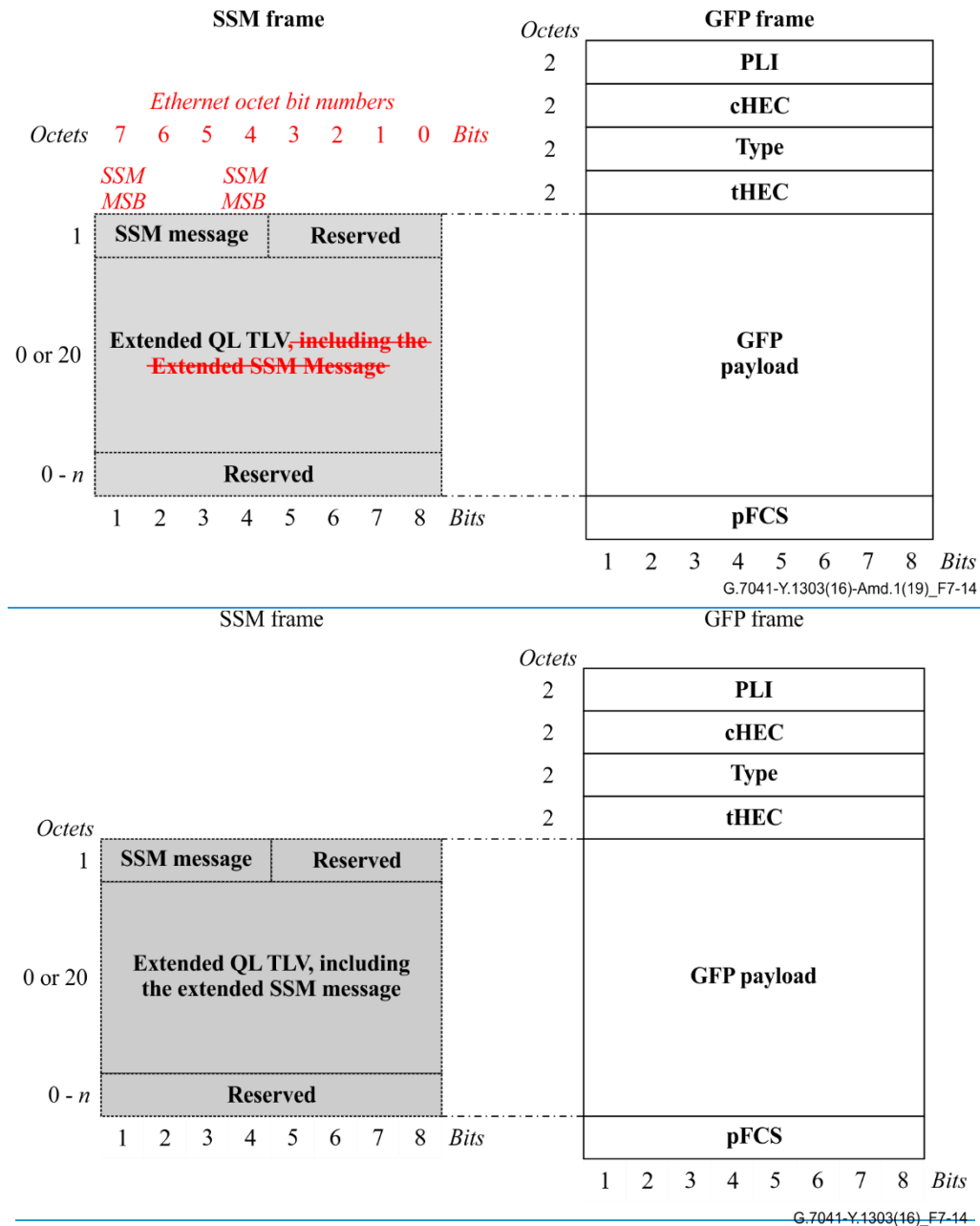
Figure 7-14 – SSM mapping into GFP-F
