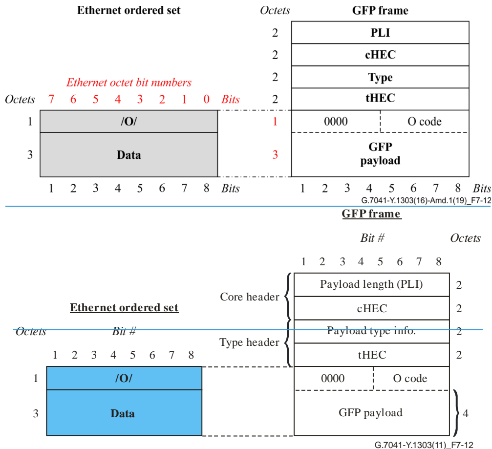
Figure 7-12 – Ethernet ordered set mapping into GFP-F
