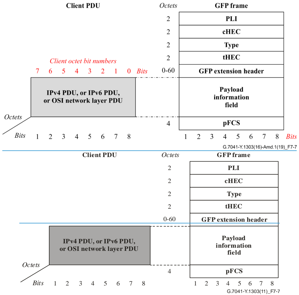
Figure 7-7 – IPv4/IPv6/OSI network layer PDUs and GFP frame relationships
