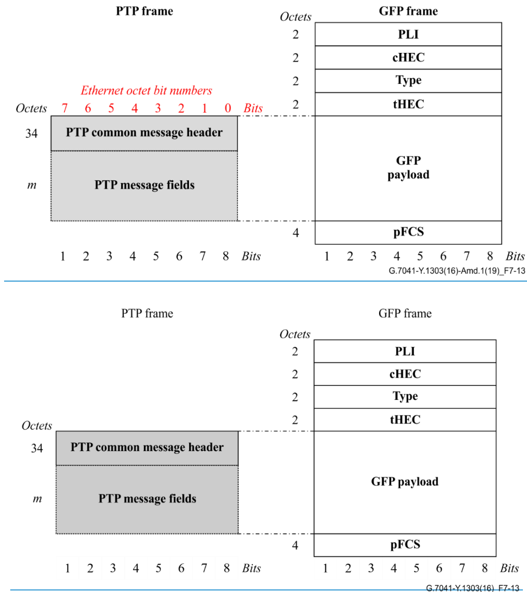
Figure 7-13 – PTP message mapping into GFP-F
