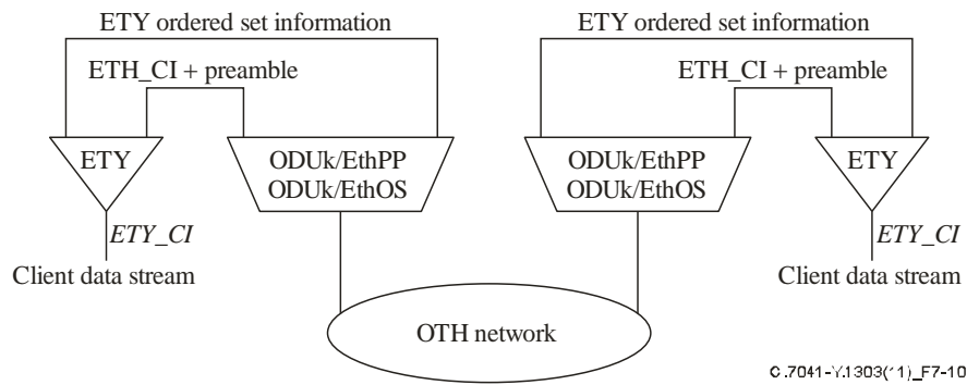
Figure 7-10 – Functional model for mapping 10GBASE-R information into the ODUk
