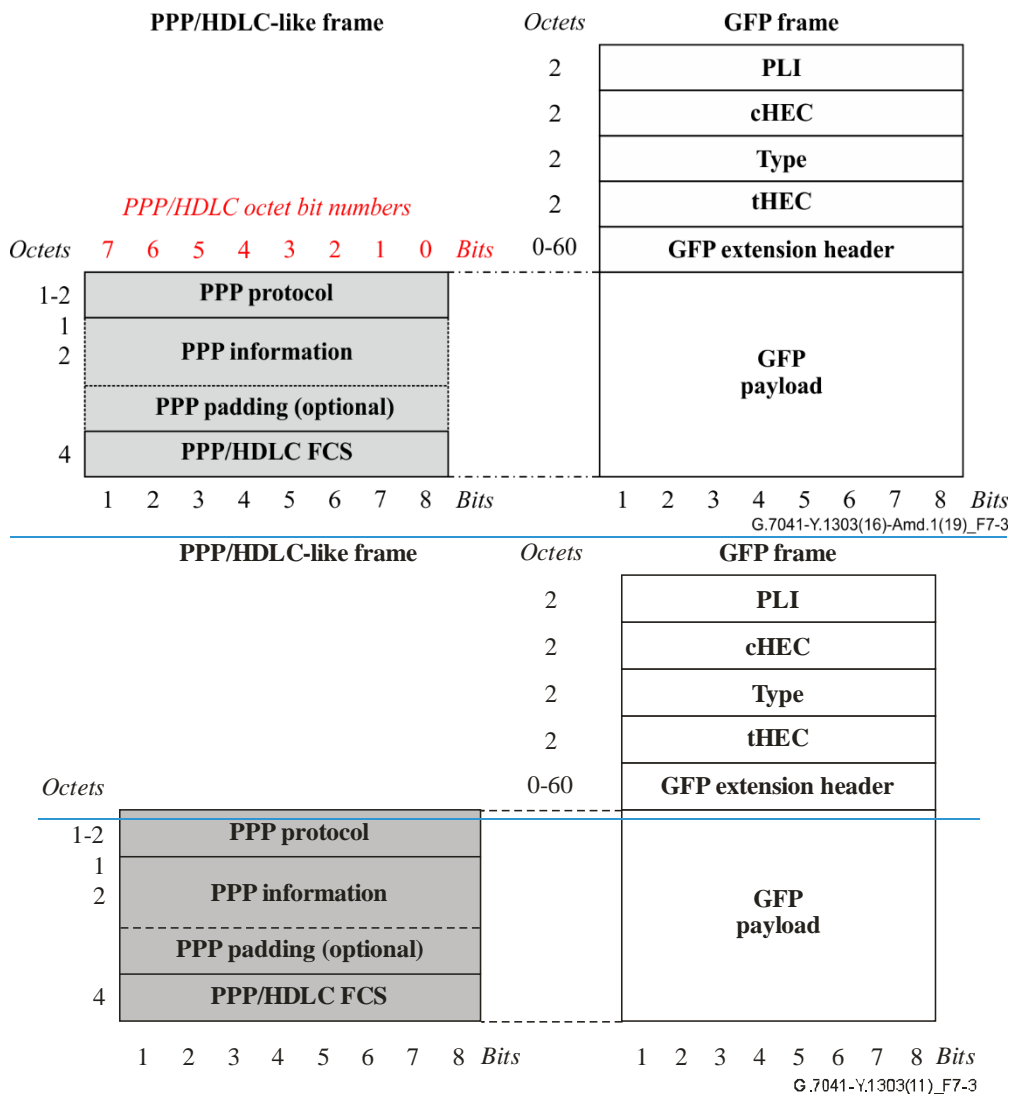
Figure 7-3 – PPP/HDLC and GFP frame relationships (with PPP's ACFC configuration option)
