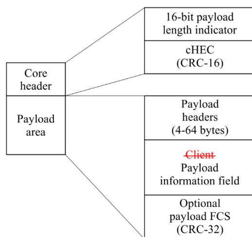
Figure 6-1 – Frame format for GFP client frames
