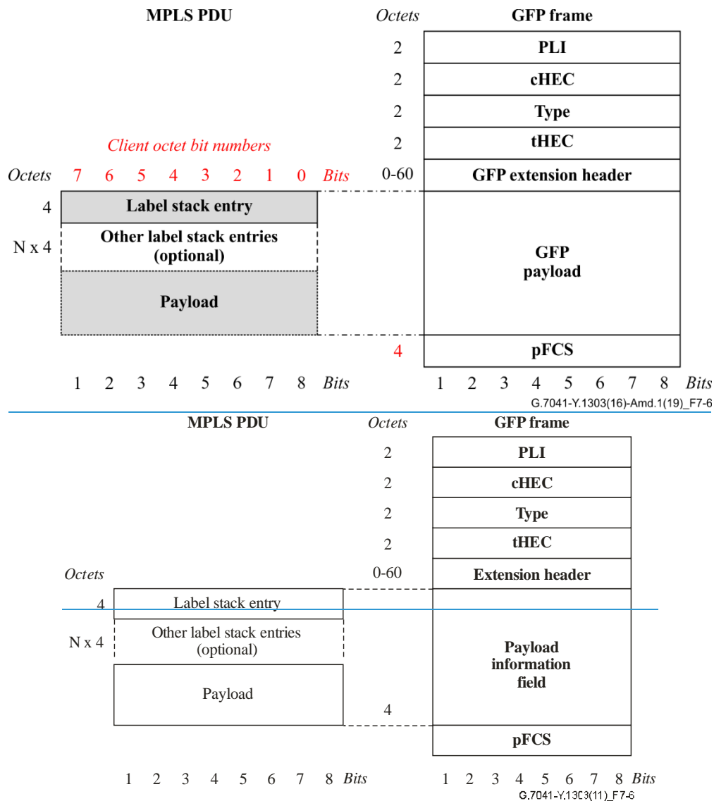
Figure 7-6 – MPLS PDU and GFP frame relationships
