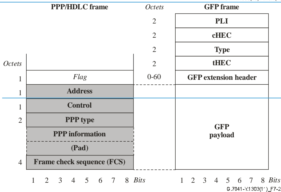
Figure 7-2 – HDLC/PPP and GFP frame relationships
