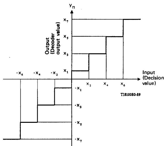
FIGURE 1/G.733
