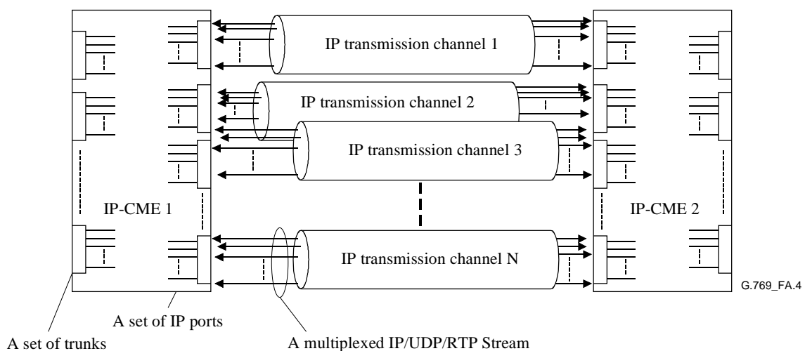
Figure A.4/G.769/Y.1242 – Configuration of the RTP connection between the IP-CMEs
