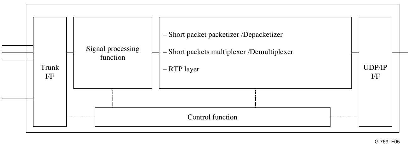
Figure 5/G.769/Y.1242 – Basic functions related to audio stream handling
