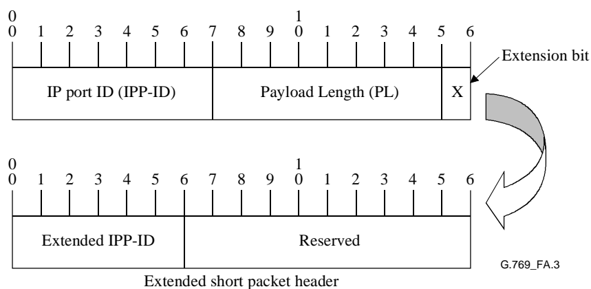
Figure A.3/G.769/Y.1242 – Format of the short packet header
