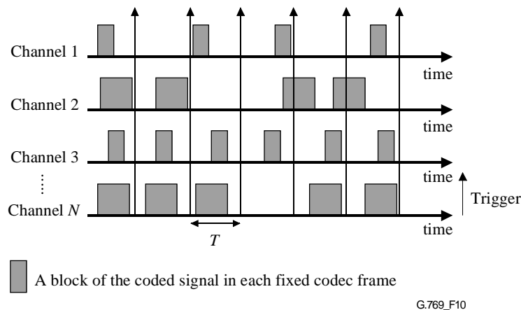
Figure 10/G.769/Y.1242 – Multiplexing and packetization by triggers of periodical timer
