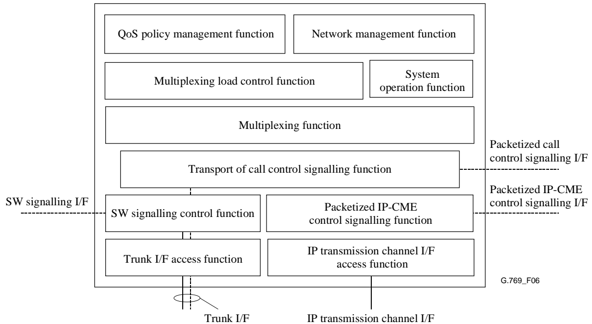
Figure 6/G.769/Y.1242 – Functions of the IP-CMEs
