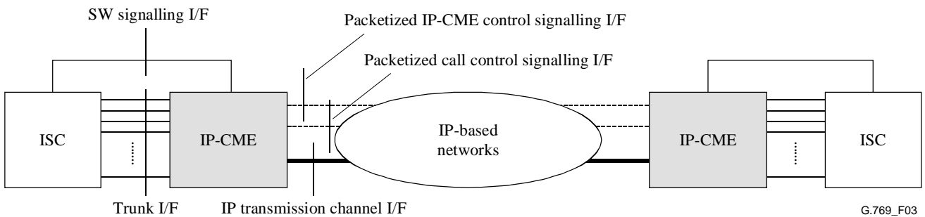
Figure 3/G.769/Y.1242 – Network connection interfaces of the IP-CME
