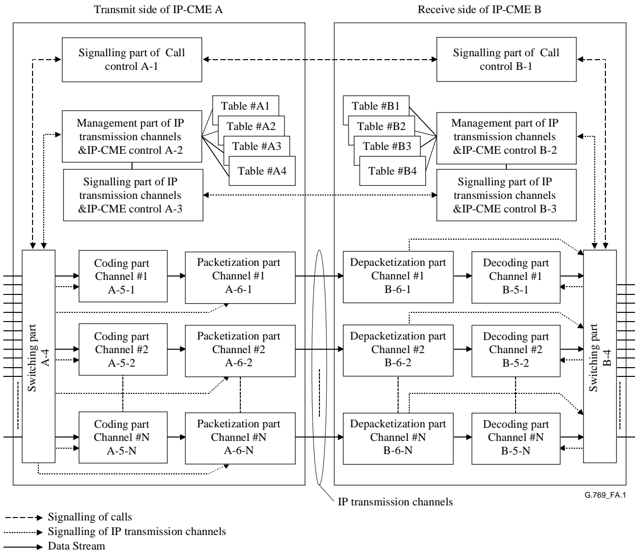
Figure A.1/G.769/Y.1242 – Conceptual block diagram of IP transmission channel control
