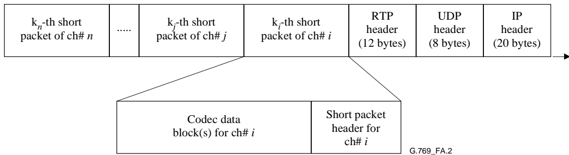
Figure A.2/G.769/Y.1242 – IP packet structure and short packet header elements
