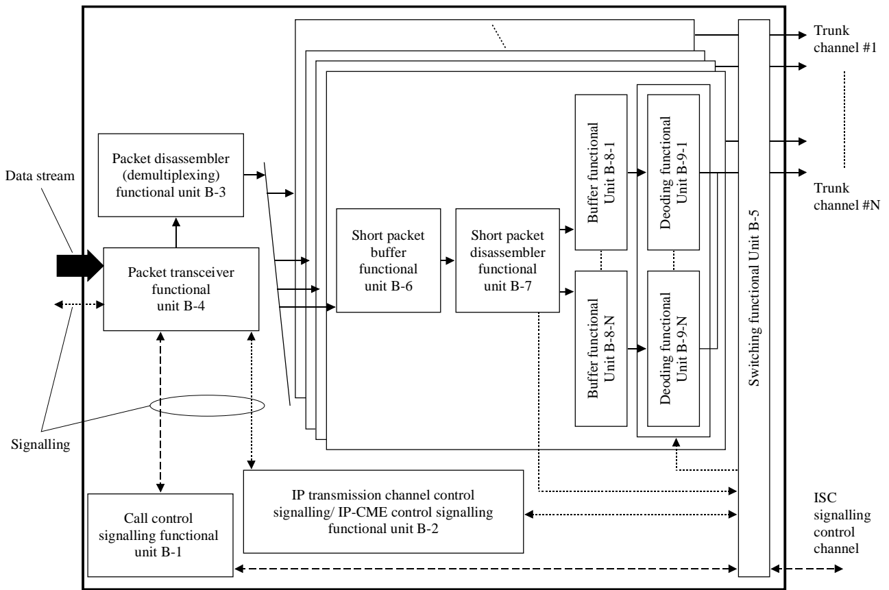
Figure I.2/G.769/Y.1242 – Example of block diagram of multiplication in Receive side of IP-CME
