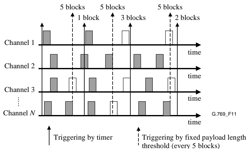
Figure 11/G.769/Y.1242 – The packetization mechanism in Scheme 4
