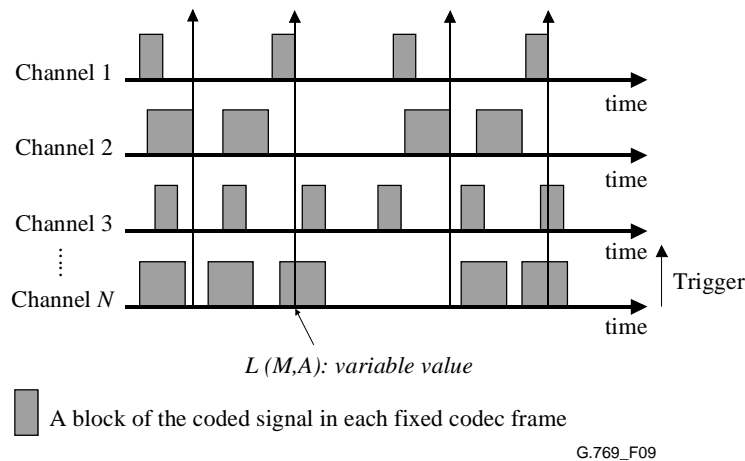
Figure 9/G.769/Y.1242 – Multiplexing and packetization by triggers of dynamic payload length threshold
