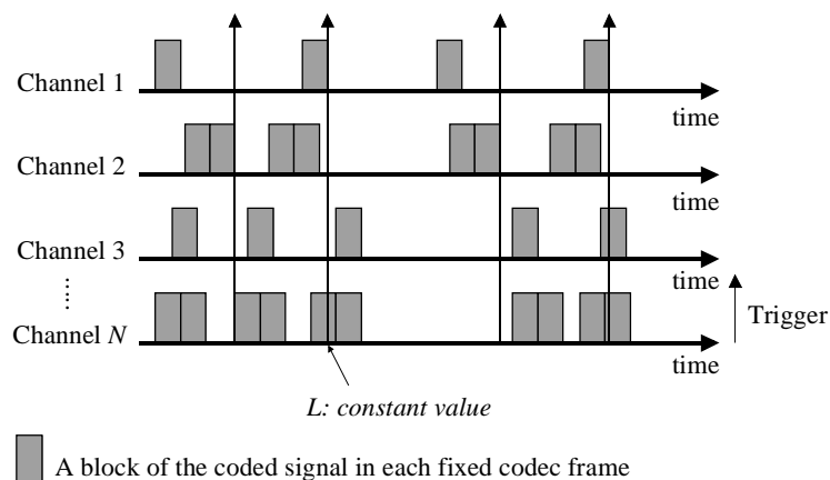
Figure 8/G.769/Y.1242 – Multiplexing and packetization by triggers of fixed payload length threshold
