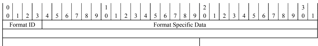
Figure 3/G.7714.1/Y.1705.1 – General Discovery Message format
