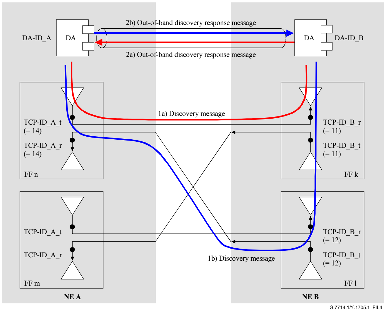
Figure II.4/G.7714.1/Y.1705.1 – Auto discovery in case of miswired interfaces
