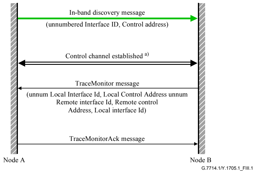
Figure III.1/G.7714.1/Y.1705.1 – Summary of discovery messages used in GMPLS based implementations
