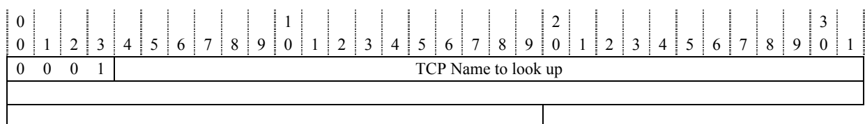
Figure 4/G.7714.1/Y.1705.1 – TCP-ID Name Message format
