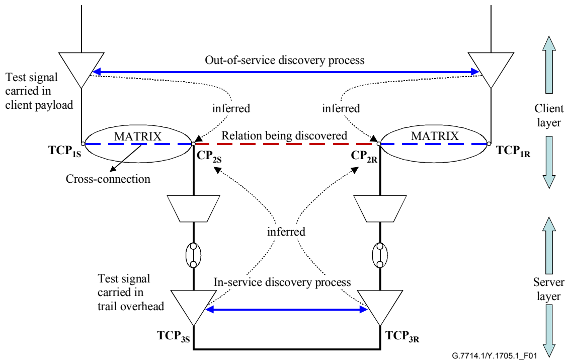
Figure 1/G.7714.1/Y.1705.1 – Entities in the in-service and out-of-service discovery processes
