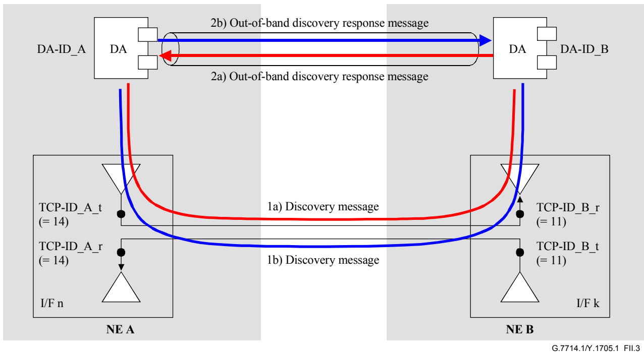
Figure II.3/G.7714.1/Y.1705.1 – Auto discovery in case of correctly wired interfaces
