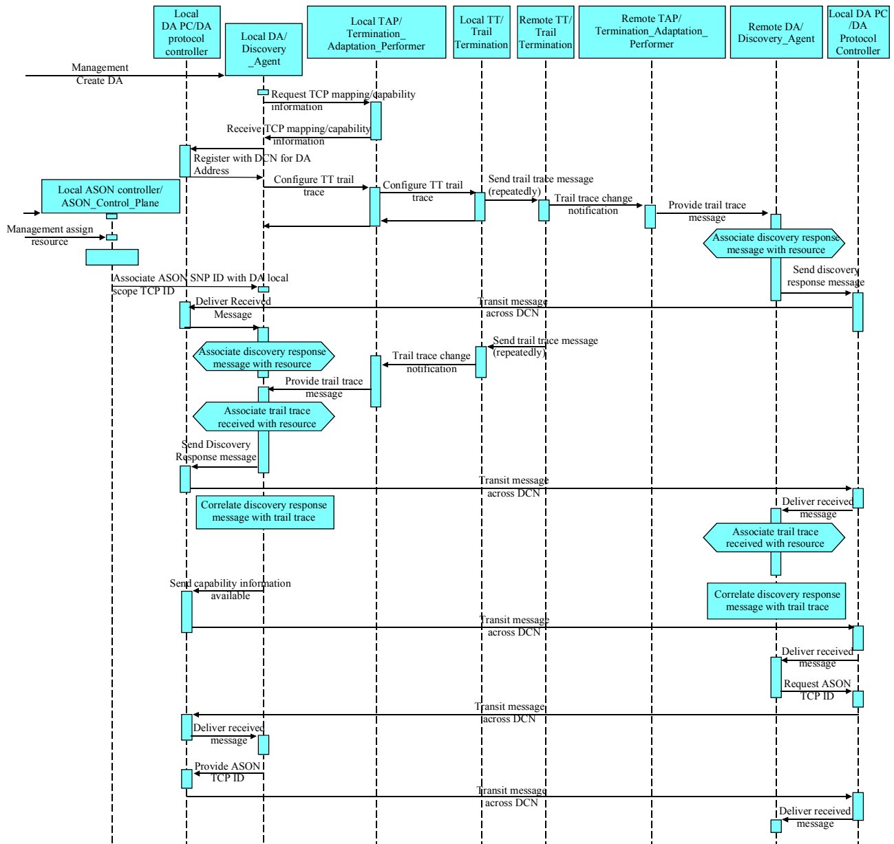
Figure I.1/G.7714.1/Y.1705.1 – Sequence diagram
