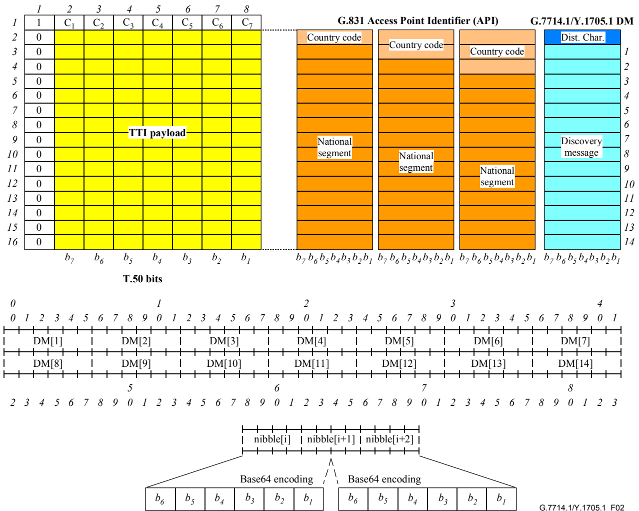
Figure 2/G.7714.1/Y.1705.1 – Auto Discovery Message (DM) format within the trail trace format
