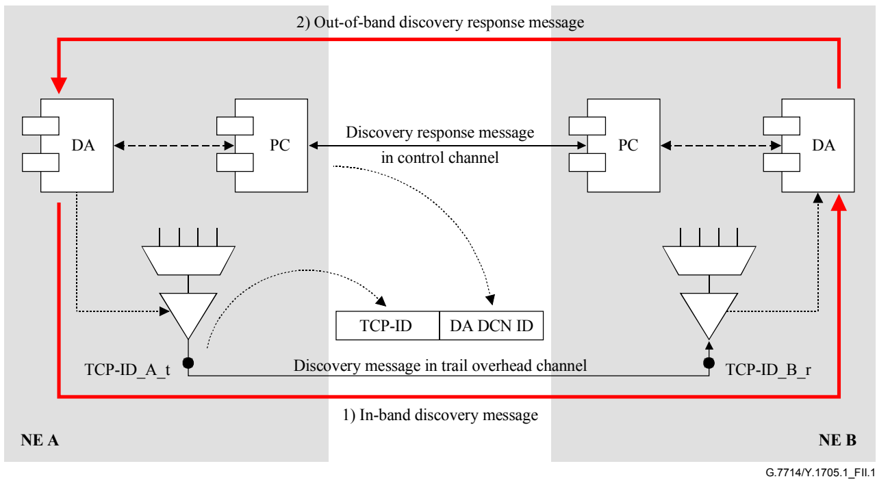
Figure II.1/G.7714.1/Y.1705.1 – Layer Adjacency Discovery procedure initiated by NE A
