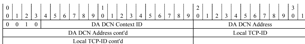
Figure 5/G.7714.1/Y.1705.1 – DA DCN Address Message format
