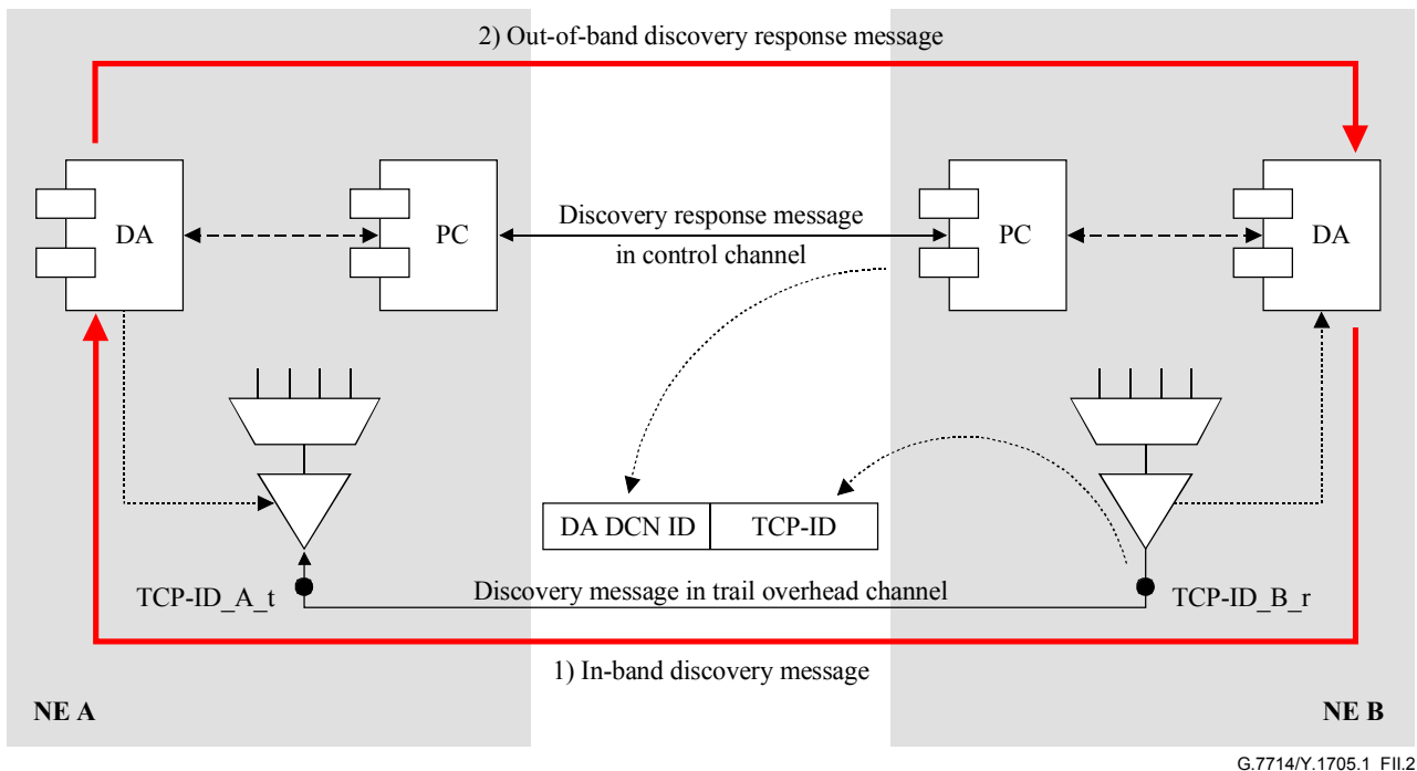
Figure II.2/G.7714.1/Y.1705.1 – Layer Adjacency Discovery procedure initiated by NE B
