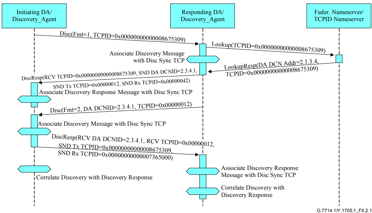
Figure II.2.1/G.7714.1/Y.1705.1 – Sequence for discovery between two DAs using different message formats
