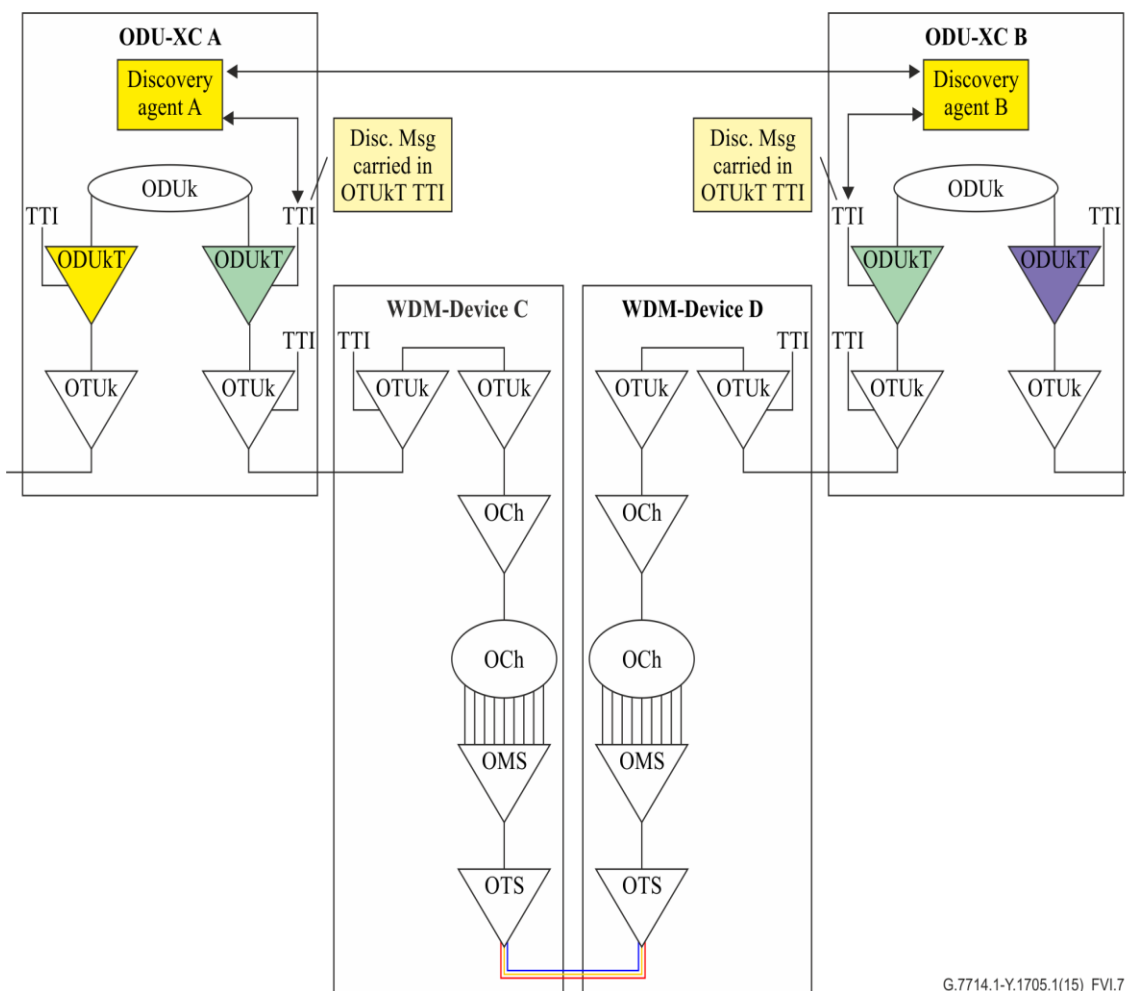
Figure VI.7 – Example of ODUkT TTI (SAPI sub-field)-based LAD for OTN with WDM equipment
