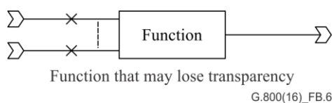
Figure B.6 – A system which loses information, for example by merging symbols from multiple input ports
