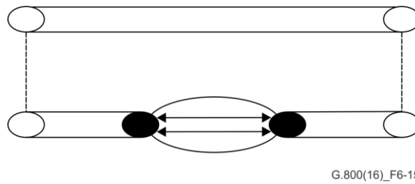
Figure 6-15 – Serial compound composed of component links and a subnetwork with configured subnetwork connections
