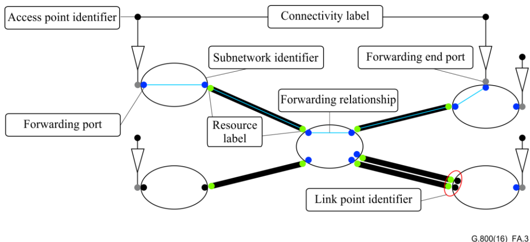
Figure A.3 – Identifiers in a layer network
