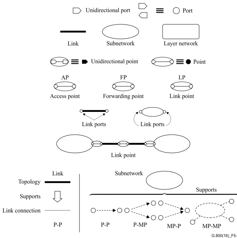
Figure 5-1 – Diagrammatic conventions
