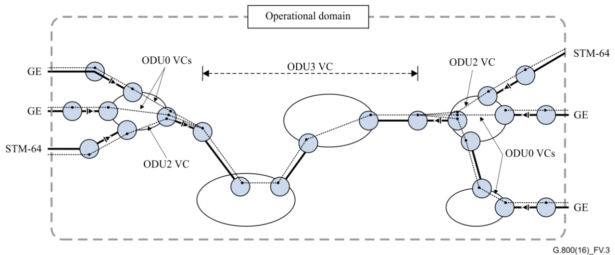
Figure V.3 – Example of virtual path (aggregation of service instances)
