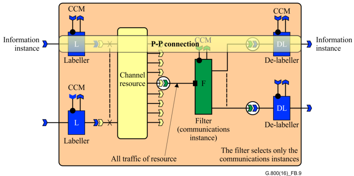
Figure B.9 – Demerger and the construction of a point to point connection
