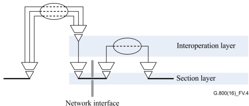
Figure V.4 – Network interface
