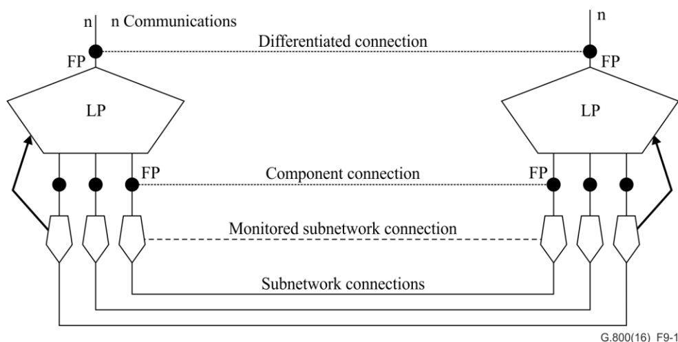
Figure 9-1 – Transport model for a differentiated connection
