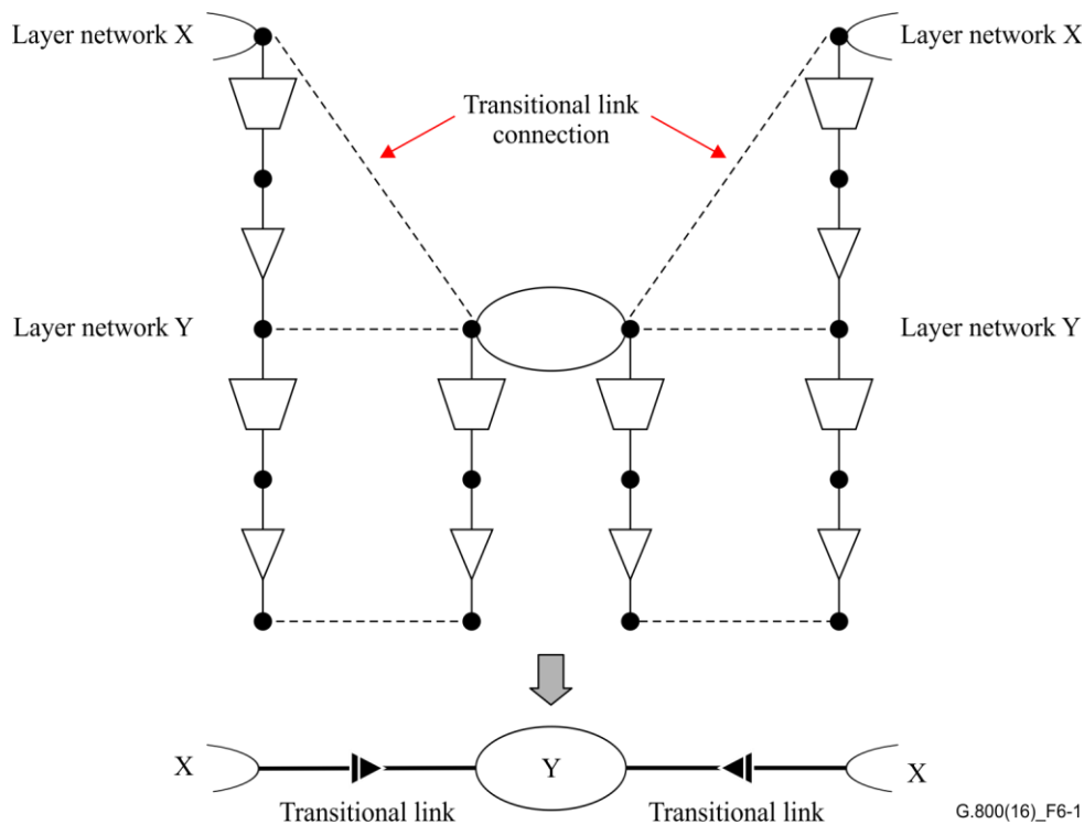
Figure 6-1 – Transitional link between layer networks X and Y
