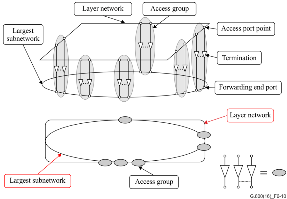
Figure 6-10 – Layer network
