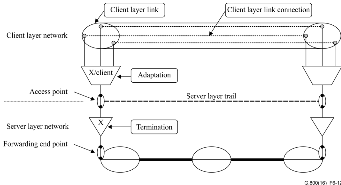
Figure 6-12 – Client-server relationship
