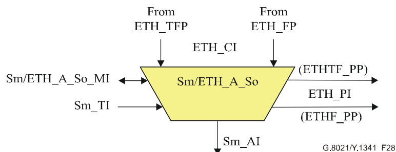
Figure 28/G.8021/Y.1341 – Sm/ETH_A_So symbol
