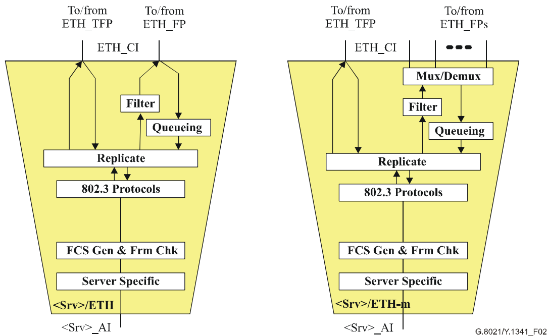
Figure 2/G.8021/Y.1341 – Server to ETH adaptation functions
