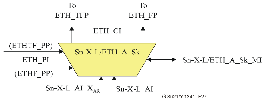
Figure 27/G.8021/Y.1341 – Sn-X-L/ETH_A_Sk symbol
