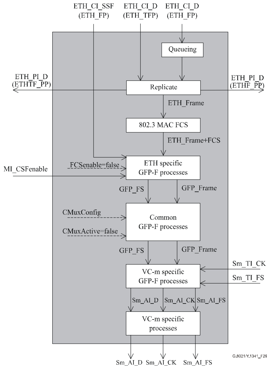
Figure 29/G.8021/Y.1341 – Sm/ETH_A_So process diagram
