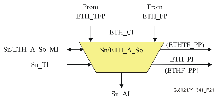
Figure 21/G.8021/Y.1341 – Sn/ETH_A_So symbol
