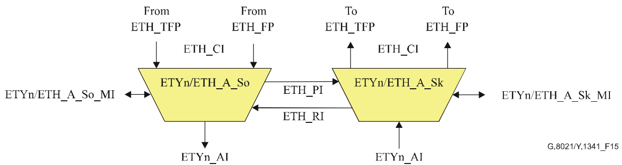
Figure 15/G.8021/Y.1341 – ETY n /ETH_A source and sink adaptation functions
