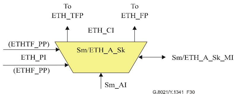
Figure 30/G.8021/Y.1341 – Sm/ETH_A_Sk symbol
