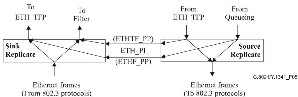
Figure 5/G.8021/Y.1341 – Replicate processes
