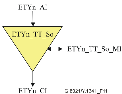
Figure 11/G.8021/Y.1341 – ETYn_TT_So symbol
