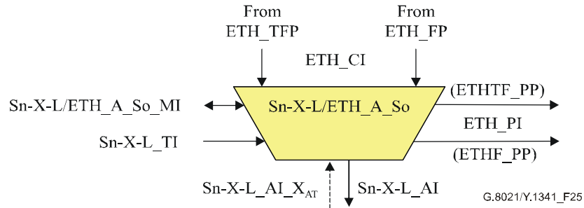
Figure 25/G.8021/Y.1341 – Sn-X-L/ETH_A_So symbol
