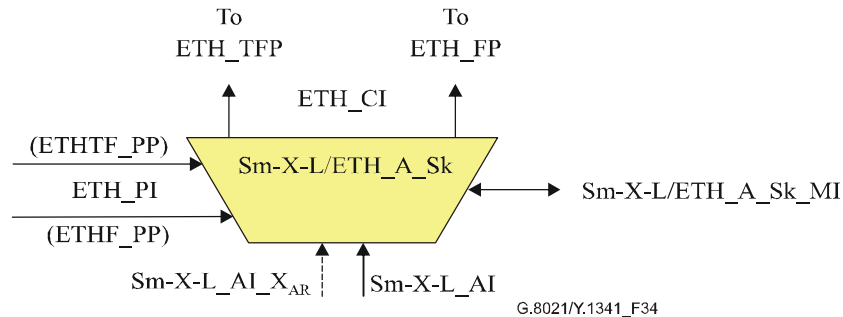
Figure 34/G.8021/Y.1341 – Sm-X-L/ETH_A_Sk symbol
