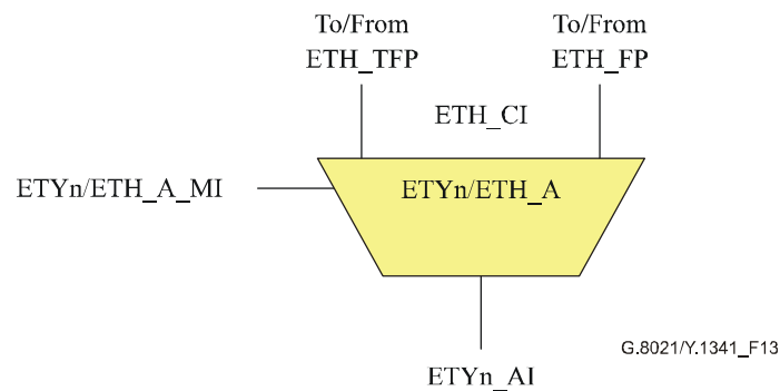
Figure 13/G.8021/Y.1341 – ETYn server to ETH adaptation function
