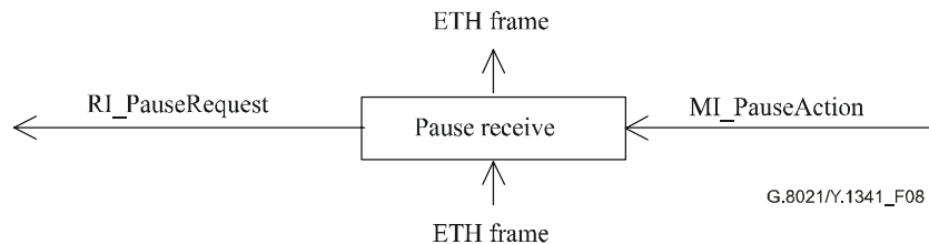
Figure 8/G.8021/Y.1341 – Receive pause process
