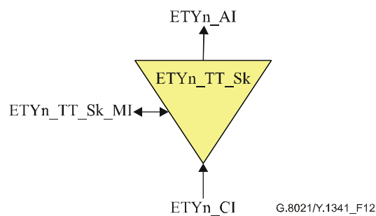
Figure 12/G.8021/Y.1341 – ETYn_TT_Sk symbol
