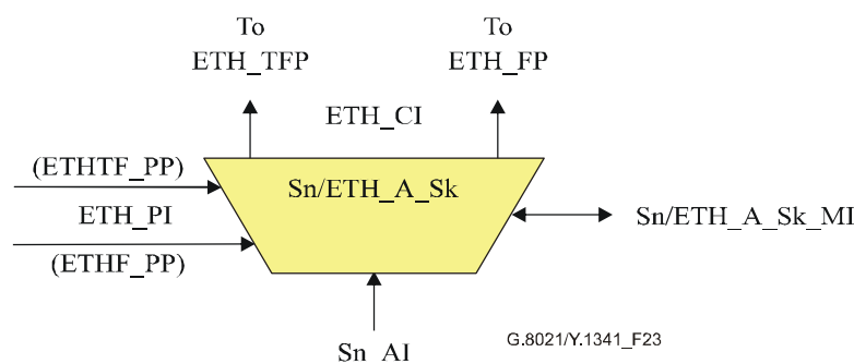
Figure 23/G.8021/Y.1341 – Sn/ETH_A_Sk symbol
