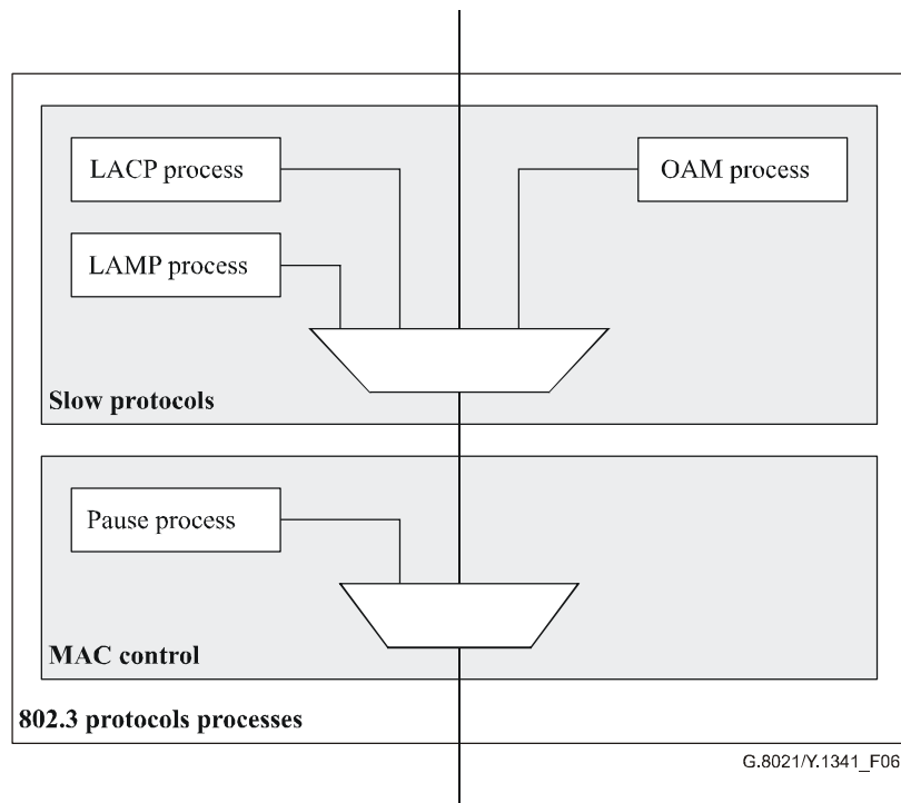
Figure 6/G.8021/Y.1341 – 802.3 protocols processes
