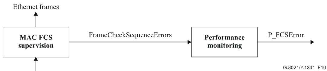
Figure 10/G.8021/Y.1341 – MAC frame check process
