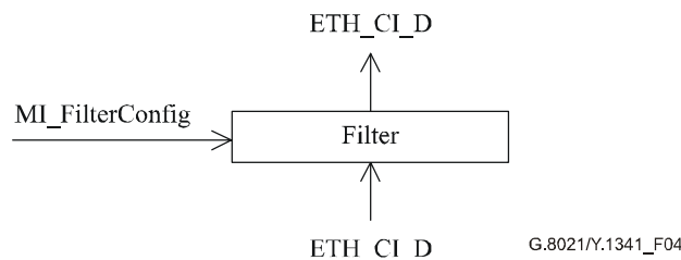
Figure 4/G.8021/Y.1341 – Filter process
