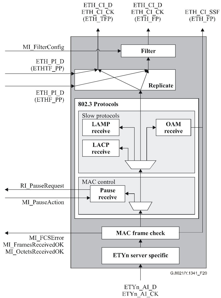
Figure 20/G.8021/Y.1341 – ETYn/ETH_A_Sk process diagram
