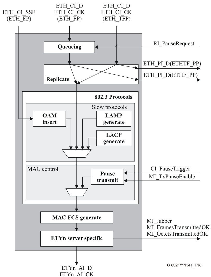
Figure 18/G.8021/Y.1341 – ETYn/ETH_A_So process diagram
