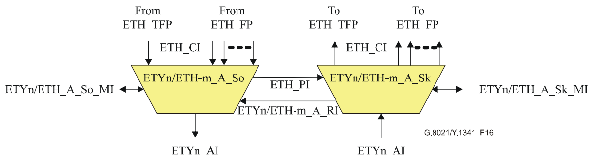
Figure 16/G.8021/Y.1341 – ETY n /ETH-m_A source and sink adaptation functions
