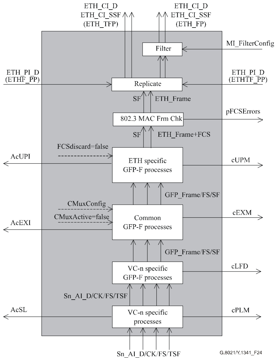
Figure 24/G.8021/Y.1341 – Sn/ETH_A_Sk process diagram
