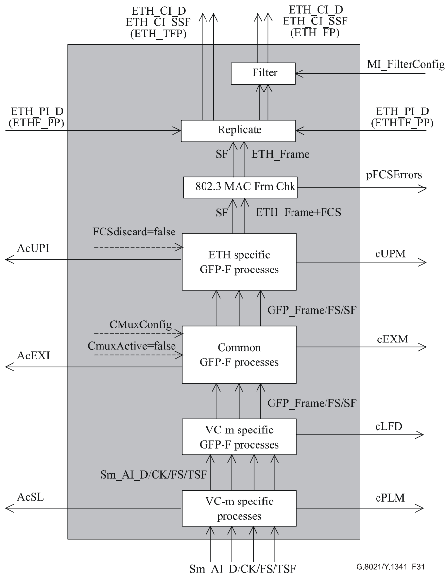
Figure 31/G.8021/Y.1341 – Sm/ETH_A_Sk process diagram
