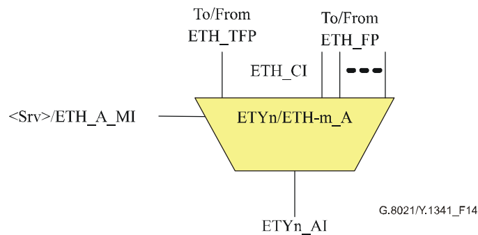
Figure 14/G.8021/Y.1341 – ETYn/ETH adaptation function (Multiple Flow Point)
