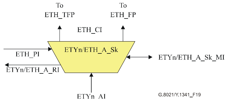
Figure 19/G.8021/Y.1341 – ETYn/ETH_A_Sk symbol
