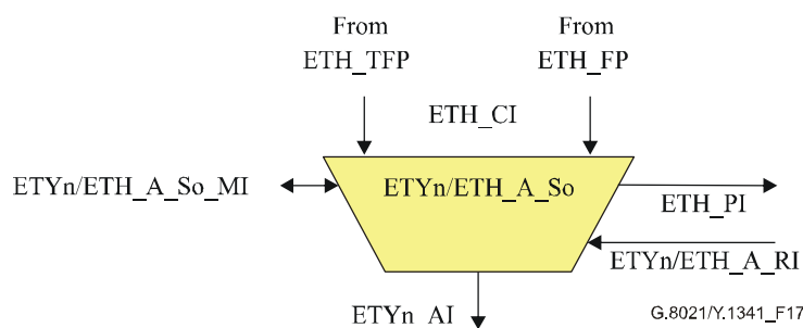
Figure 17/G.8021/Y.1341 – ETY n /ETH_A_So symbol
