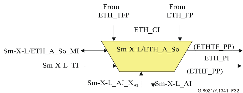
Figure 32/G.8021/Y.1341 – Sm-X-L/ETH_A_So symbol
