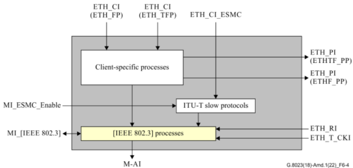
Figure 6-4 – M-AI/ETH_A_So process
