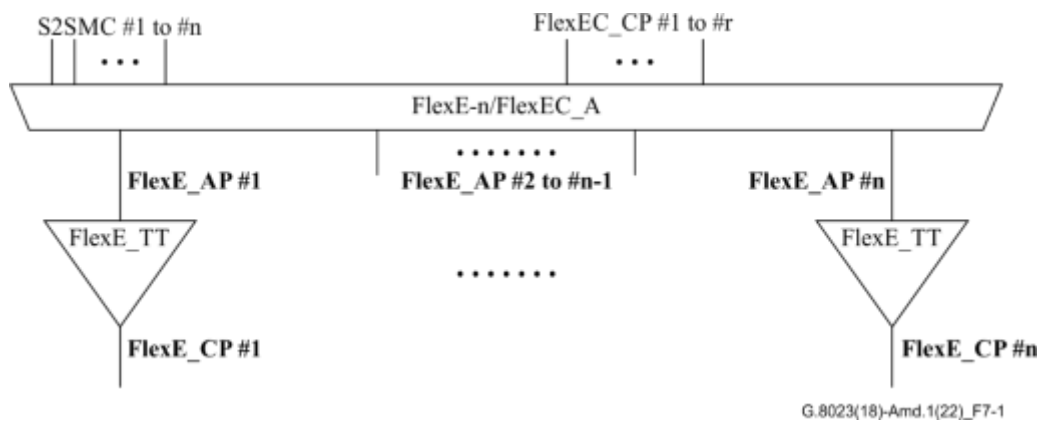
Figure 7-1 – FlexE functions
