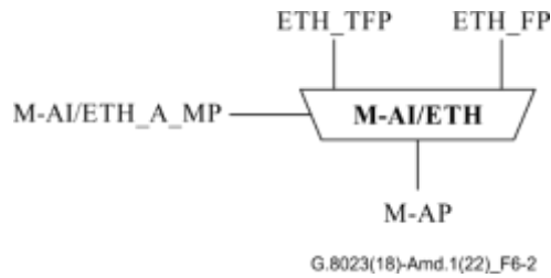
Figure 6-2 – M-AI to ETH adaptation function
