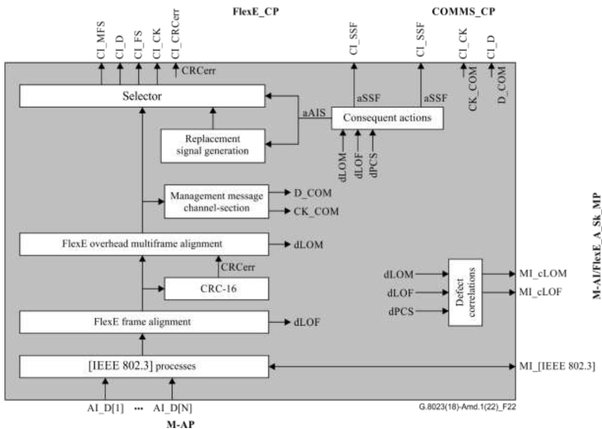
Figure 6-22 – M-AI/FlexE_A_Sk processes
