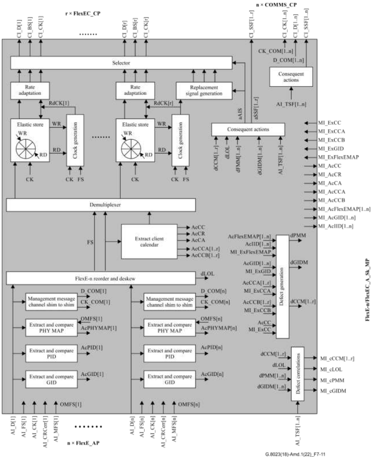
Figure 7-11 – FlexE-n/FlexEC_A_Sk processes
