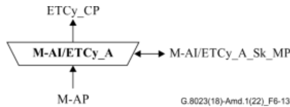
Figure 6-13 – M-AI/ETCy_A_Sk function
