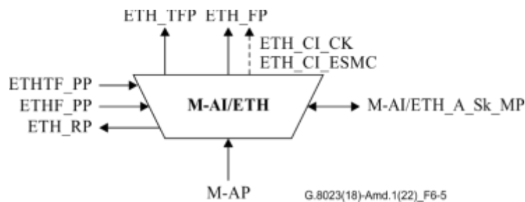
Figure 6-5 – M-AI/ETH_A_Sk symbol
