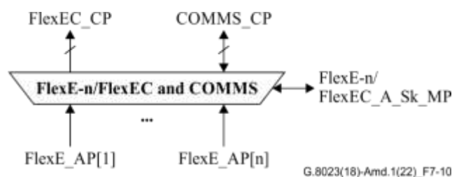
Figure 7-10 – FlexE-n/FlexEC_A_Sk function
