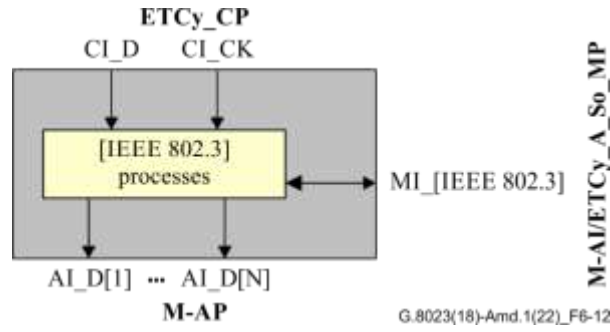
Figure 6-12 – M-AI/ETCy_A_So processes
