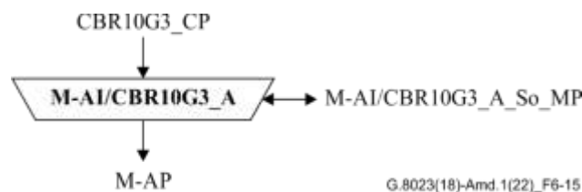
Figure 6-15 – M-AI/CBR10G3_A_So function
