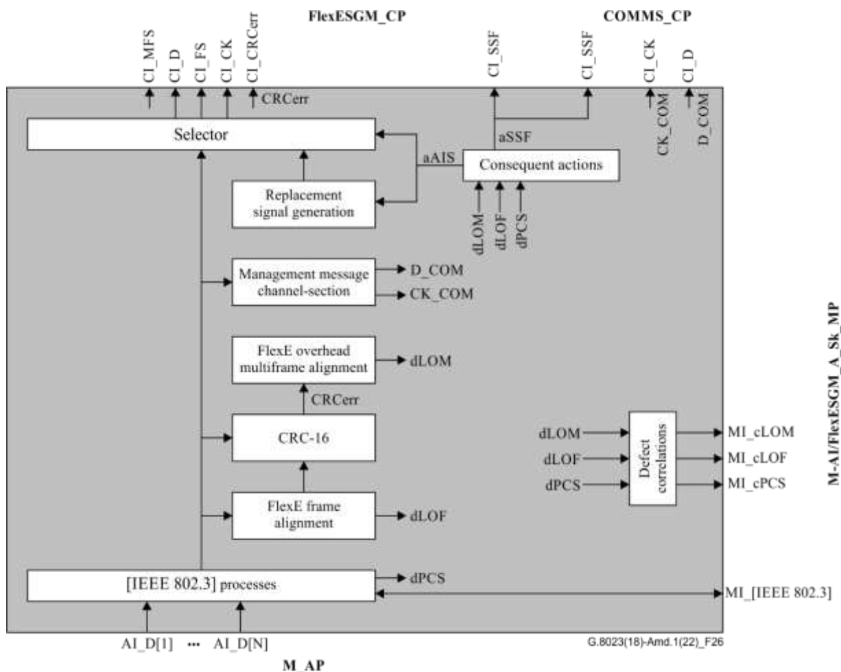
Figure 6-26 – M-AI/FlexESGM_A_Sk processes
