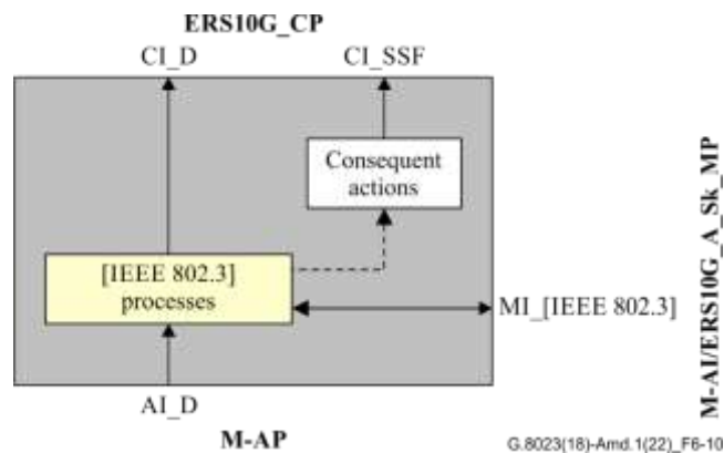
Figure 6-10 – M-AI/ERS10G_A_Sk processes
