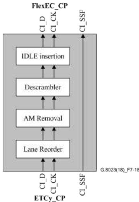
Figure 7-18 – ETCy>FlexEC processes (y = 40GR, 50GR, 100GR)
