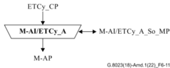
Figure 6-11 – M-AI/ETCy_A_So function
