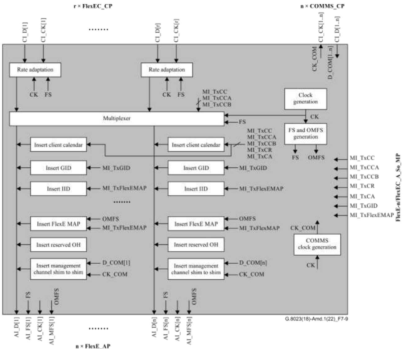
Figure 7-9 – FlexE-n/FlexEC_A_So processes
