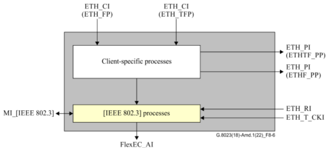
Figure 8-6 – FlexEC/ETH_A_So processes
