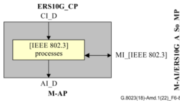
Figure 6-8 – M-AI/ERS10G_A_So processes
