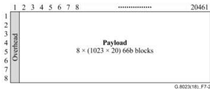
Figure 7-2 – FlexE frame
