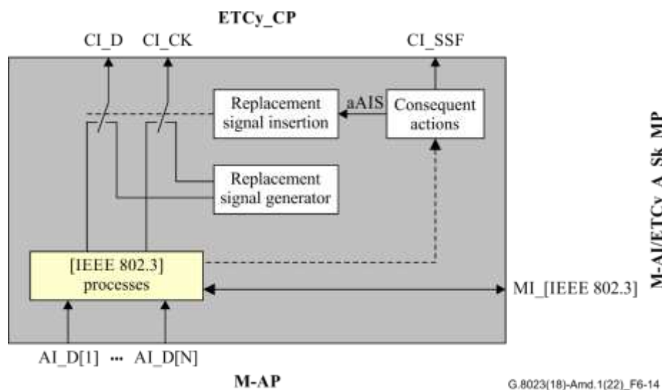
Figure 6-14 – M-AI/ETCy_A_Sk processes
