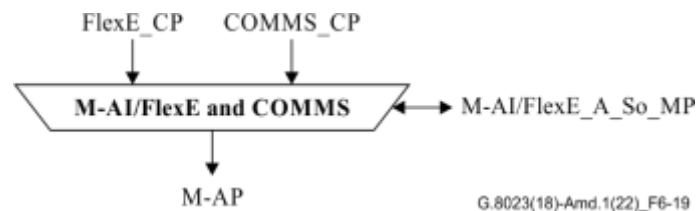
Figure 6-19 – M-AI/FlexE_A_So function
