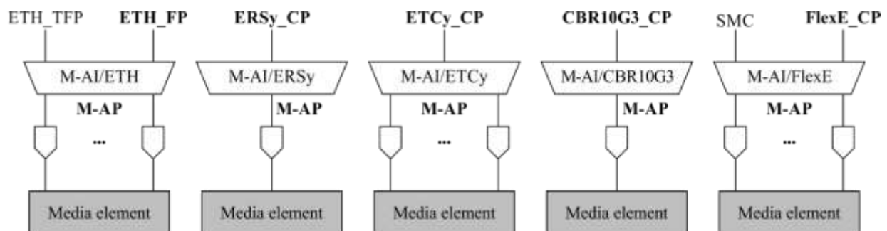
Figure 6-1 – M-AI to client adaptation functions
