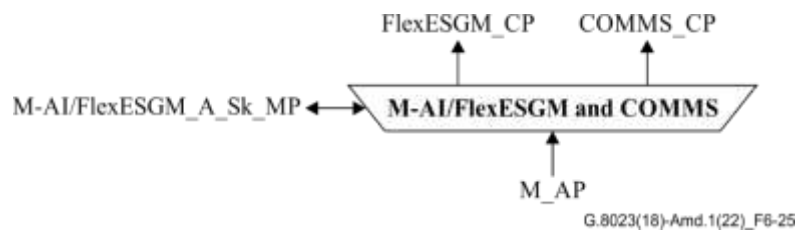
Figure 6-25 – M-AI/FlexESGM_A_Sk function
