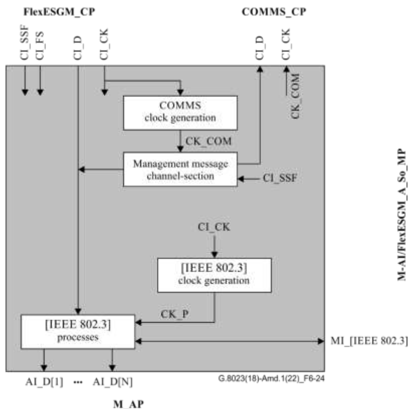
Figure 6-24 – M-AI/FlexESG_A_So processes
