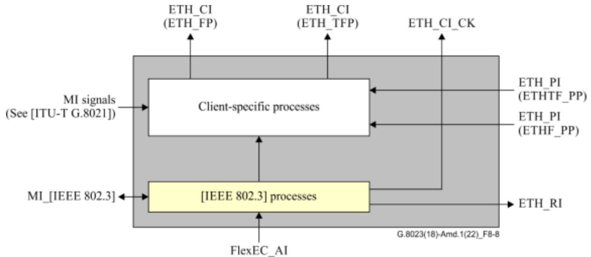
Figure 8-8 – FlexEC/ETH_A_Sk processes
