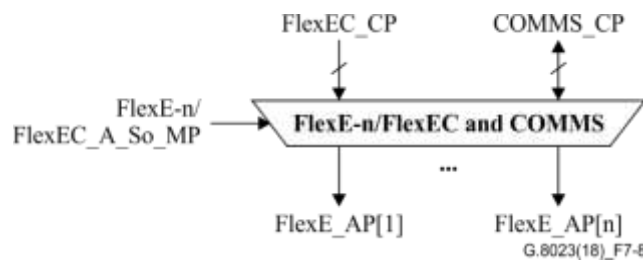
Figure 7-8 – FlexE-n/FlexEC_A_So function
