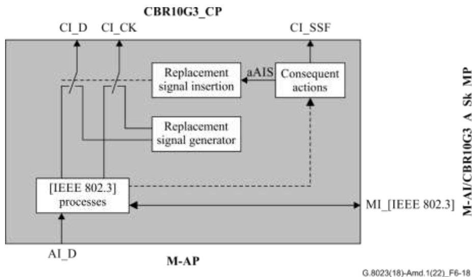
Figure 6-18 – M-AI/CBR10G3_A_Sk processes
