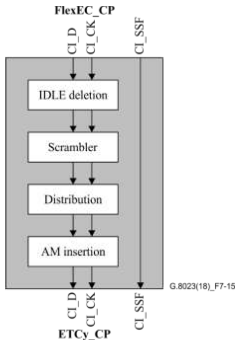
Figure 7-15 – FlexEC>ETCy processes (y = 40GR, 50GR, 100GR)
