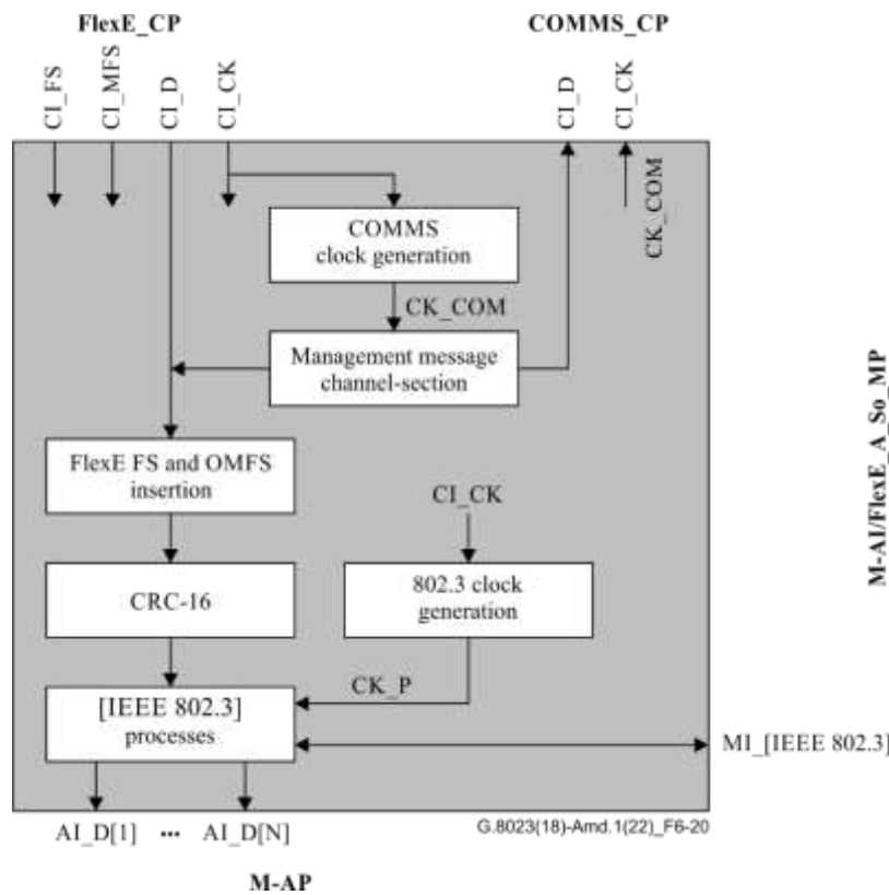
Figure 6-20 – M-AI/FlexE_A_So processes
