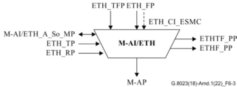
Figure 6-3 – M-AI/ETH_A_So symbol
