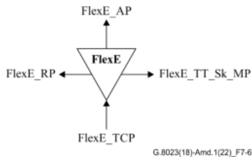
Figure 7-6 – FlexE_TT_Sk function
