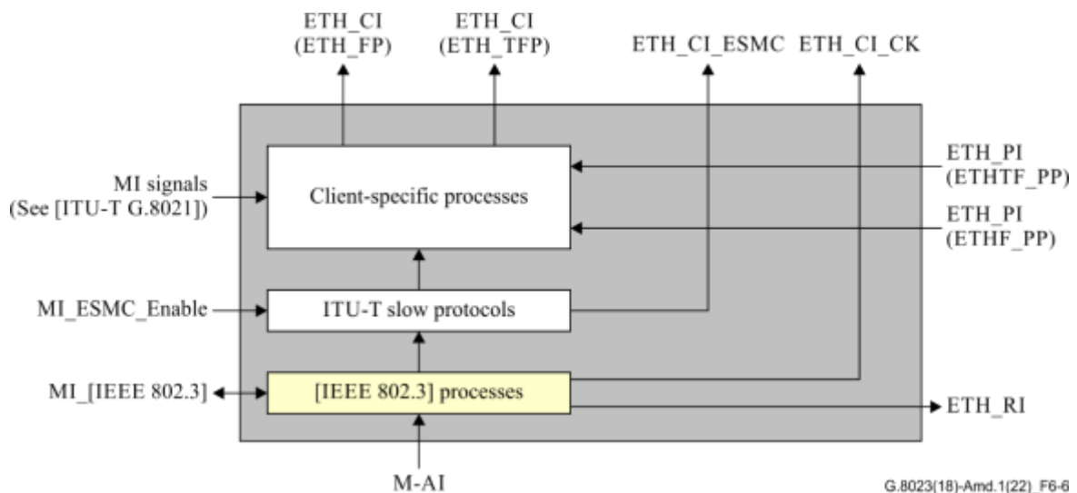
Figure 6-6 – M-AI/ETH_A_Sk process
