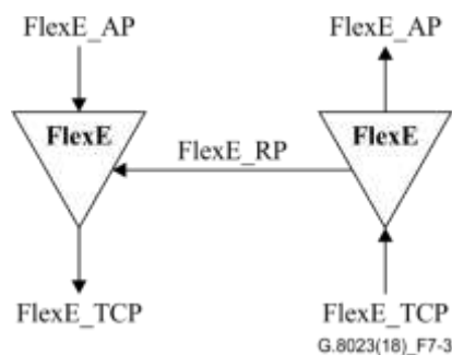
Figure 7-3 – FlexE_TT
