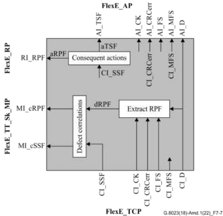
Figure 7-7 – FlexE_TT_Sk processes
