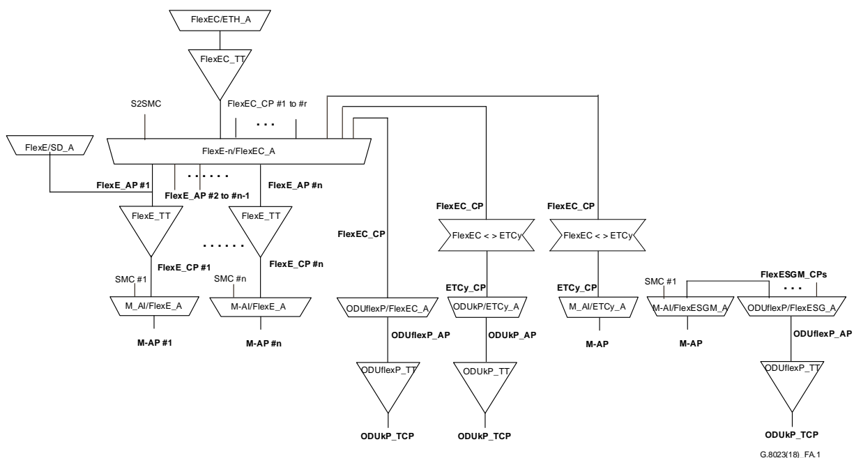
Figure A.1 – Overview of FlexE-related atomic functions
