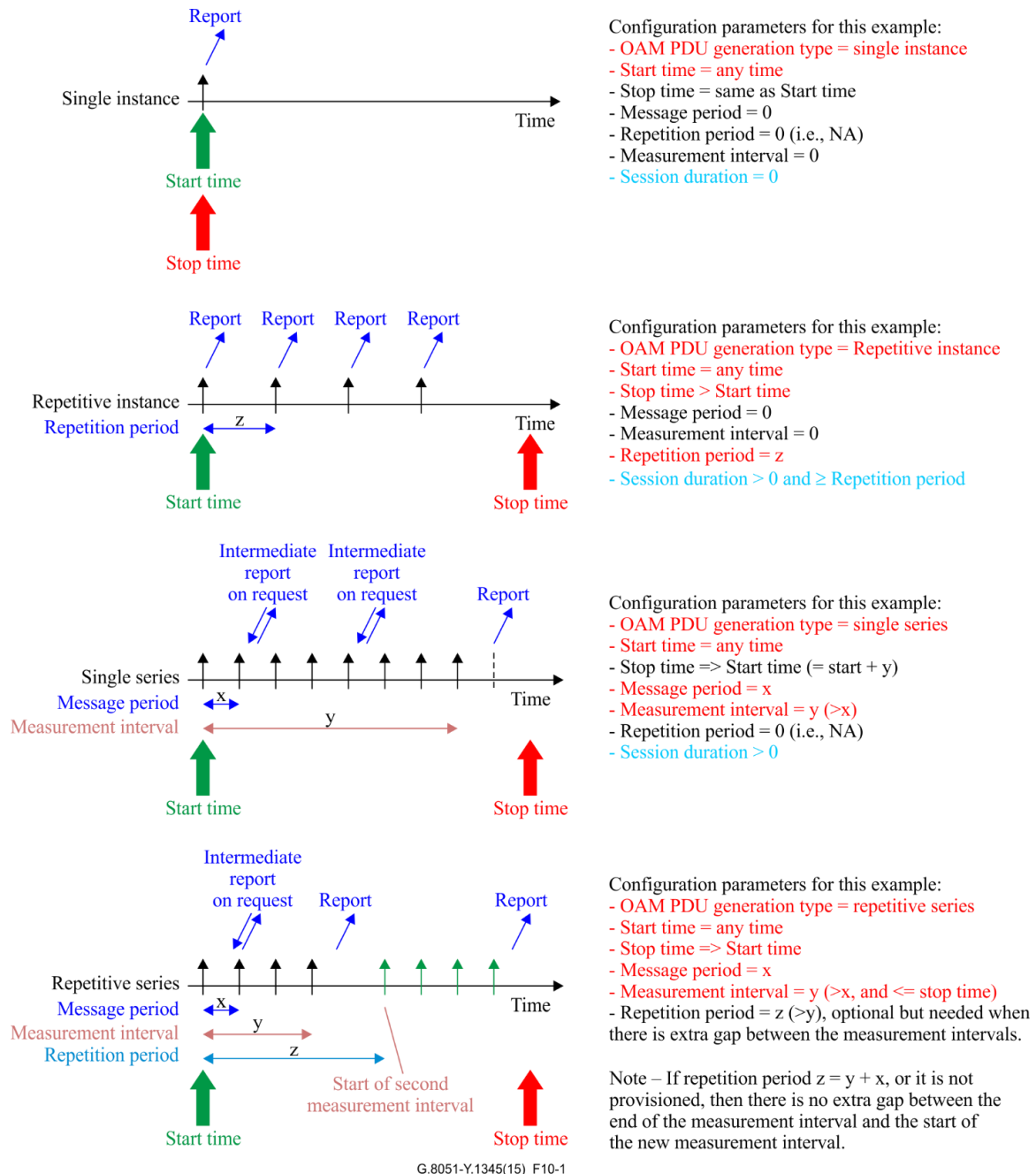
Figure 10-1 – On-demand OAM PDU generation mechanisms
