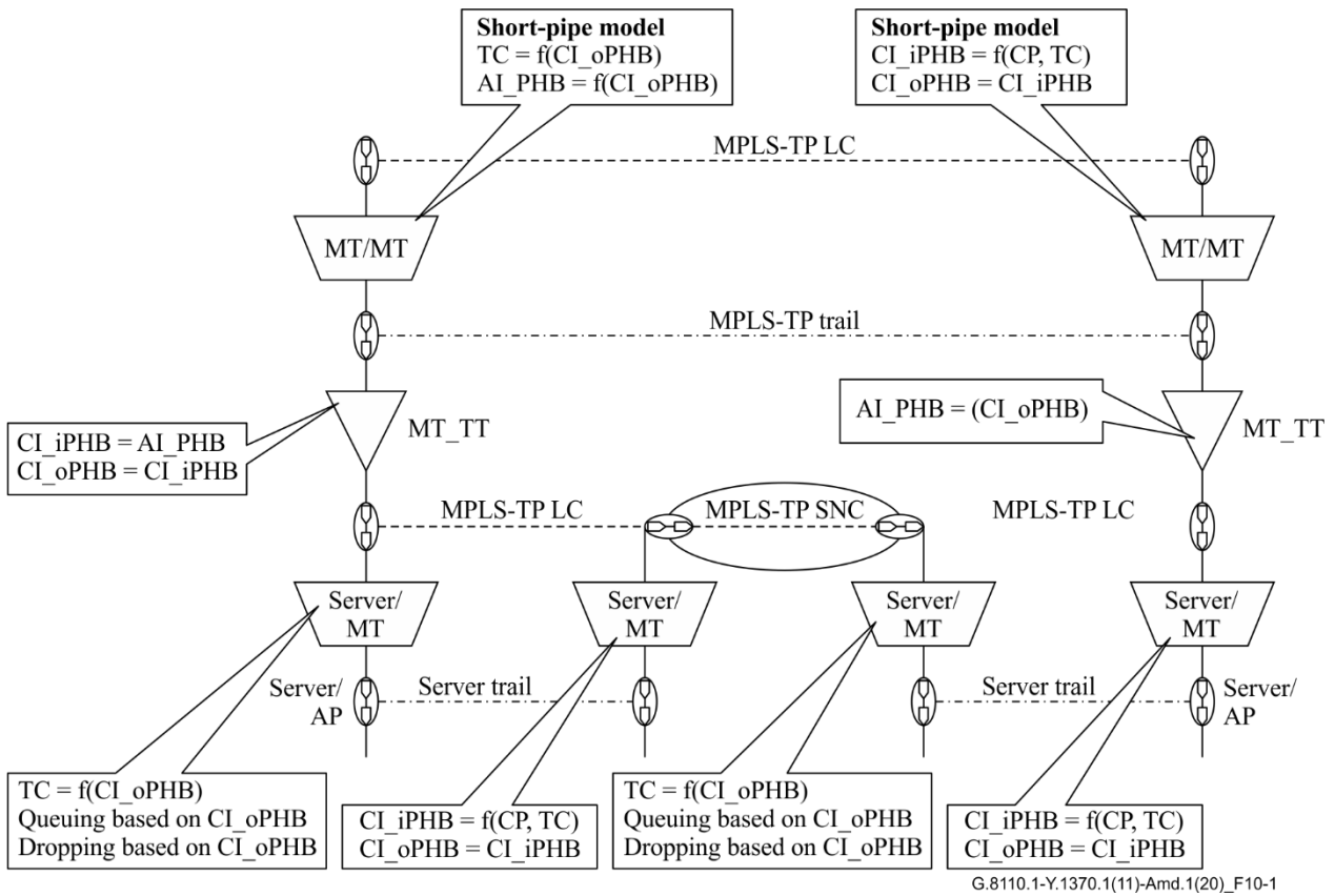
Figure 10-1 – Reference diagram for the short-pipe model
