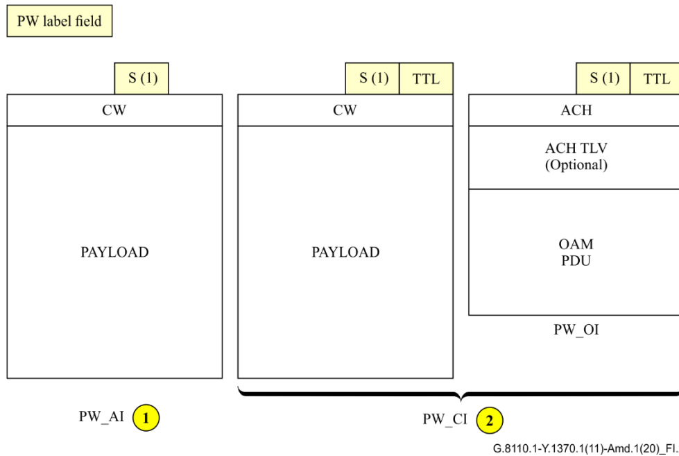
Figure I.2 – MPLS-TP network adapted and characteristic information traffic units (reference points 1 and 2)
