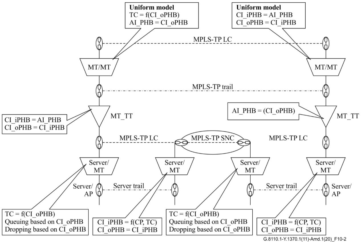
Figure 10-2 – Reference diagram for the uniform model
