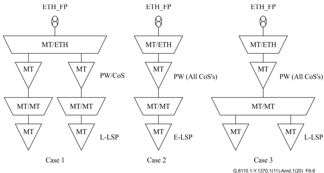
Figure 6-6 – Examples of QoS processing in MT/Client_A function
