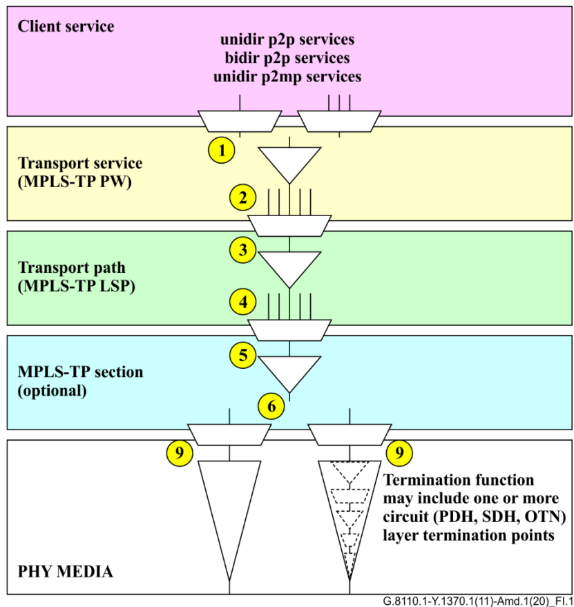
Figure I.1 – MPLS-TP network architecture (layer view) example
