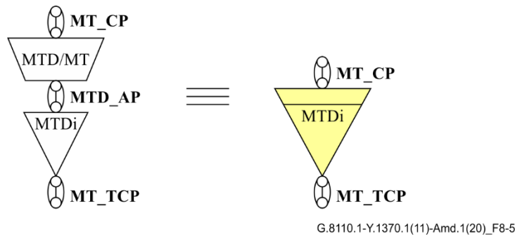
Figure 8-5 – MPLS-TP half MIP compound function
