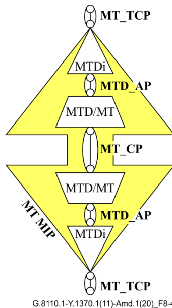
Figure 8-4 – MPLS-TP MIP compound function
