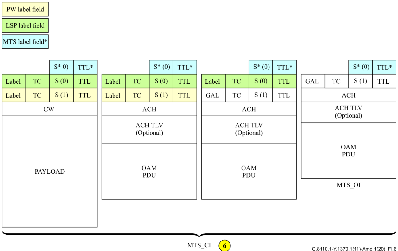
Figure I.6 – MPLS-TP network adapted and characteristic information traffic units (reference point 6)
