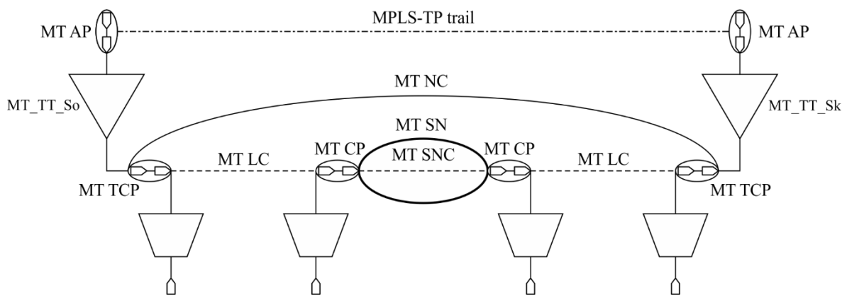
Figure 6-4 – MPLS-TP layer network example
