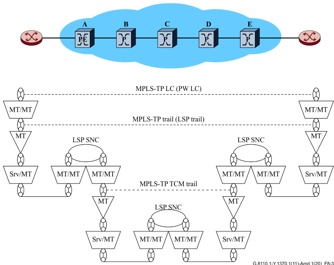
Figure 8-3 – MPLS-TP TCM example
