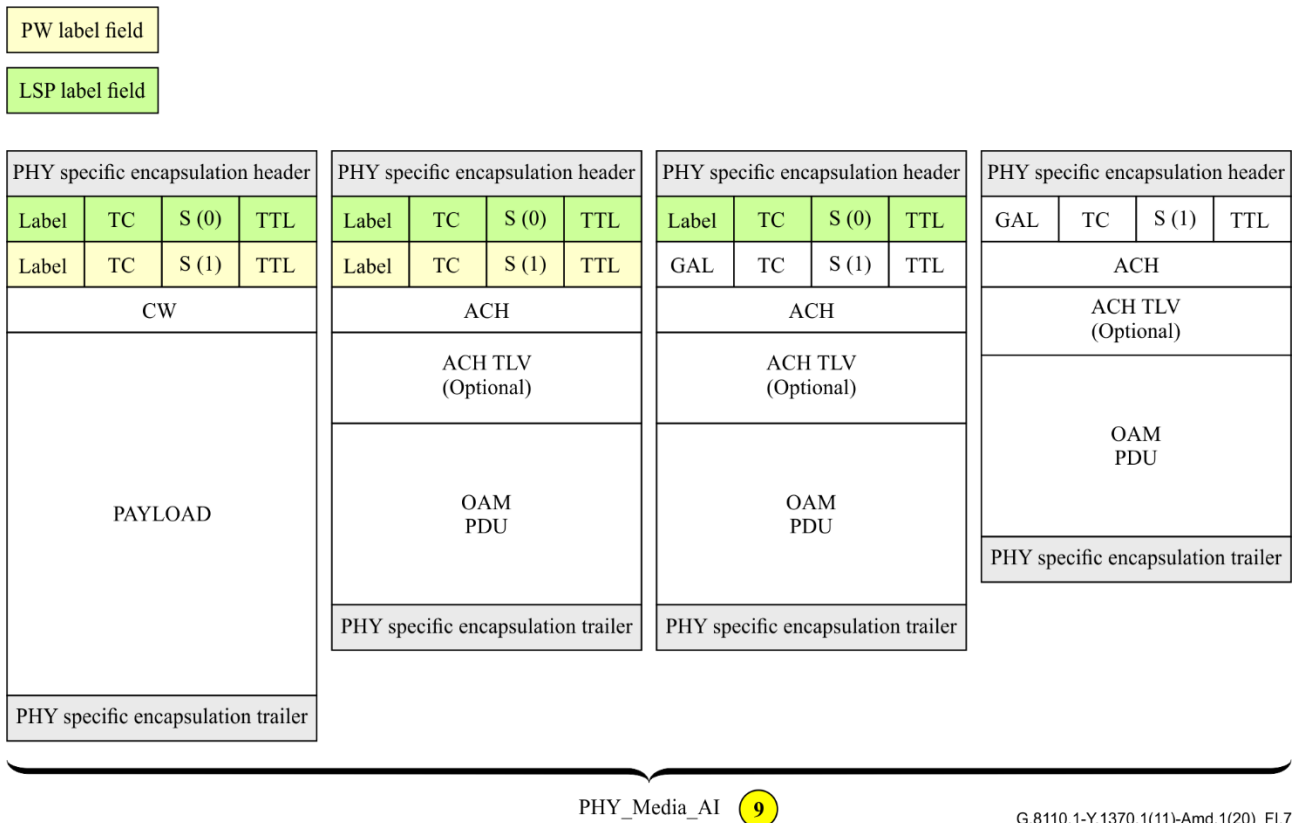
Figure I.7 – MPLS-TP network adapted and characteristic information traffic units (reference point 9)
