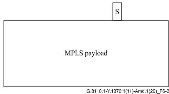
Figure 6-2 – MT_AI traffic unit
