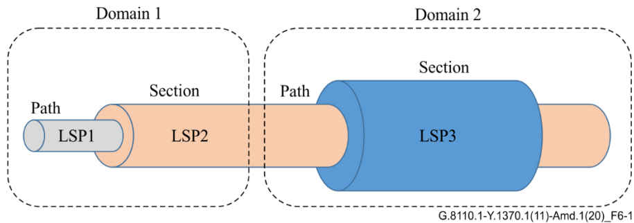
Figure 6-1 – MPLS-TP roles and layers
