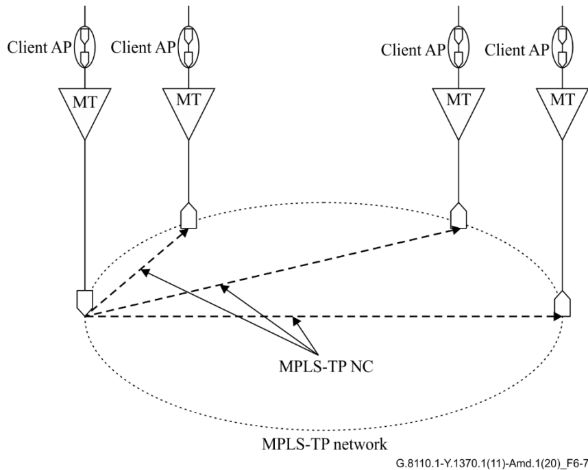
Figure 6-7 – Point-to-multipoint MPLS-TP connection
