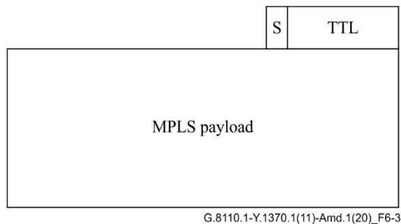
Figure 6-3 – MT_CI traffic unit
