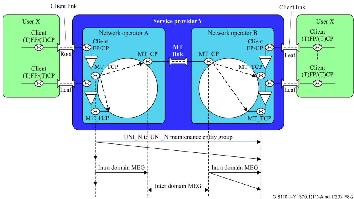
Figure 8-2 – Point-to-multipoint MPLS-TP connection administrative domain associated maintenance entity groups
