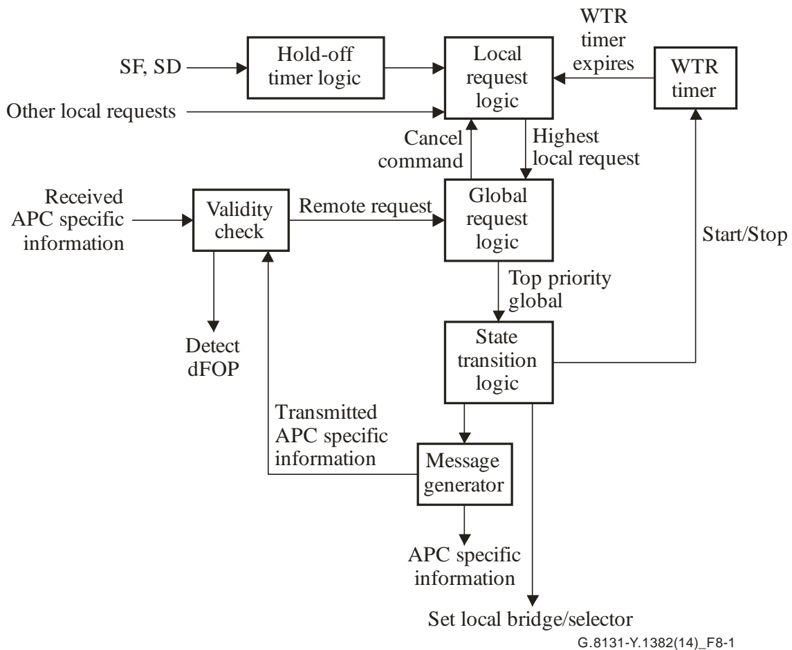
Figure 8-1 – Principle of MPLS-TP linear protection switching algorithm
