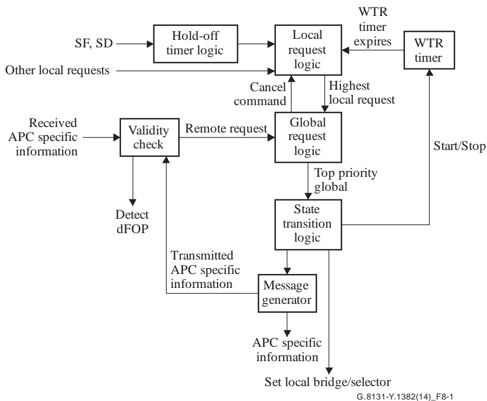
Figure 8-1 – Principle of MPLS-TP linear protection switching algorithm
