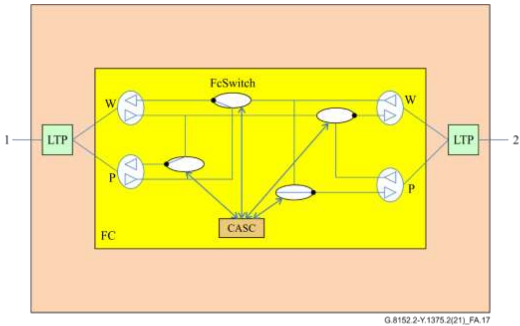
Figure A.17 – Wrapping: Node B with failure on link between node B and node C
