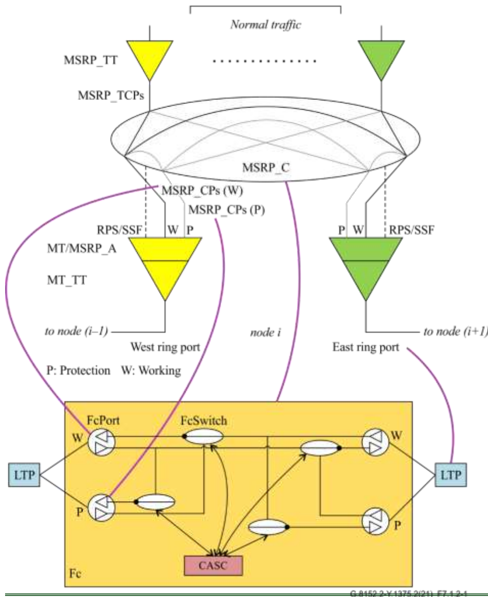
Figure 7-4 Mapping between MSRP functions and information model artefacts
