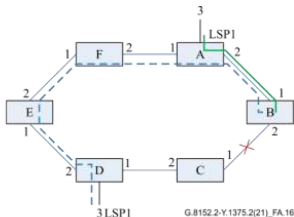
Figure A.16 – Short-wrapping for link failure
