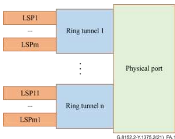
Figure A.1 – The logic layers of the ring
