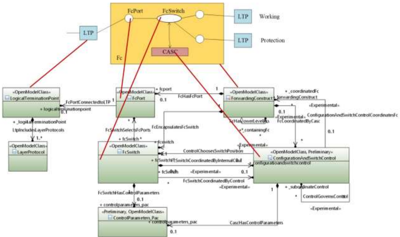
Figure 7-2 – Simplified resilience model for MPLS-TP linear protection
