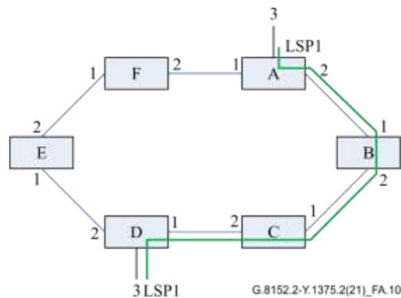
Figure A.10 – Basic network
