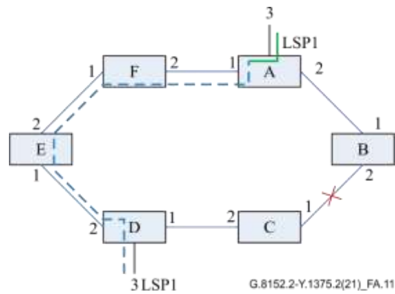
Figure A.11 – Steering for link failure
