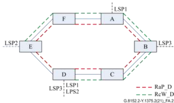
Figure A.2 – Ring tunnels in MSRP
