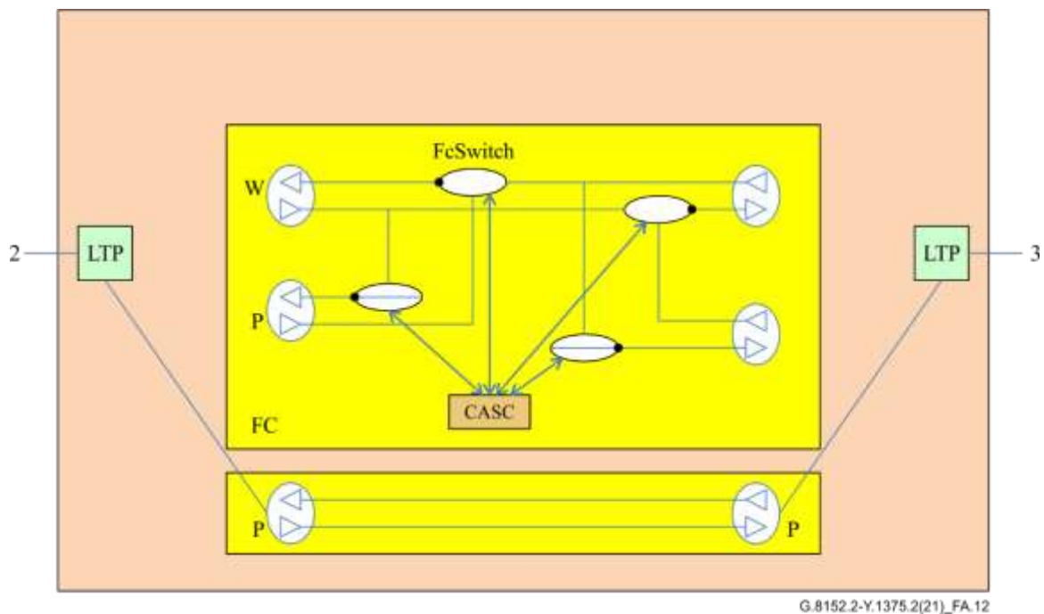
Figure A.12 – Steering: Node D with failure on link between node B and node C
