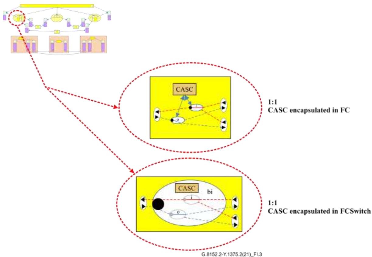
Figure I.3 – Detail of a nodal view of 1:1 switches
