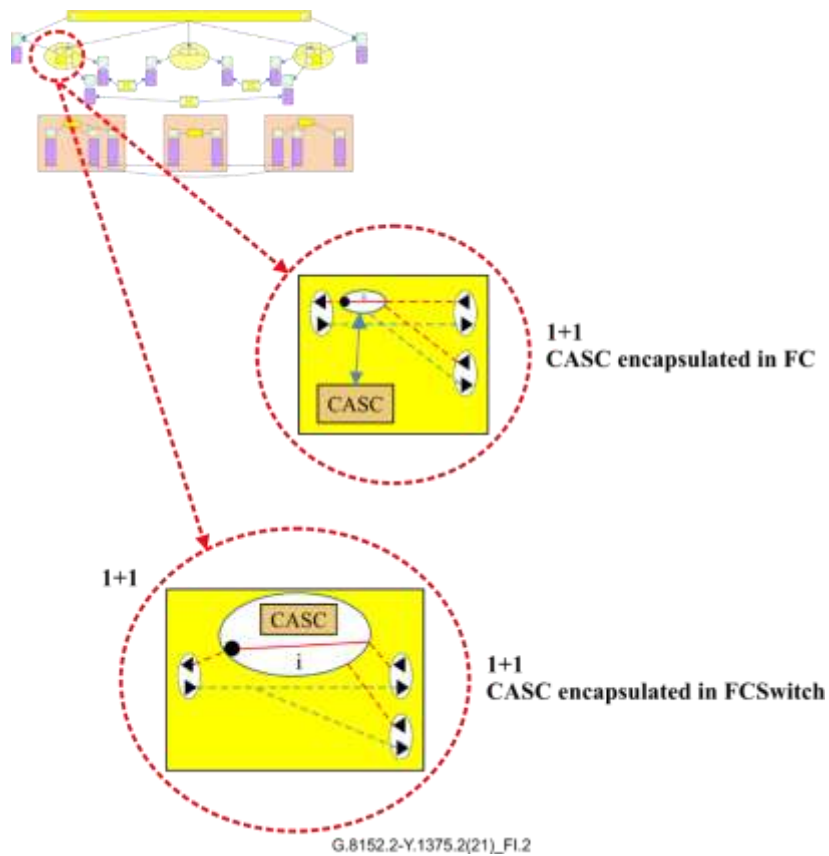
Figure I.2 – Detail of a nodal view of 1+1 switches
