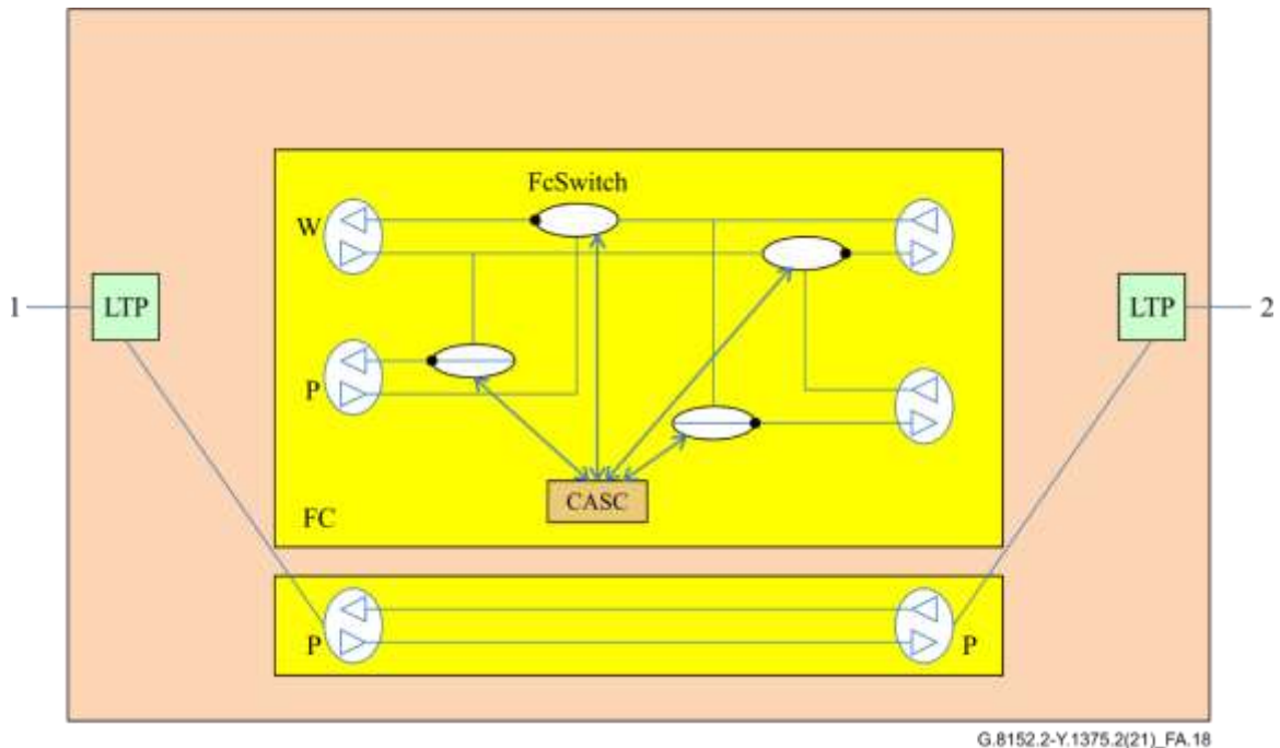
Figure A.18 – Short-wrapping: Node E and node F with failure on link between node B and node C
