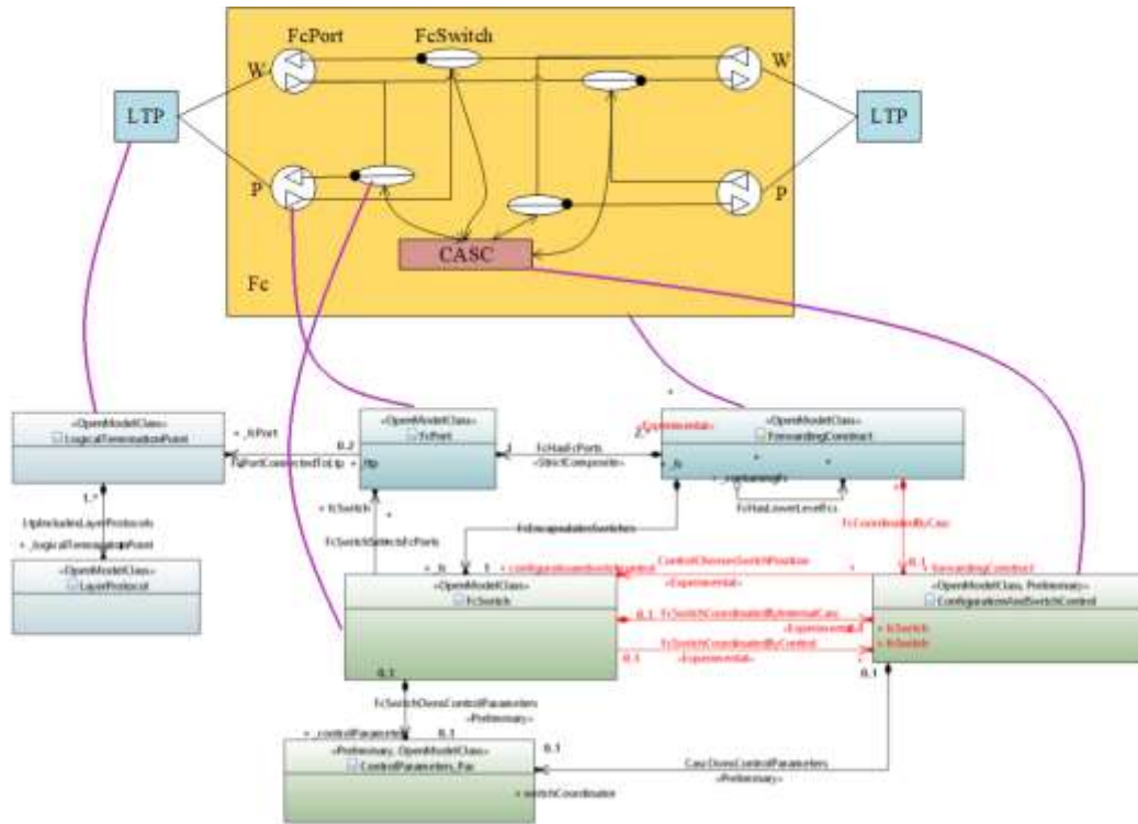
Figure 7-5 Simplified resilience model for MSRP
