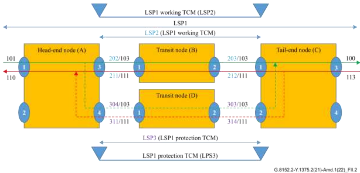
Figure II.2 – Example reference network for MPLS-TP SNC/S
