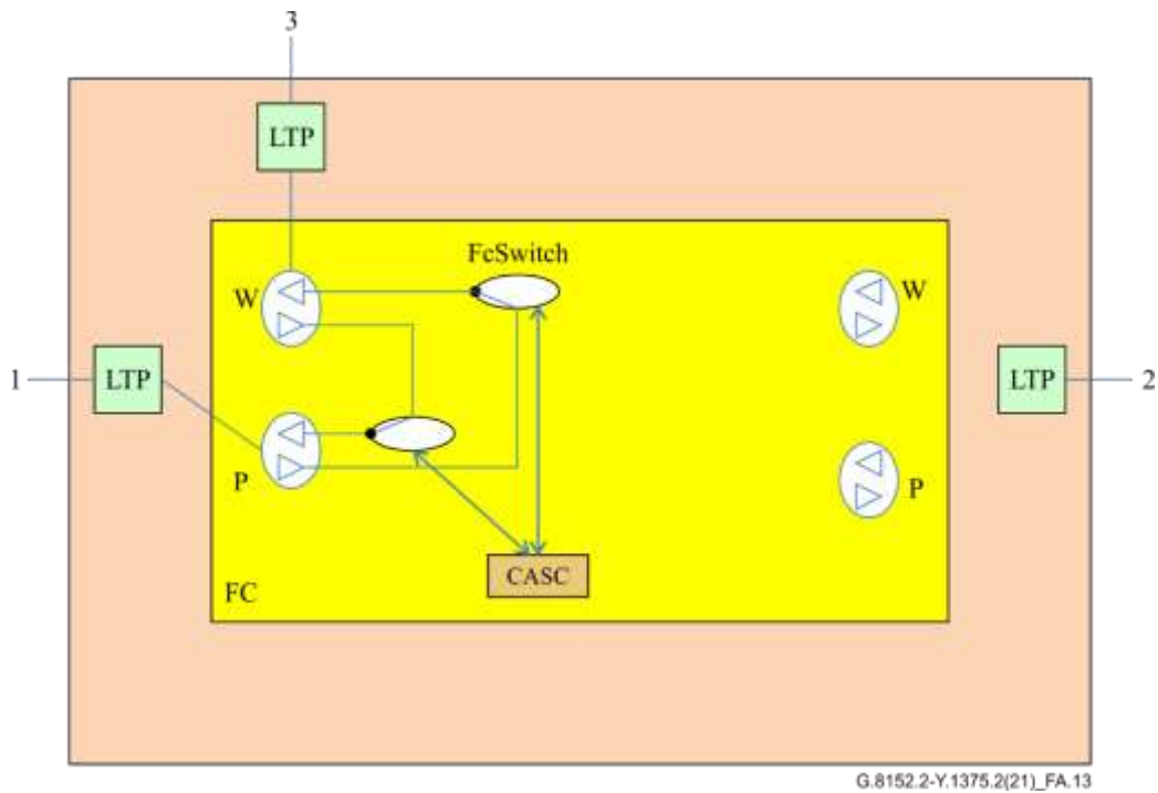
Figure A.13 – Steering: Node A with failure on link between node B and node C
