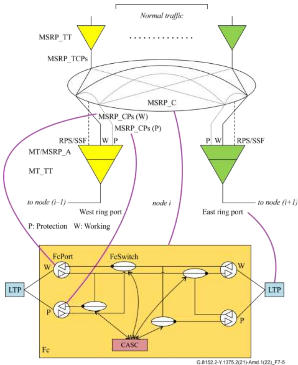
Figure 7-5 – Mapping between MSRP functions and information model artefacts
