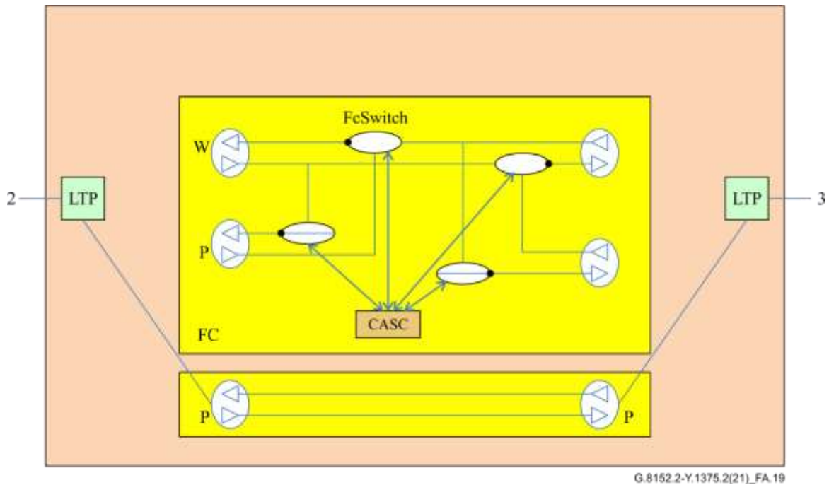
Figure A.19 – Short-wrapping: Node D with failure on the link between node B and node C
