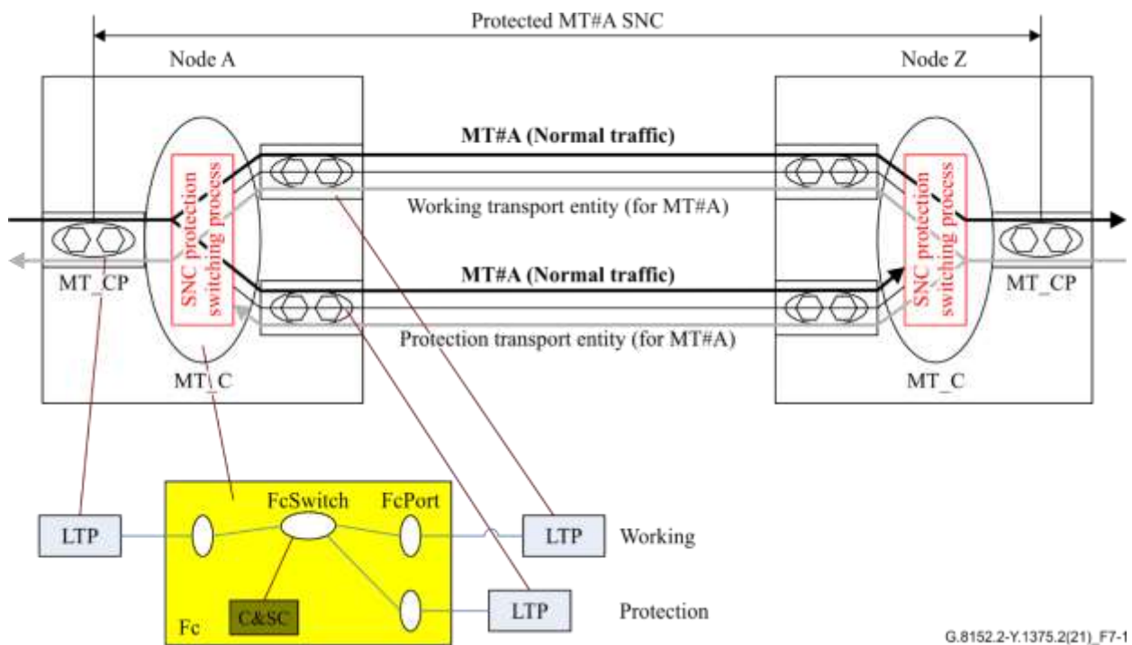
Figure 7-1 – Mapping between [ITU-T G.8131] and [ITU-T G.7711] for MPLS-TP linear protection model
