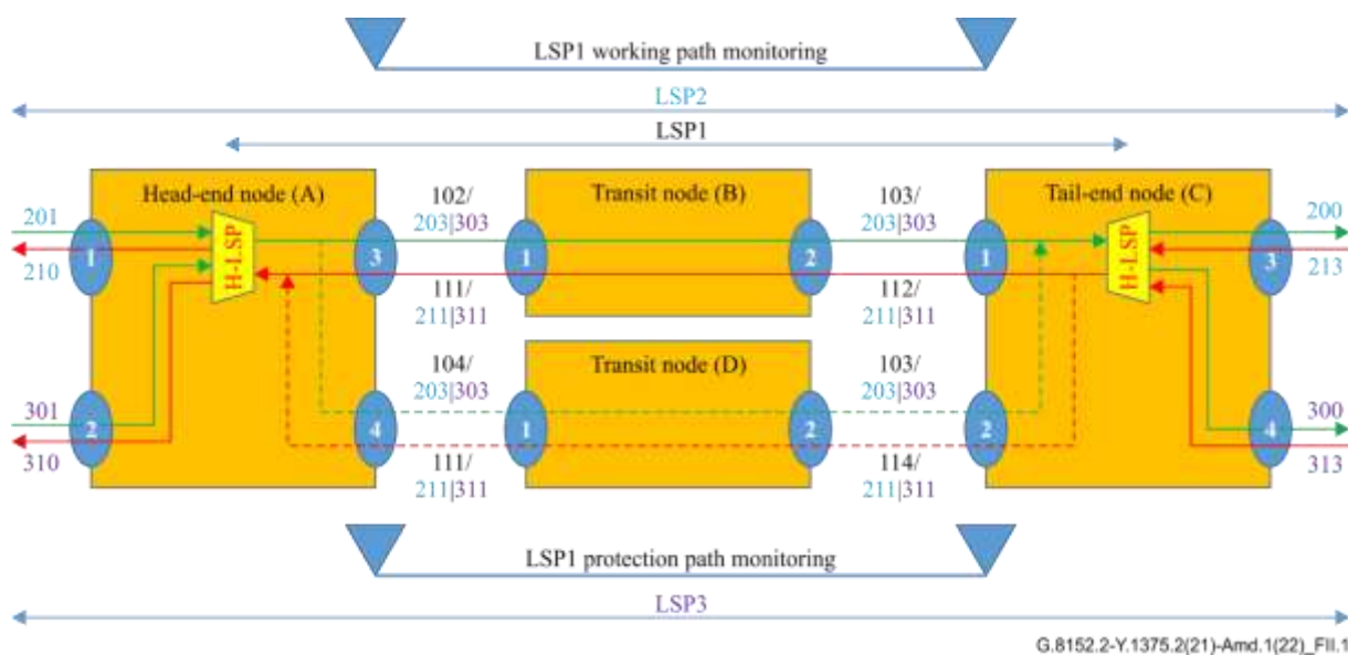
Figure II.1 – Example reference network for MPLS-TP trail protection
