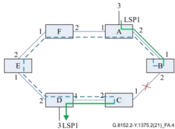
Figure A.4 – Wrapping for link failure
