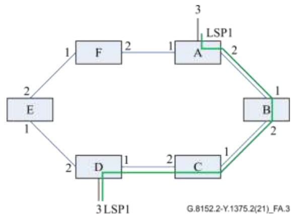
Figure A.3 – Basic network
