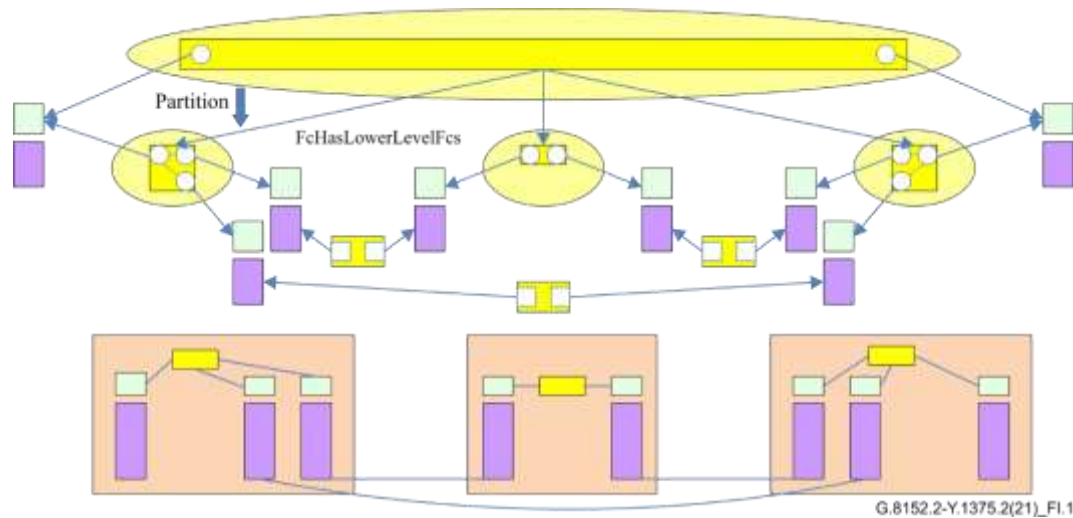
Figure I.1 – Simple example of linear 1+1/1:1 (from Figure XIV.1-1 of [ITU-T G.7711])
