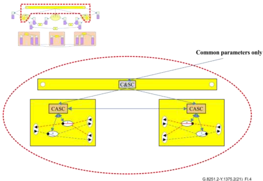
Figure I.4 – Showing a high-level abstract controller in a 1:1 case
