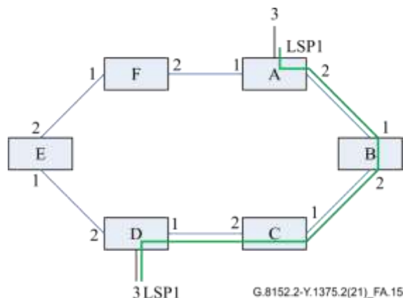
Figure A.15 – Basic network
