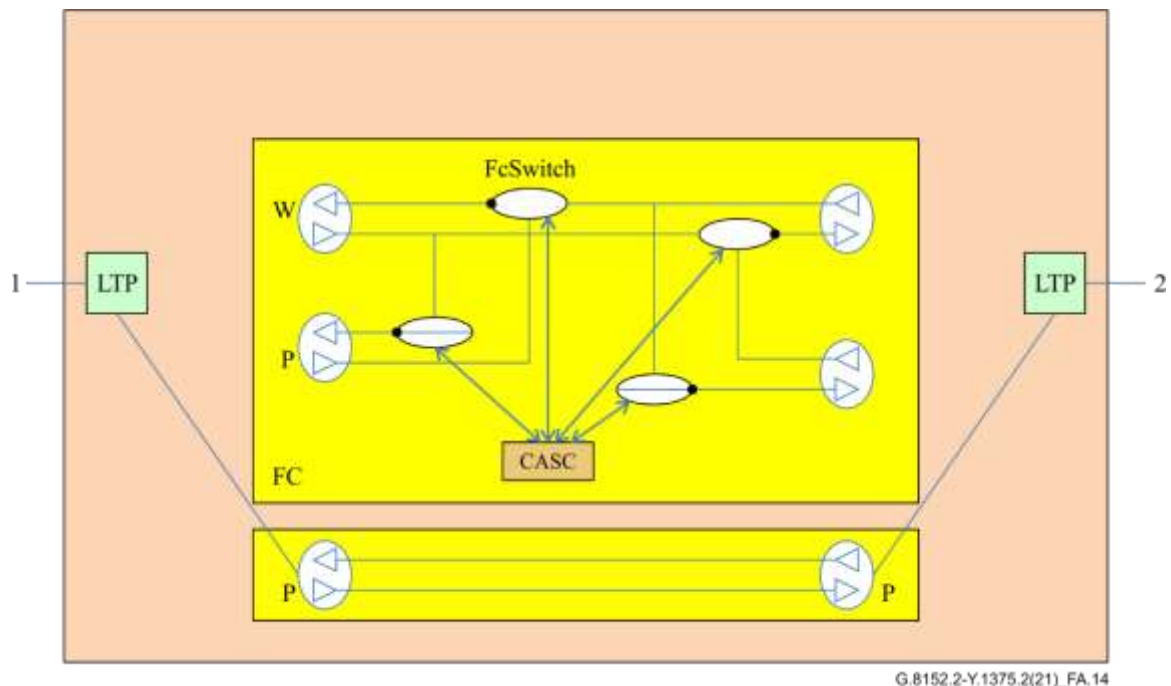
Figure A.14 – Steering: Node E and node F with failure on link between node B and node C
