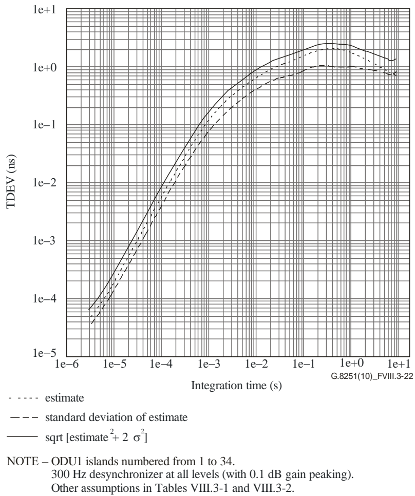
Figure VIII.3-22 – CBR2G5 client short-term wander (TDEV) results for Case 4 (Model 2)
