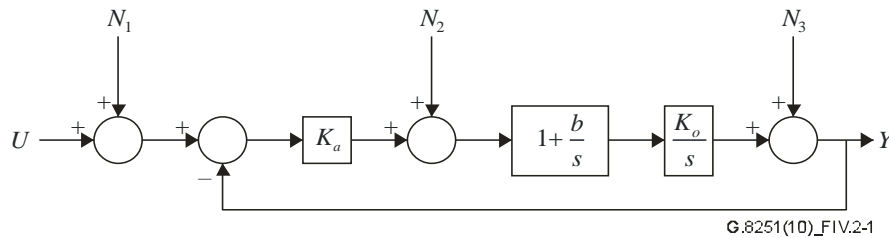
Figure IV.2-1 – Regenerator model
