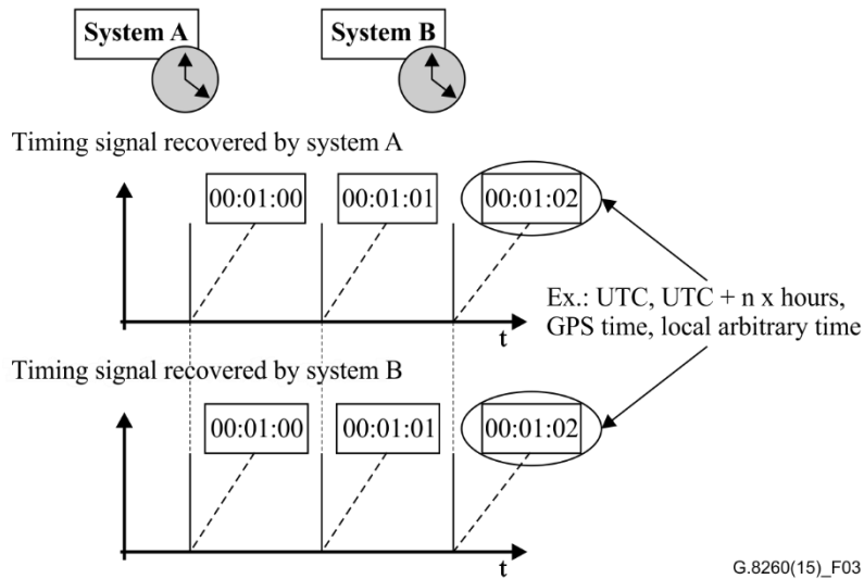
Figure 3 – Time synchronization
