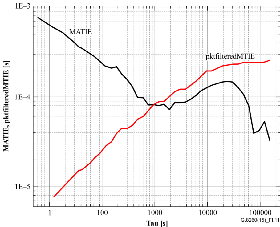
Figure I.11 – Example MATIE and pktfilteredMTIE data
