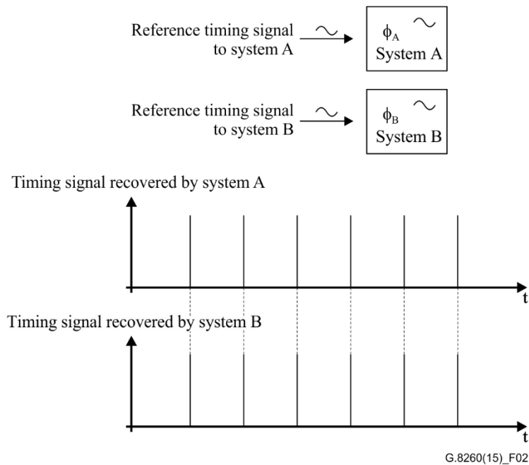
Figure 2 – Phase synchronization
