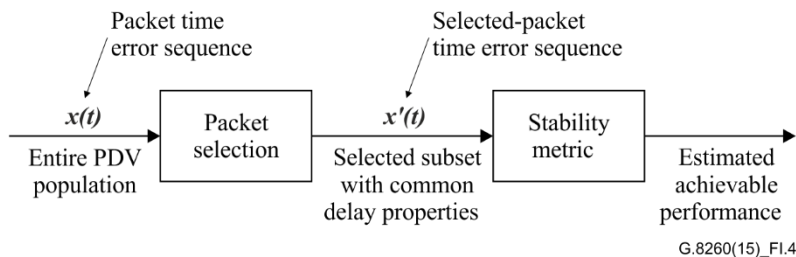
Figure I.4 – Pre-processed packet selection
