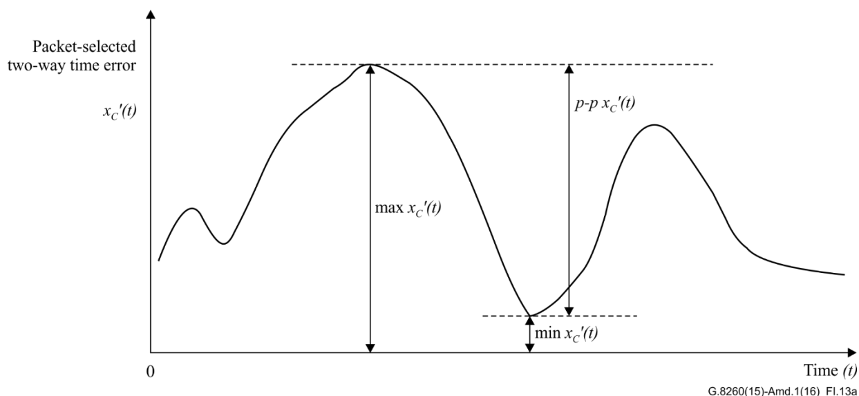
Figure I.13a – Packet-selected two-way time error sequence and derived values
