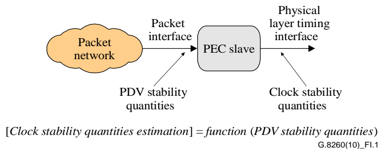
Figure I.1 – Packet equipment clock interfaces
