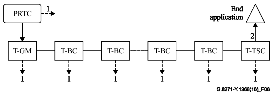
Figure 6 – Possible locations of external time and phase interfaces in a chain of Telecom-boundary clocks
