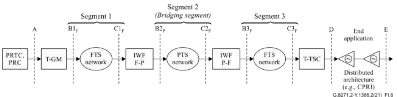
Figure I.6 – Bridging across a PTS network (CPRI – common public radio interface)
