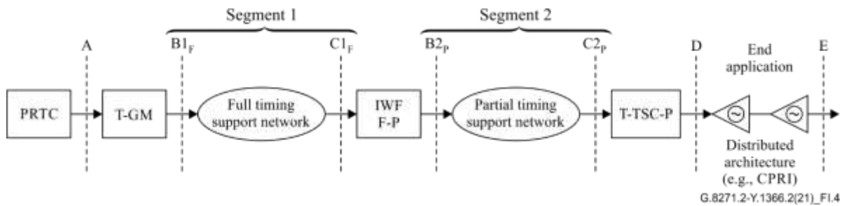
Figure I.4 – Deployment case 2b (CPRI – common public radio interface)
