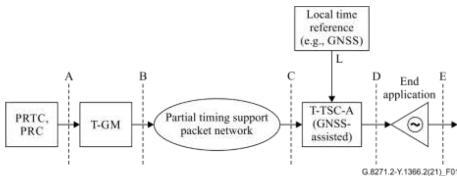
Figure 1 – Reference model for network limits for APTS
