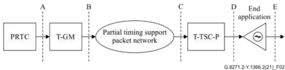
Figure 2 – Reference model for network limits for PTS
