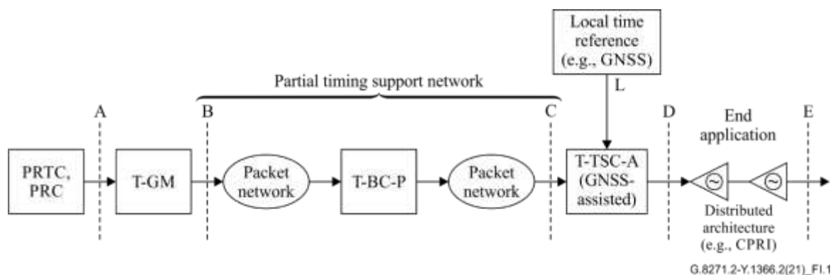
Figure I.1 – Deployment case 1a (CPRI – common public radio interface)
