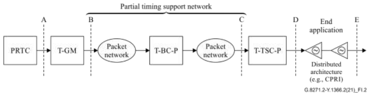
Figure I.2 – Deployment case 1b (CPRI – common public radio interface)
