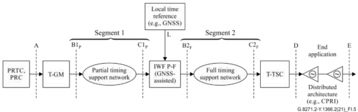
Figure I.5 – APTS network followed by a full timing support network (CPRI – common public radio interface)
