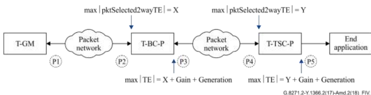
Figure IV.1 – Example network showing noise accumulation model
