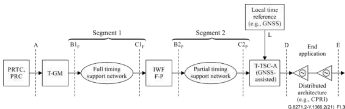
Figure I.3 – Deployment case 2a (CPRI – common public radio interface)
