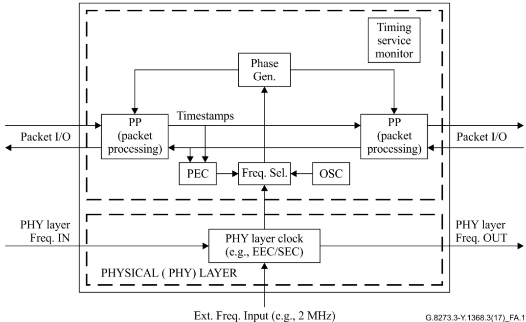
Figure A.1 – Transparent clock model
