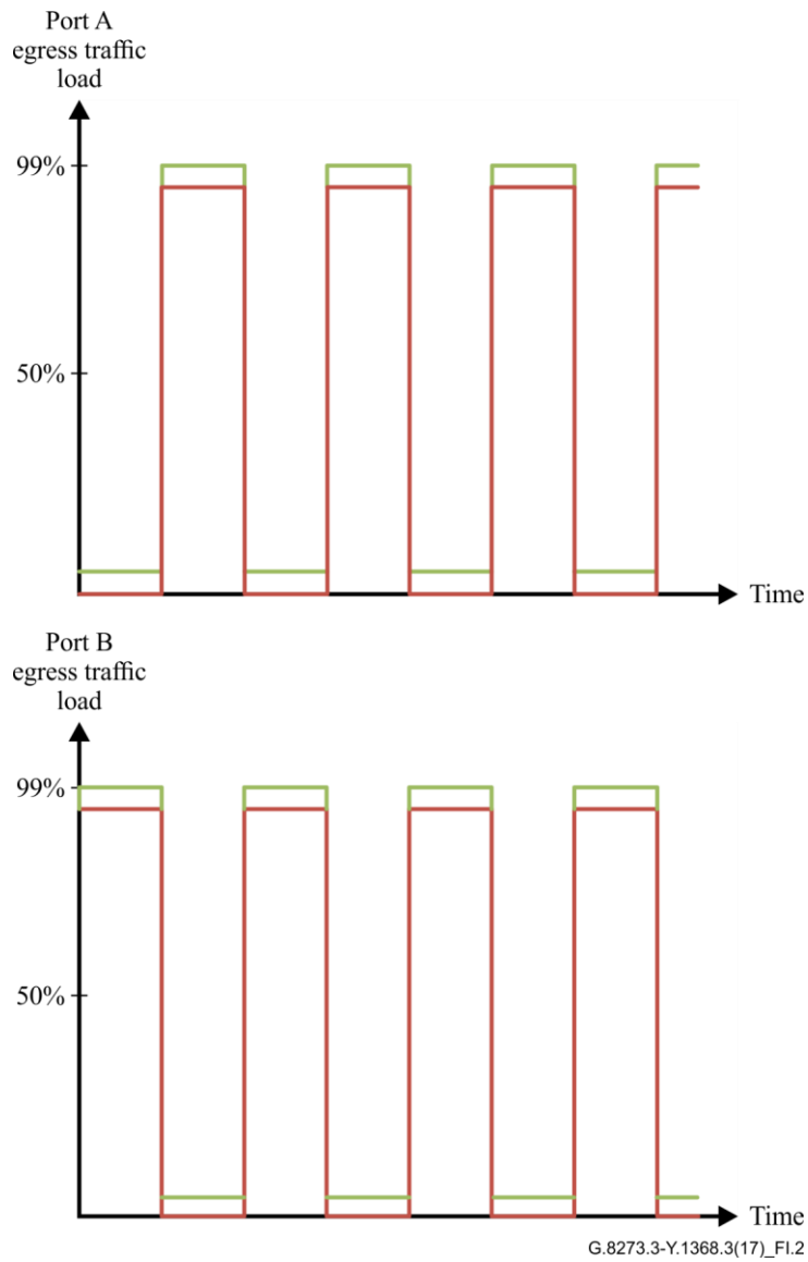
Figure I.2 – Cross traffic pattern
