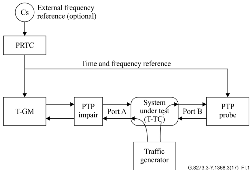
Figure I.1 – T-TC test set-up with cross traffic
