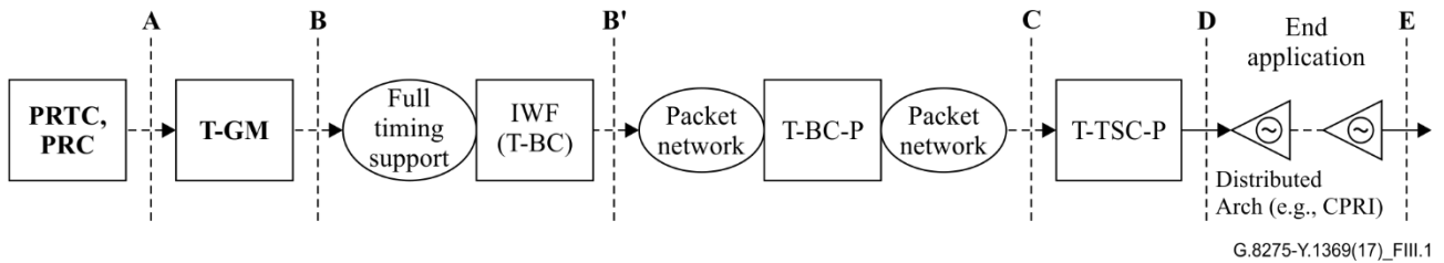
Figure III.1 – Deployment case requiring IWF
