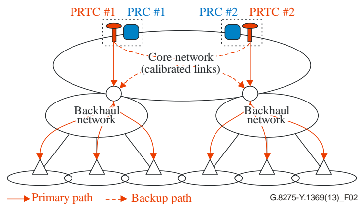
Figure 2 – Architecture with centralized PRTC functions collocated with PRC
