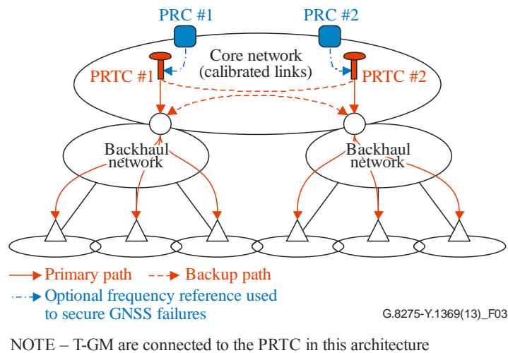
Figure 3 – Architecture with centralized PRTC functions not collocated with PRC
