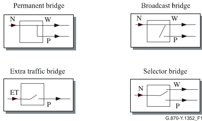
Figure 1 – Protection bridges
