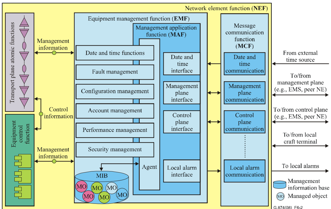
Figure 6-2 – Optical equipment management function
