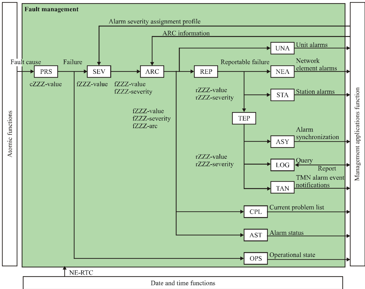
Figure 7-1 – Fault management within the OTN NEF
