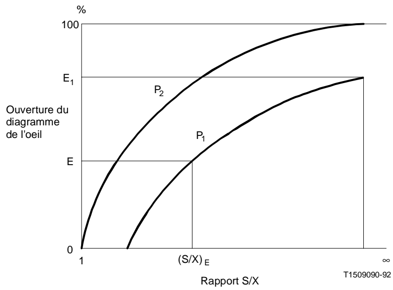
FIGURE III-3/G.957
