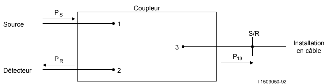
FIGURE II-1/G.957
