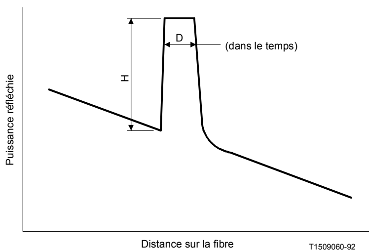
FIGURE II-2/G.957
