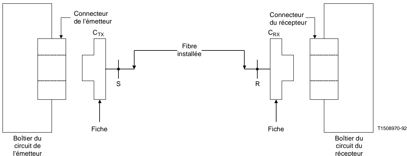
FIGURE 1/G.957
