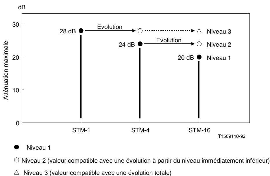
FIGURE IV-1/G.957
