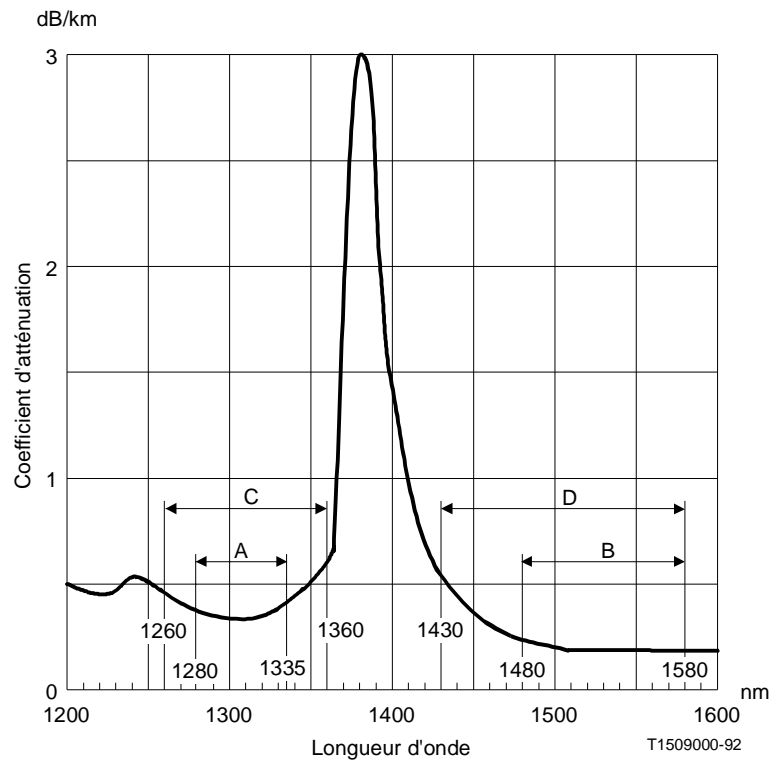
FIGURE A-1/G.957
