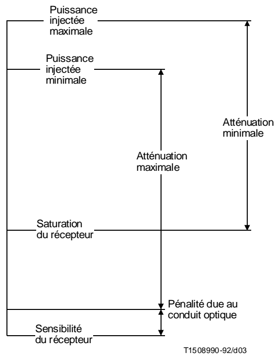
FIGURE 3/G.957
