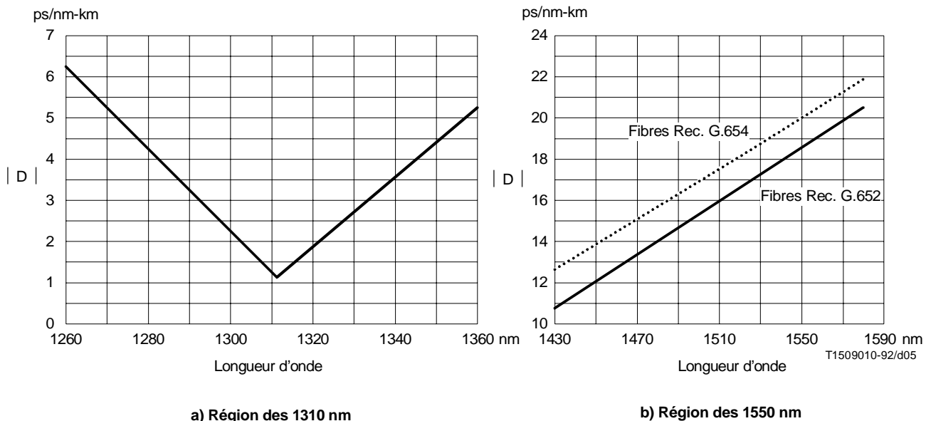
FIGURE A.2/G.957
