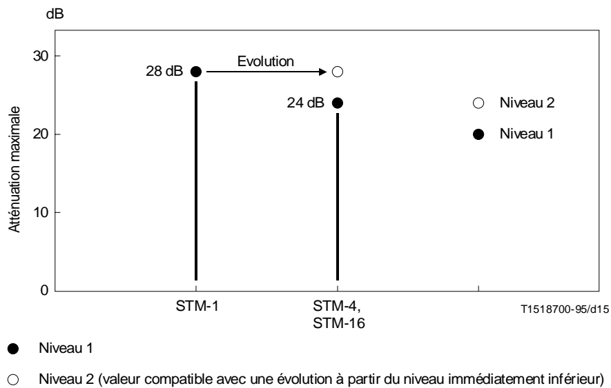
FIGURE III.1/G.957
