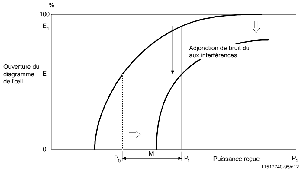
FIGURE II.2/G.957
