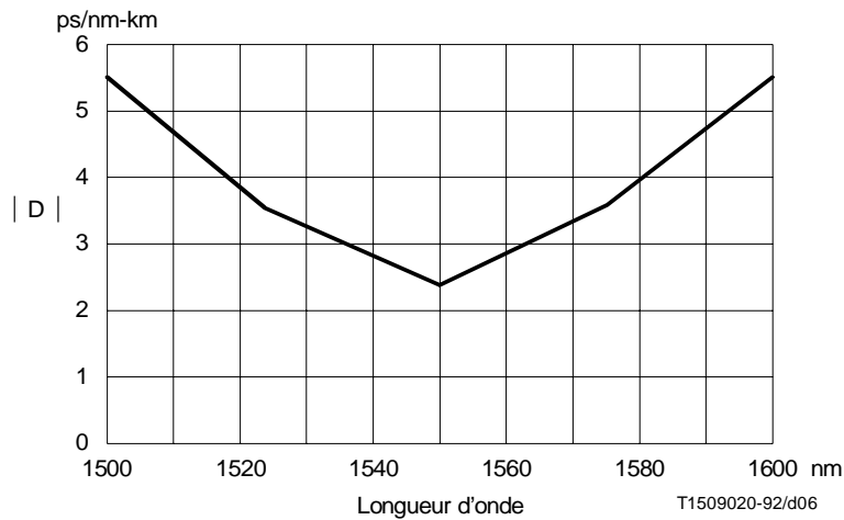
FIGURE A.3/G.957
