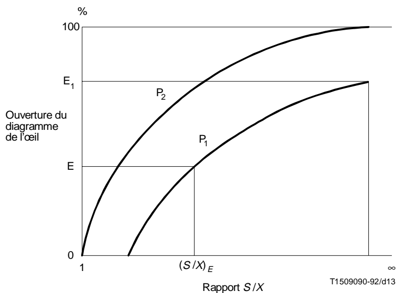
FIGURE II.3/G.957
