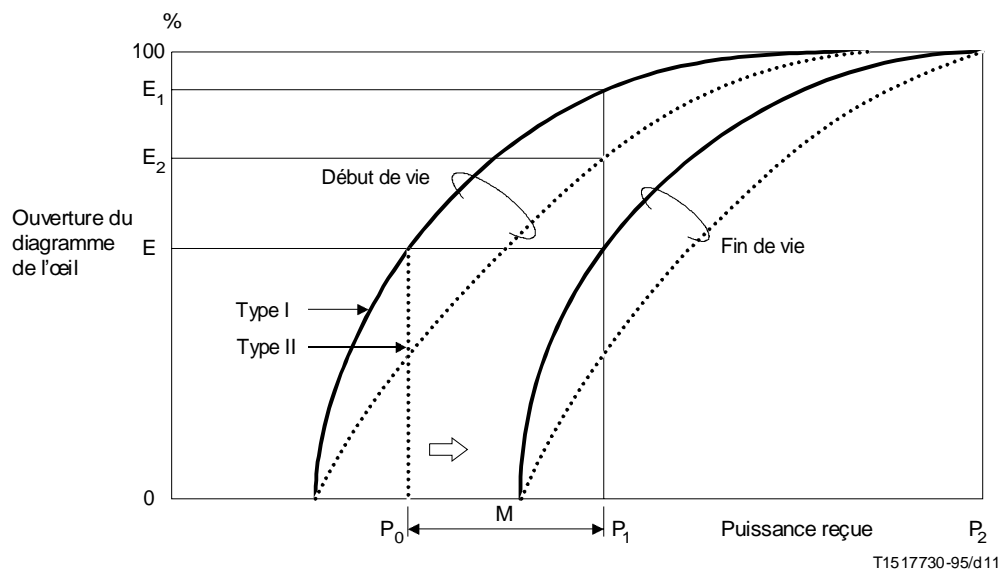
FIGURE II.1/G.957
