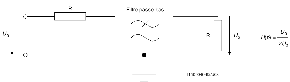
FIGURE B.2/G.957
