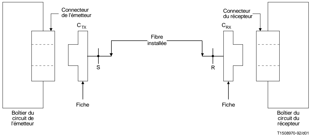
FIGURE 1/G.957
