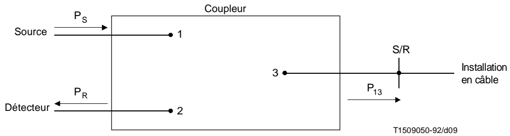
FIGURE I.1/G.957
