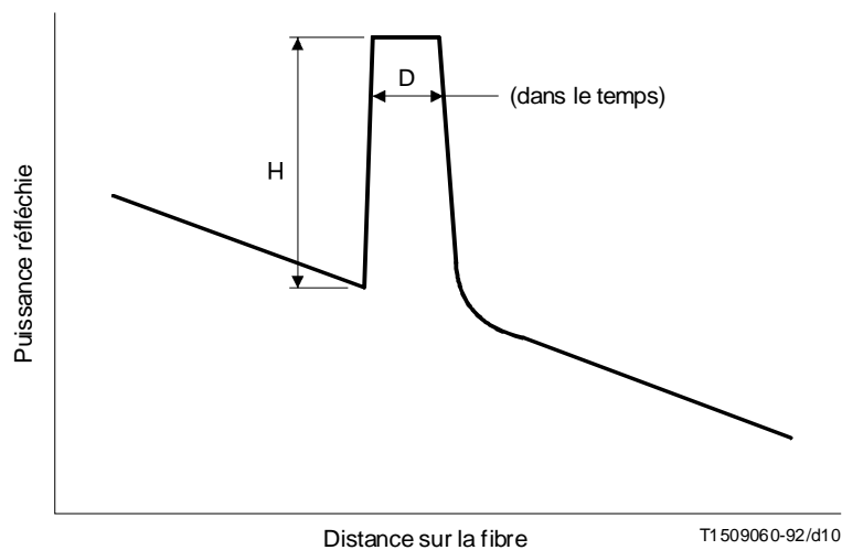
FIGURE I.2/G.957
