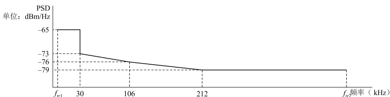
图7-1 – 424MHz PSD类型的带内极限PSD掩膜
