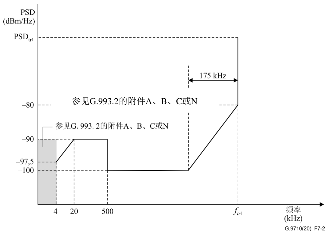
图7-2 – 低频端的带外LPM
