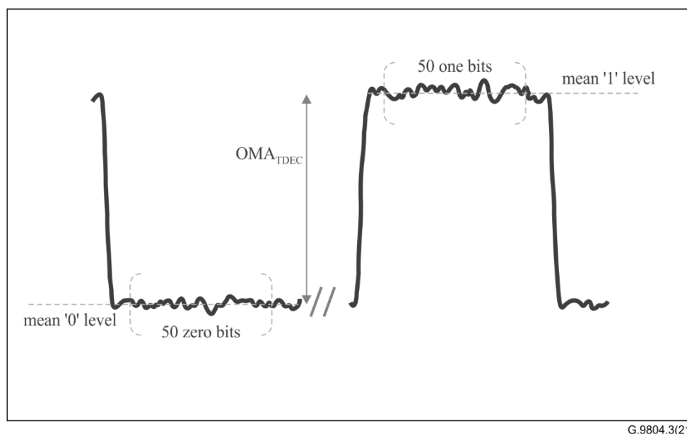
Figure 9-8 – Illustration of the OMA measurement
