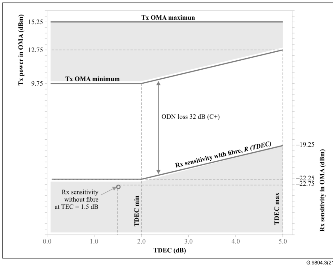
Figure 9-1 – Illustration of the relationship between transmitter power, receiver sensitivity and TDEC for 49.7664 Gbit/s downstream (C+ OPL class)
