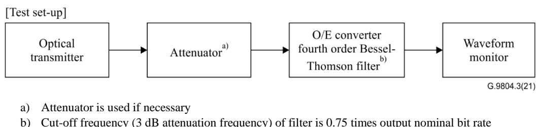
Figure 9-6 – Test set-up for mask of the eye diagram for ONU transmitter
