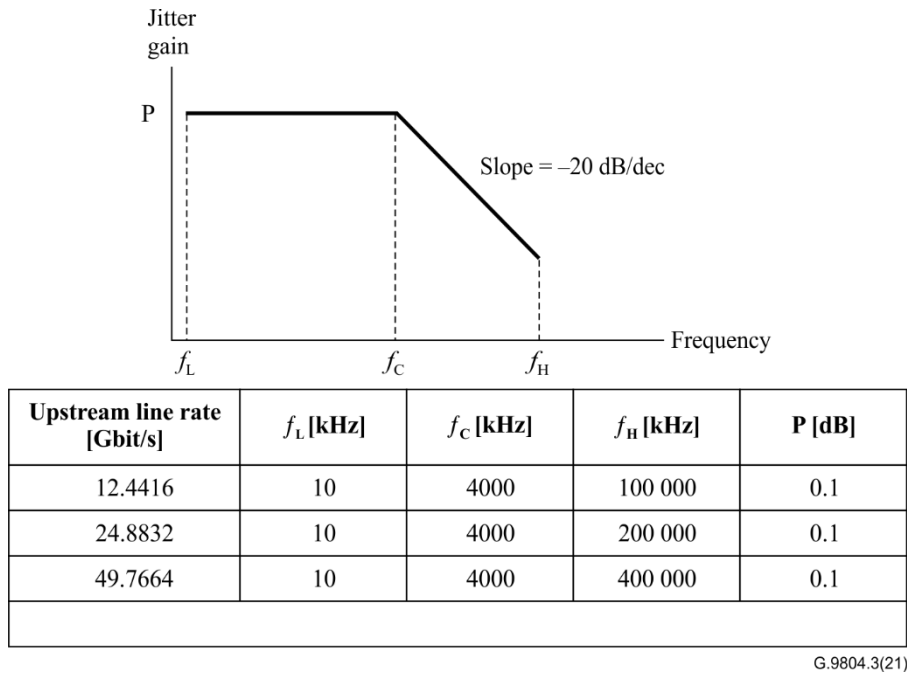
Figure 9-10 – Jitter transfer mask for ONU
