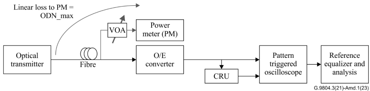
Figure 9-9a – Illustration of the TDEC measurement in the non-linear fibre regime
