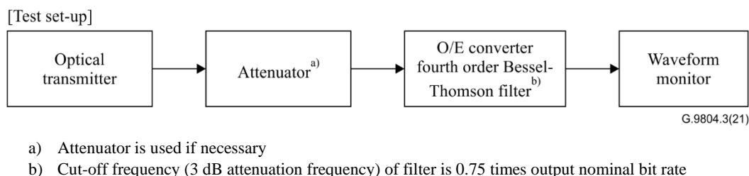
Figure 9-4 – Test set-up for mask of the eye diagram for OLT transmitter
