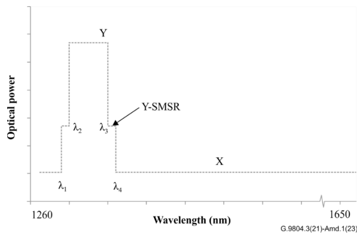
Figure 9-1a – ONU transmitter OOB-PSD mask definition
