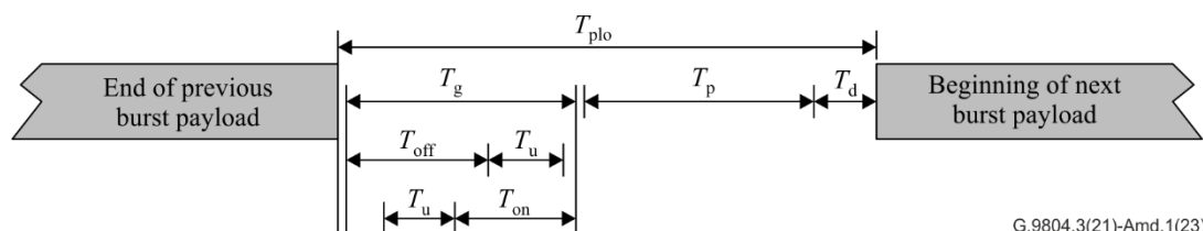
Figure III.1 – Timing relationship between the various physical layer overhead times
