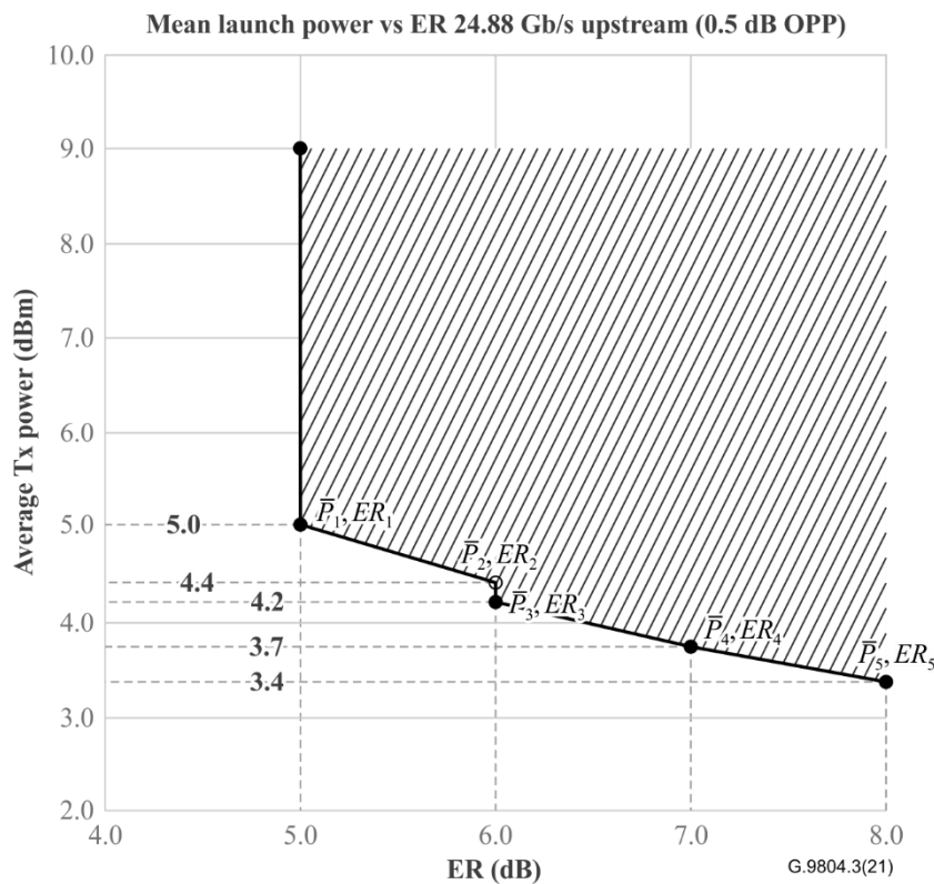
Figure I.2 –Transmitter power and ER admissible region (hatched) for 24.8832 Gbit/s upstream when OPP = 0.5dB
