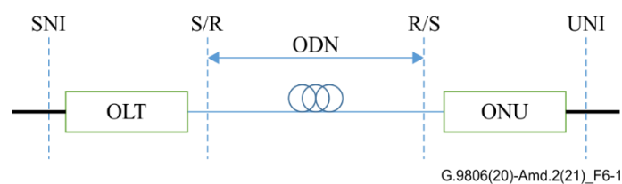
Figure 6-1 – System configuration
