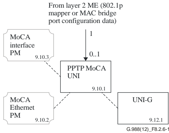
Figure 8.2.6-1 – Multimedia over C eoax A lliance
