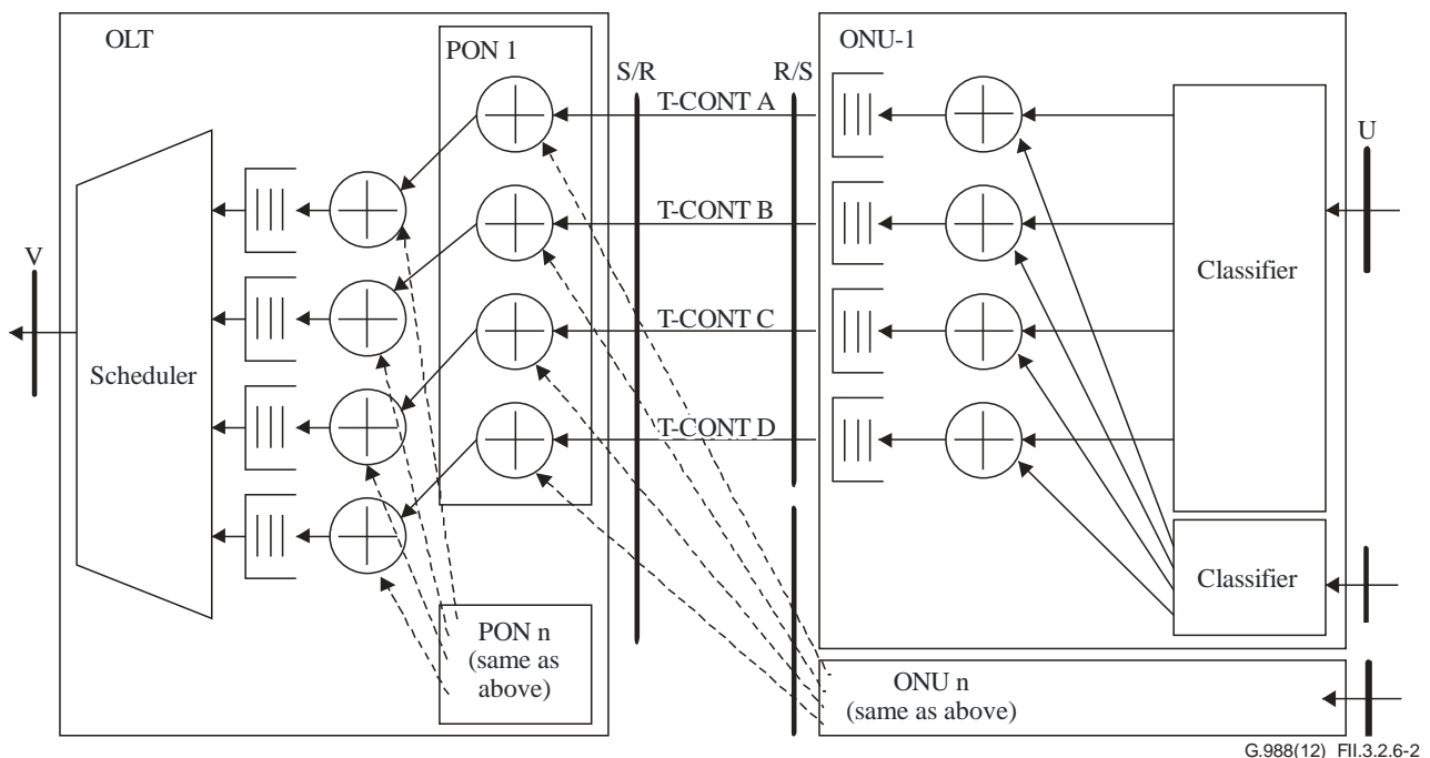
Figure II.3.2.6-2 – Upstream functionality example
