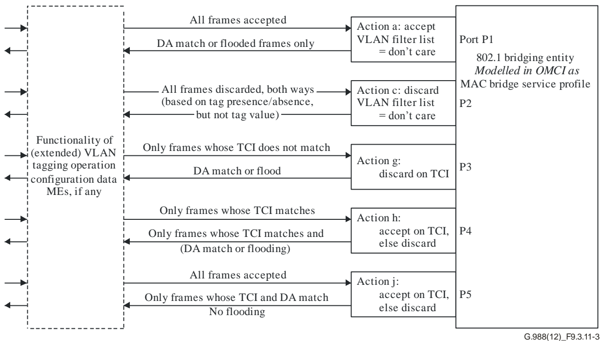
Figure 9.3.11-3 – Forwarding behaviour
