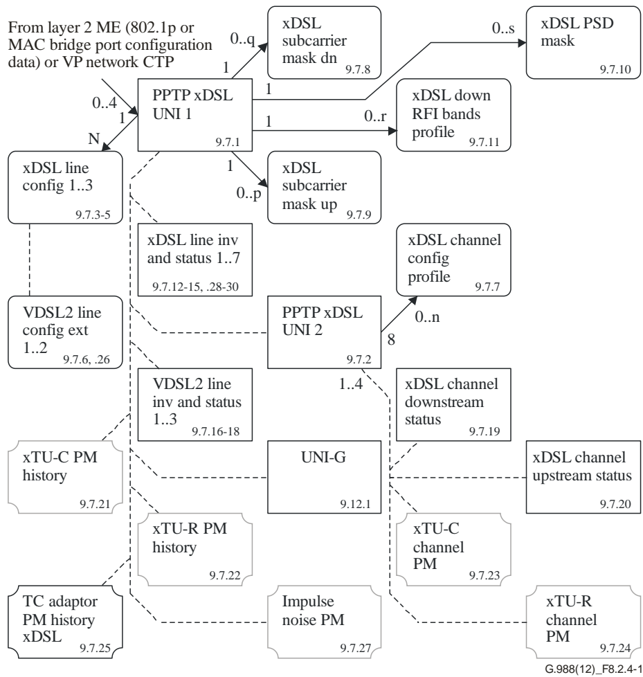
Figure 8.2.4-1 – xDSL
