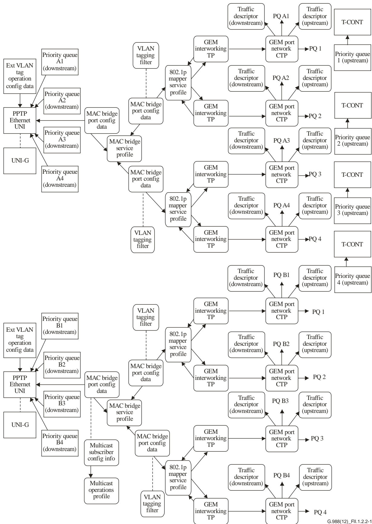
Figure II.1.2.2-1 – Multi-UNI L2-OCM
