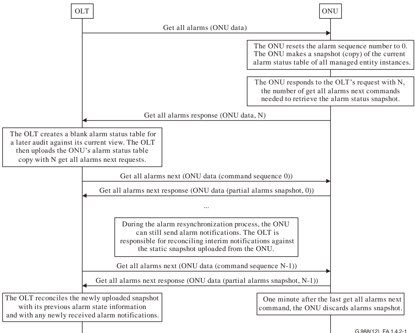
Figure A.1.4.2-1 – Alarm resynchronization
