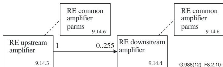
Figure 8.2.10-1 – Mid-span PON reach extender core (repeater)
