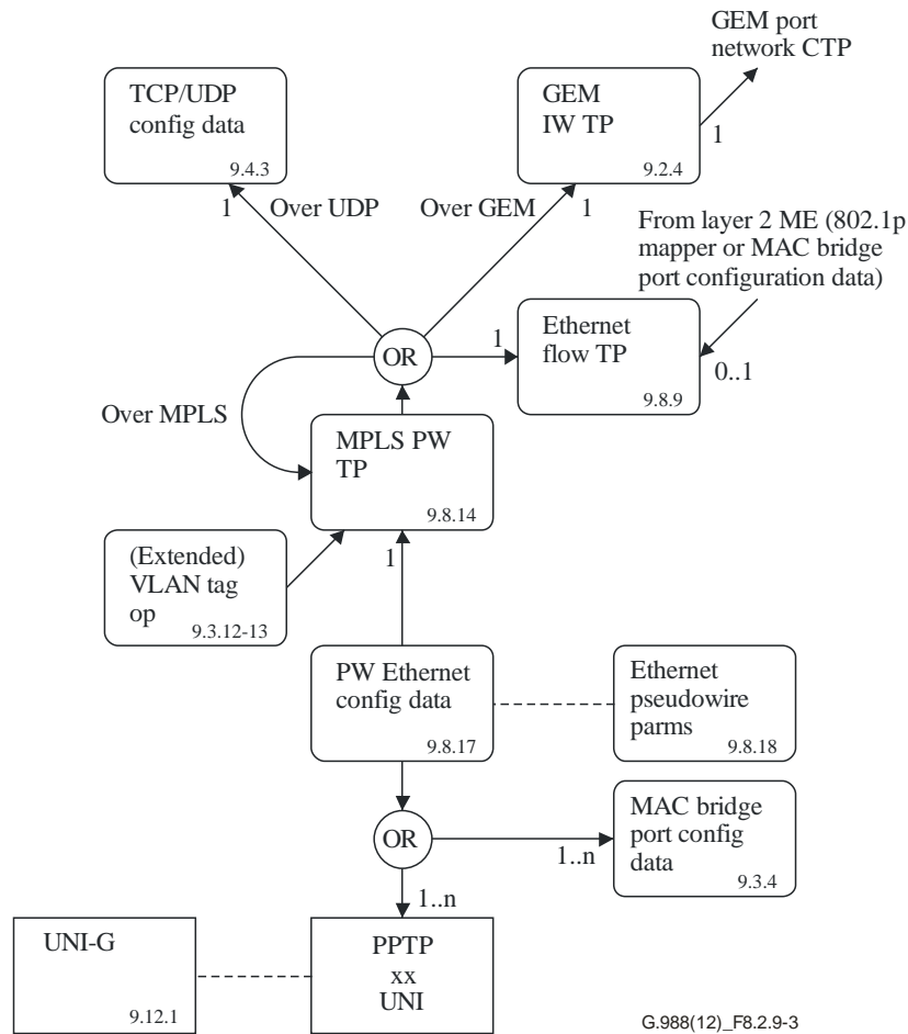
Figure 8.2.9-3 – Ethernet pseudowire
