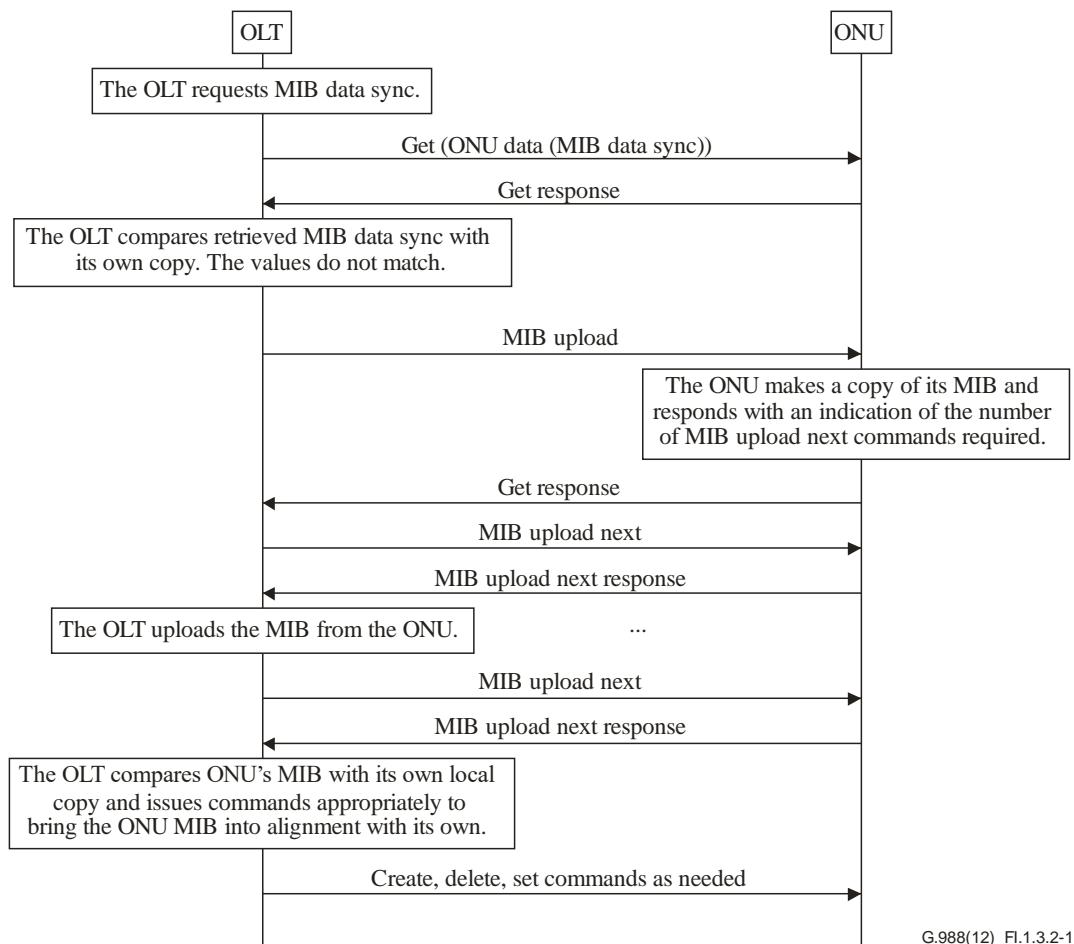
Figure I.1.3.2-1 – MIB resynchronization
