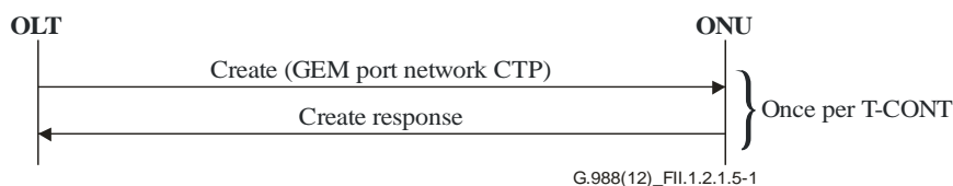
Figure II.1.2.1.5-1 – L2-OCM message flow – Step 1
