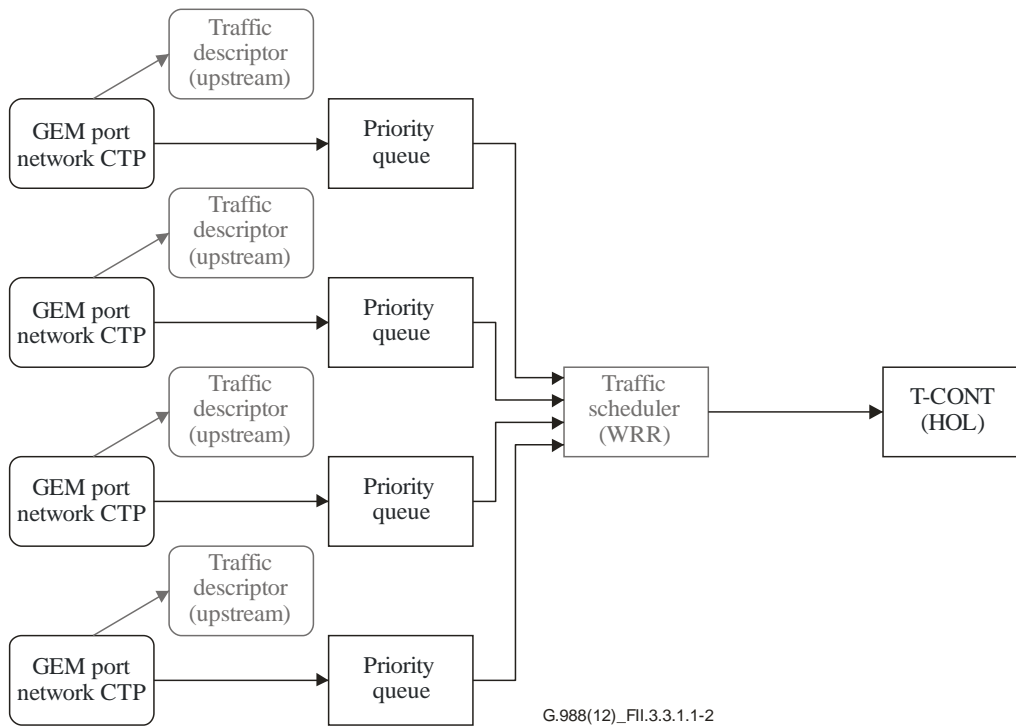
Figure II.3.3.1.1-2 – Example of weighted scheduling with four queues per T-CONT and traffic scheduler, queues connected to traffic scheduler
