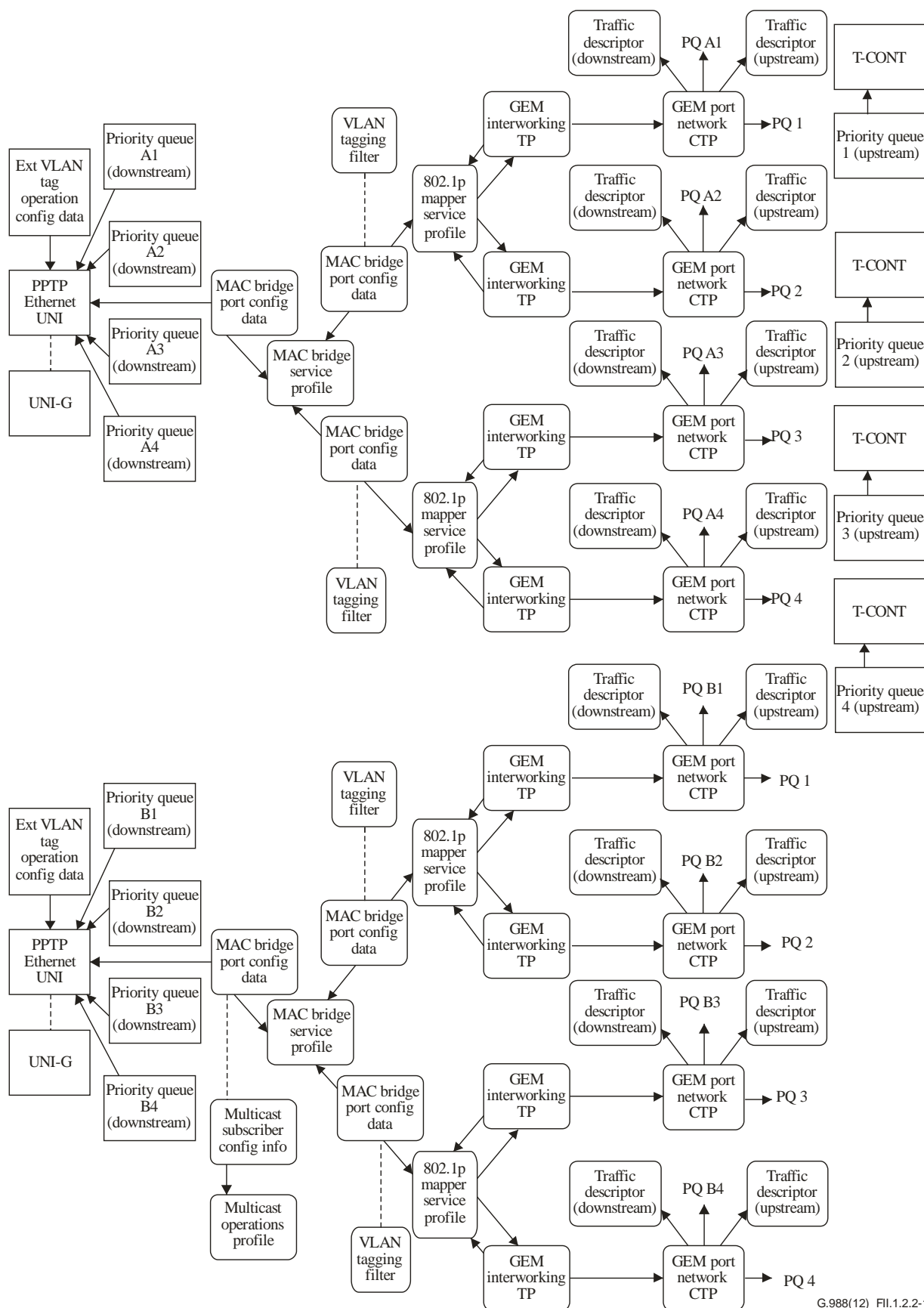
Figure II.1.2.2-1 – Multi-UNI L2-OCM
