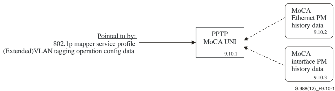
Figure 9.10-1 – Managed entities associated with home networking
