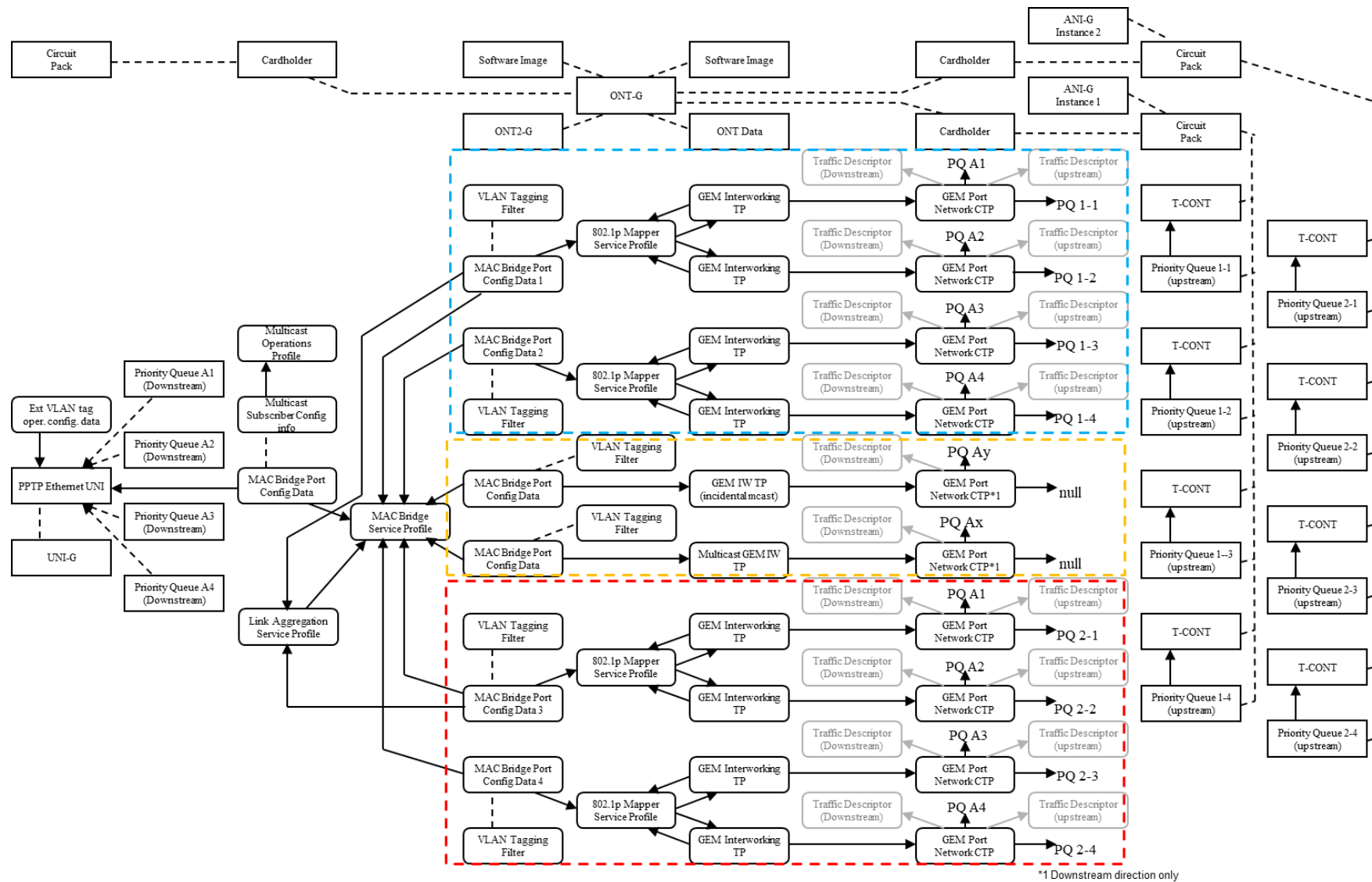
Figure II.5-2 – Supporting LAG-based channel bonding in an ONU (based on ITU-T G.988 Figure II.1.2.1-1 – Single UNI, VLANs with common priorities)
