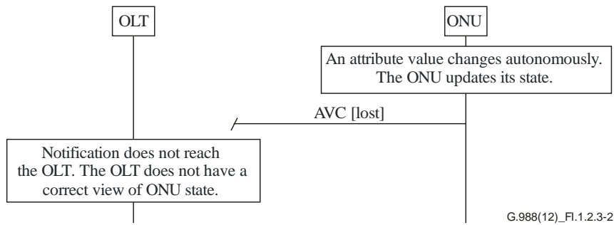
Figure I.1.2.3-2 – Lost AVC
