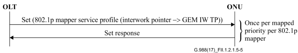
Figure II.1.2.1.5-5 – L2-OCM message flow – Step 5
