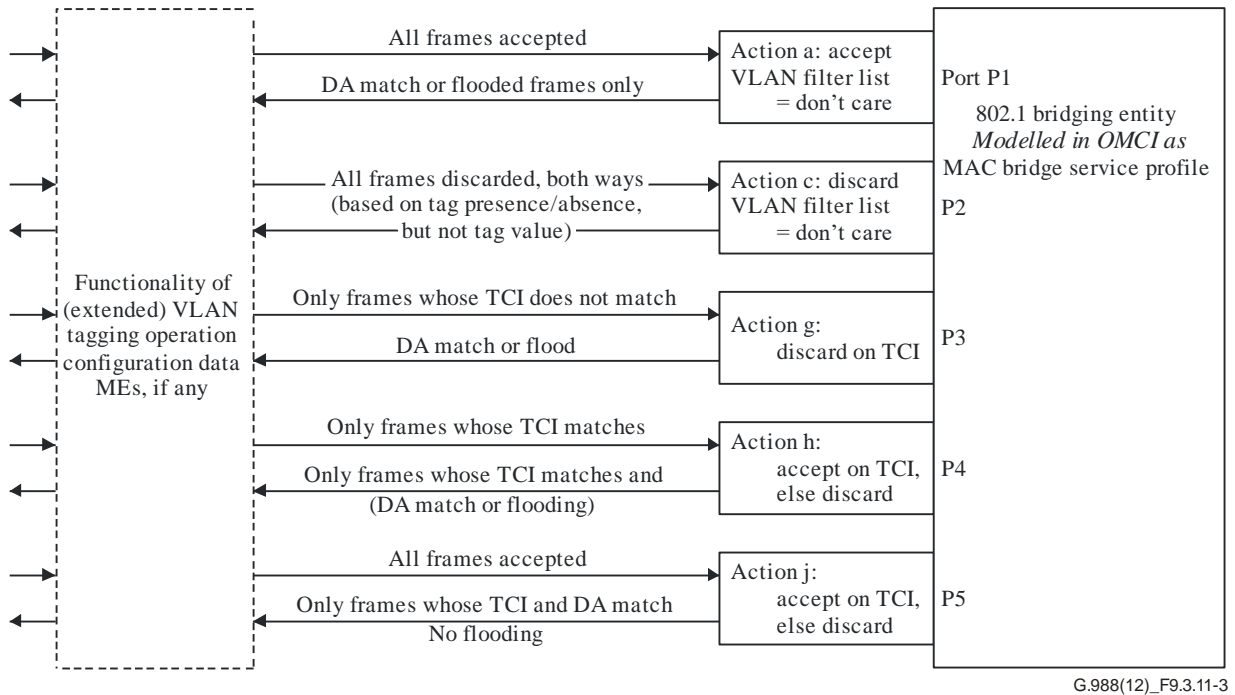
Figure 9.3.11-3 – Forwarding behaviour
