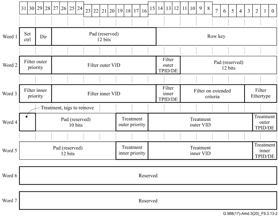
Figure 9.3.13-2 – Enhanced received frame classification and processing layout
