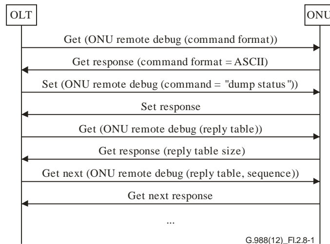
Figure I.2.8-1 – Success example
