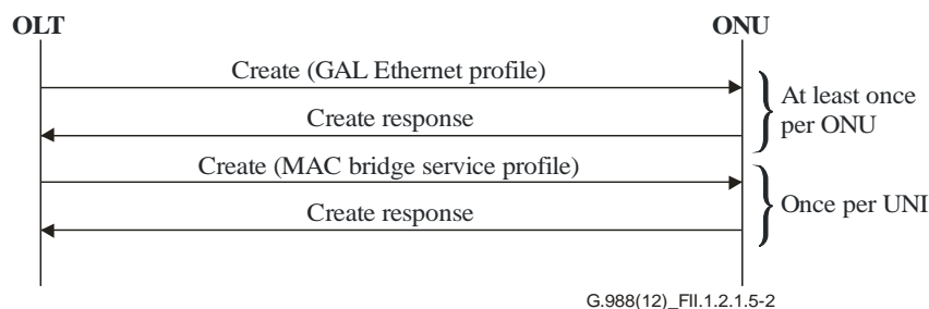
Figure II.1.2.1.5-2 – L2-OCM message flow – Step 2
