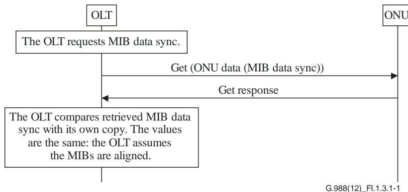
Figure I.1.3.1-1 – MIB audit
