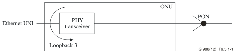
Figure 9.5.1-1 – Ethernet loopback configuration
