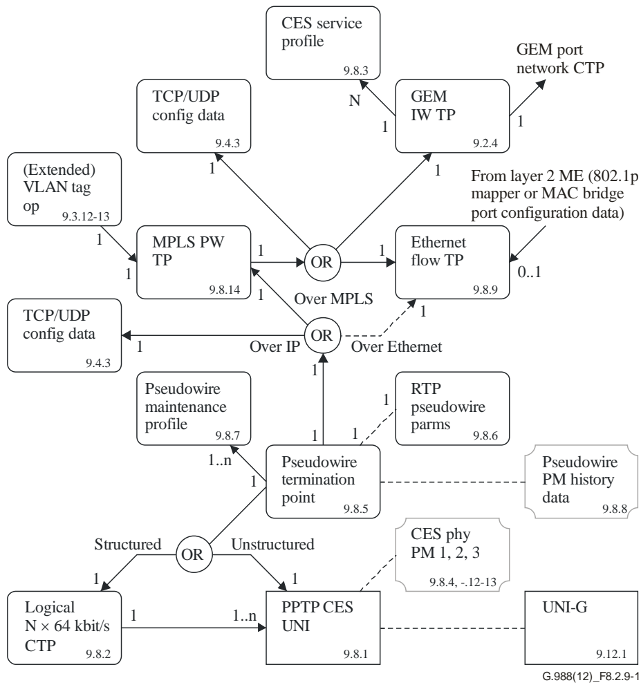
Figure 8.2.9-1 – Time division multiplex pseudowire
