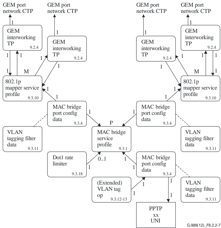
Figure 8.2.2-7 – Illustration of 1:MP map-filtering
