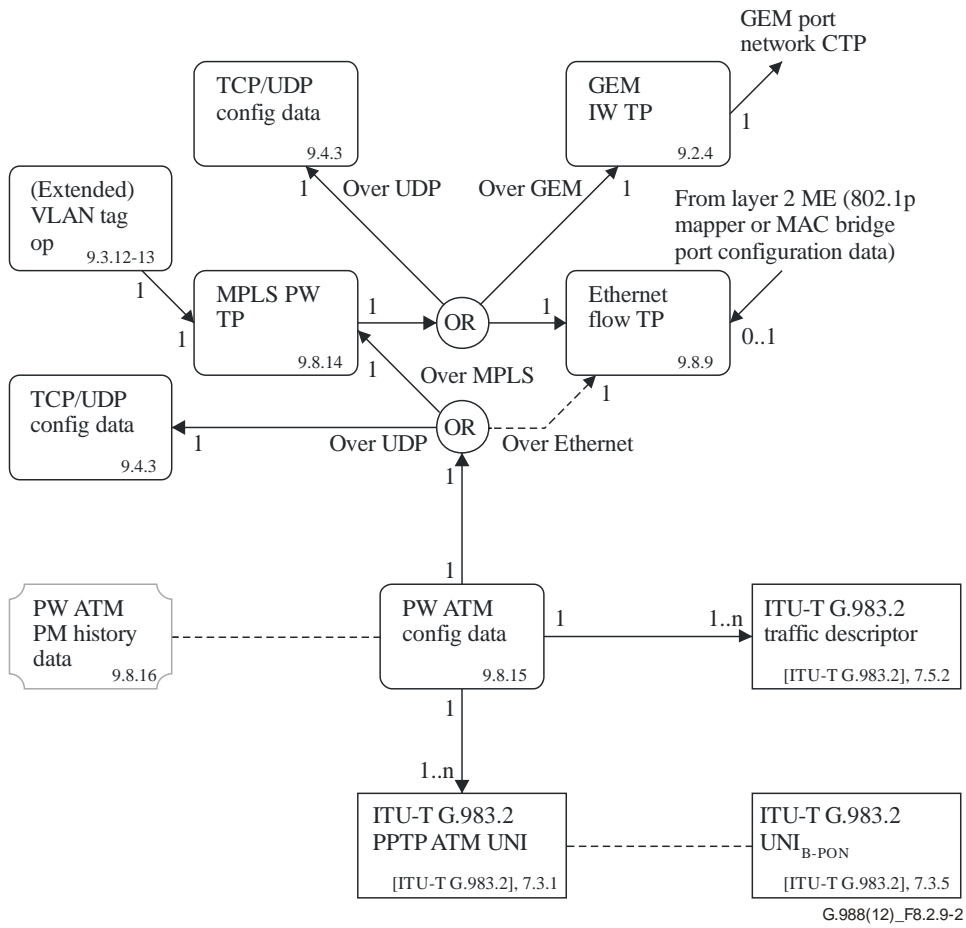
Figure 8.2.9-2 – ATM pseudowire
