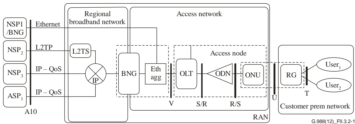
Figure II.3.2-1 – High-level architecture
