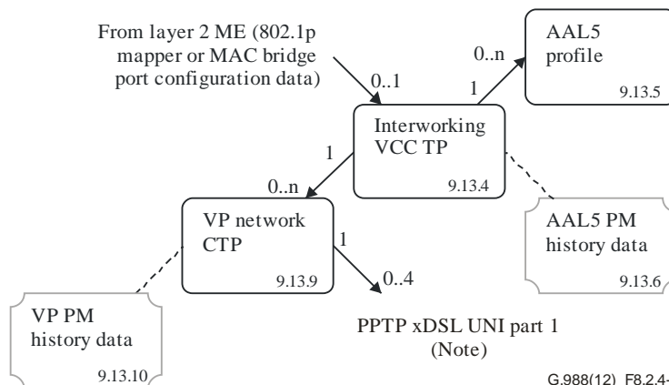
Figure 8.2.4-1 – ME relation diagram for xDSL (ADSL and VDSL) services
