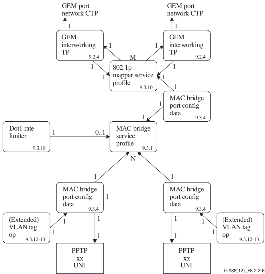
Figure 8.2.2-6 – Illustration of N:M bridge-mapping
