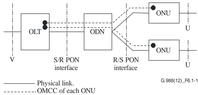
Figure 6.1-1 – Reference model, OMCI
