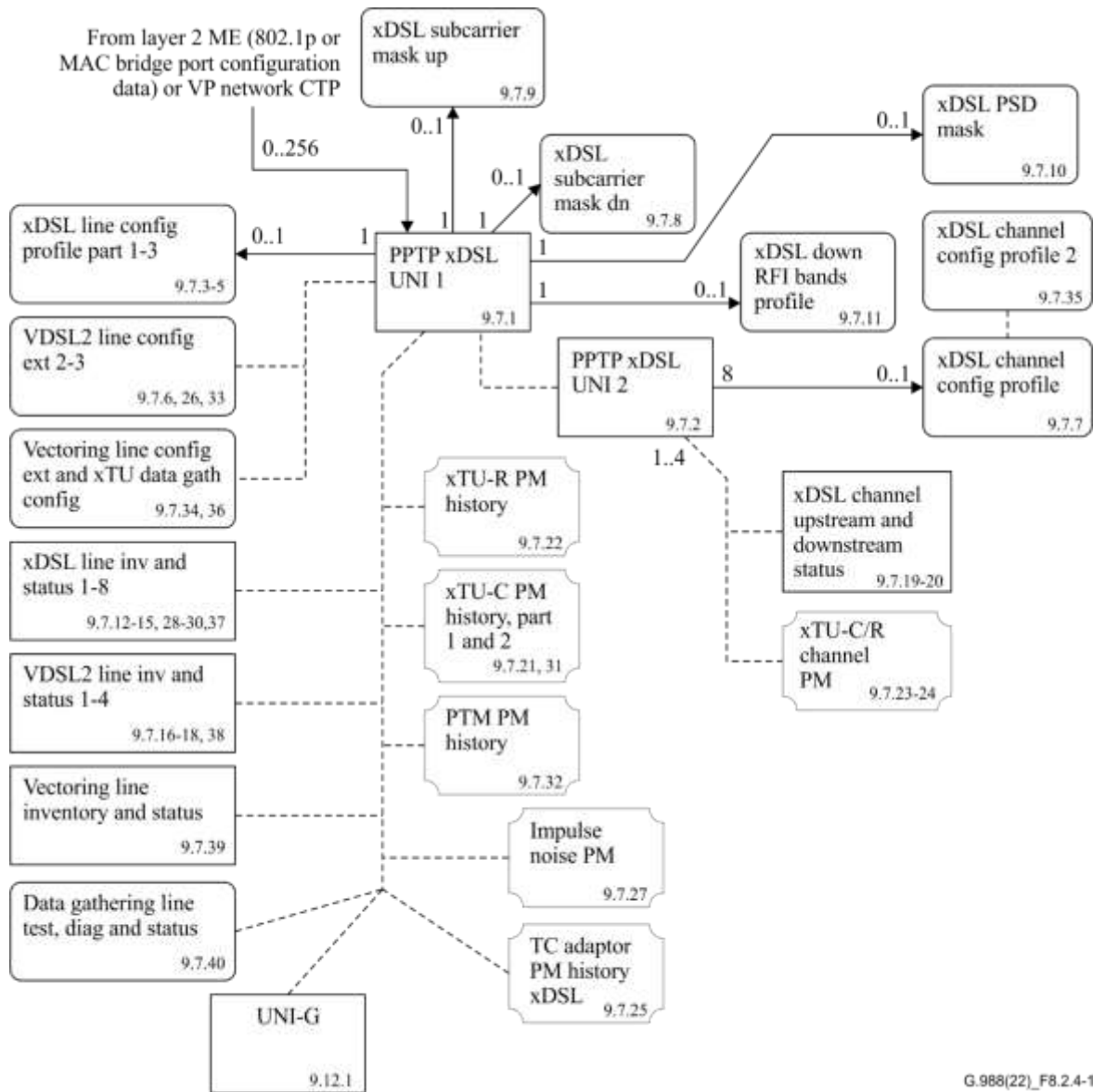
Figure 8.2.4-1 – ME relation diagram for xDSL (ADSL and VDSL) services
