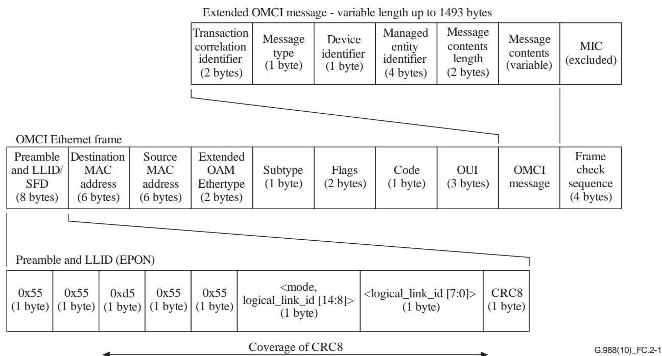
Figure C.2-1 – Extended OAM frame structure for EPON OMCI
