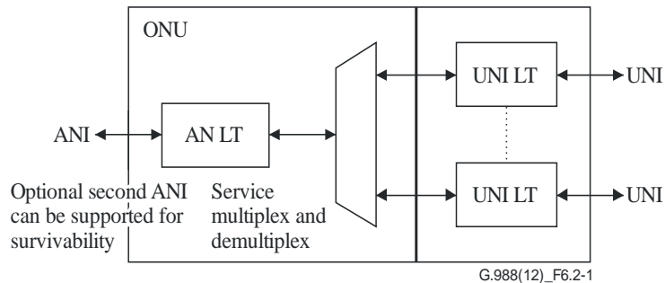
Figure 6.2-1 – ONU functional block diagram
