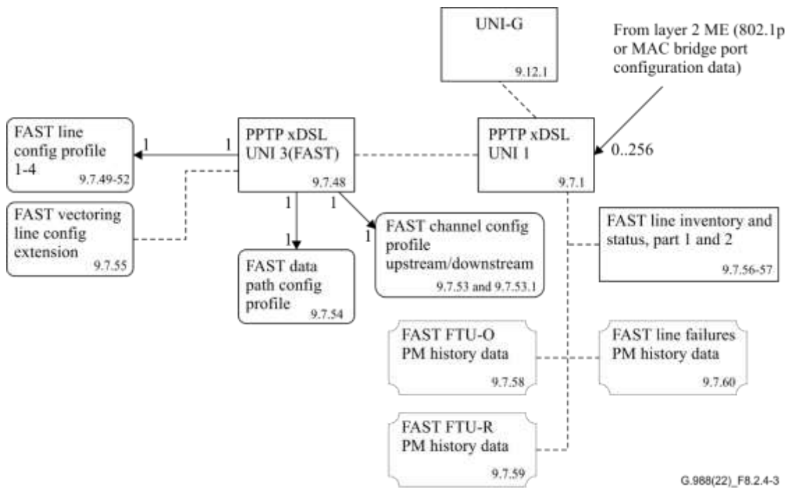
Figure 8.2.4-3 – ME relations diagram for G.fast (FAST) service
