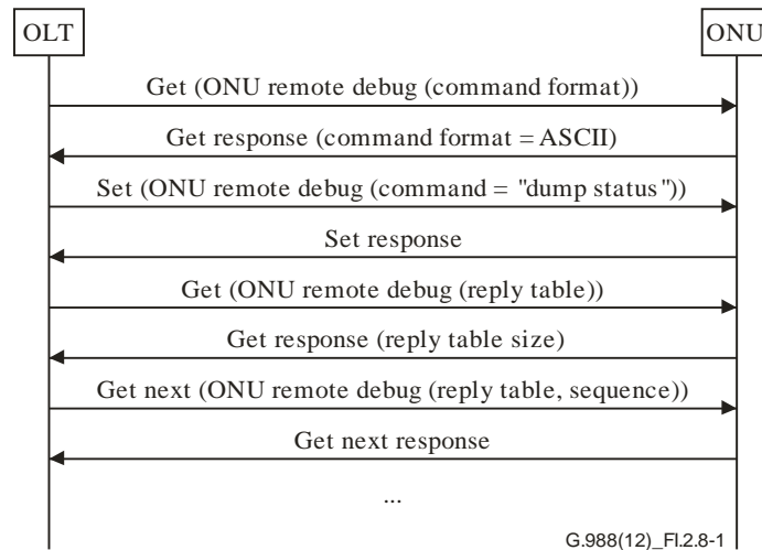
Figure I.2.8-1 – Success example
