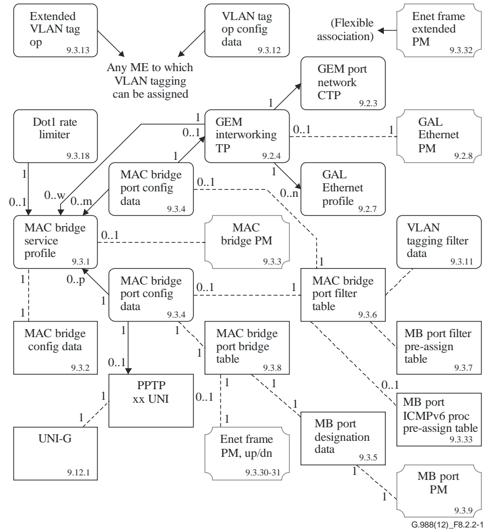
Figure 8.2.2-1 – MAC bridged LAN
