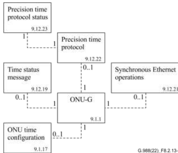
Figure 8.2.13-1 – ONU packet-based Time Synchronization
