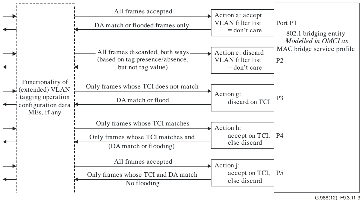
Figure 9.3.11-3 – Forwarding behaviour
