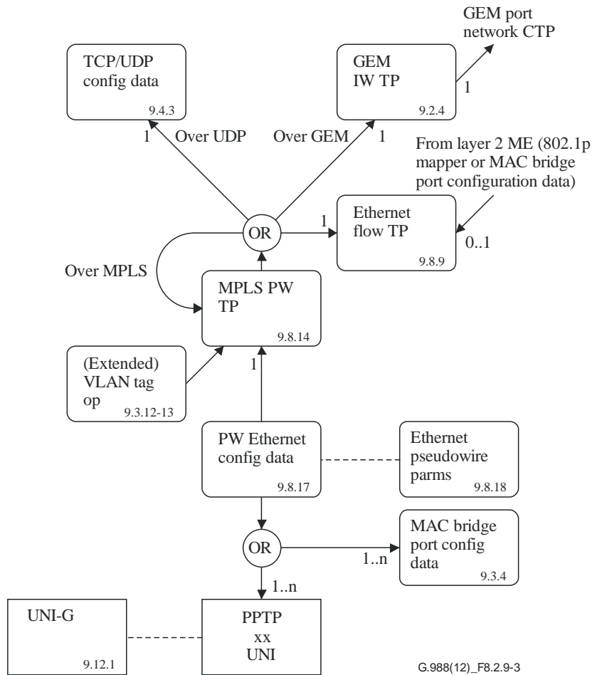
Figure 8.2.9-3 – Ethernet pseudowire
