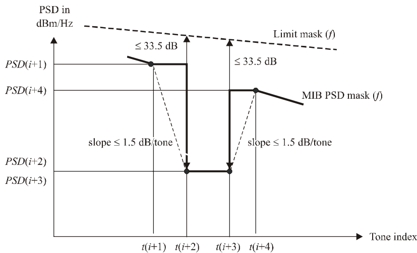
Figure 8.5.1-1/G.992.5 – Restrictions on breakpoints and MIB PSD mask (f)
