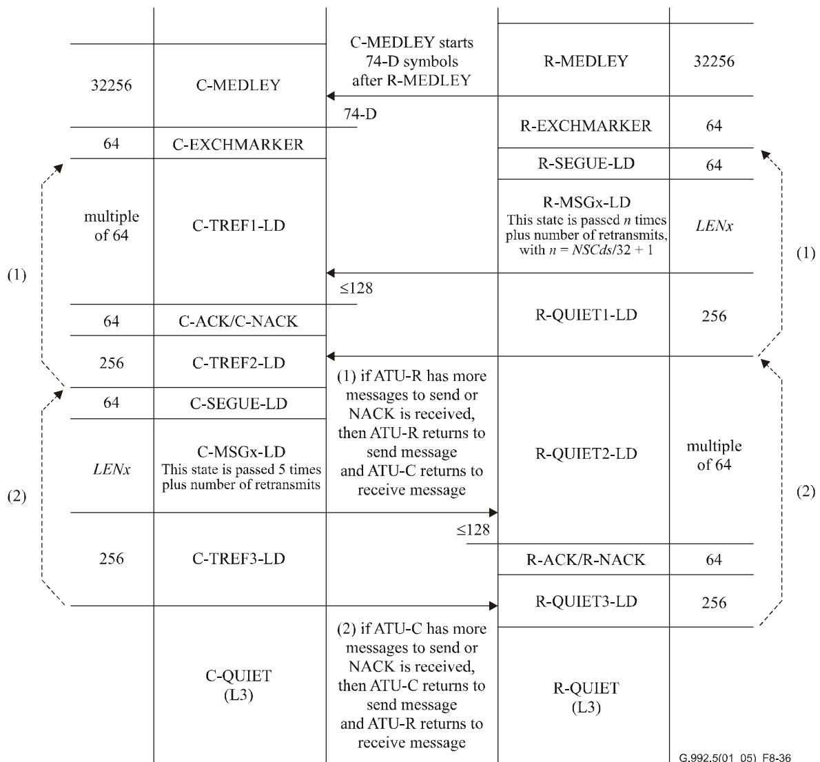
Figure 8-36/G.992.5 – Loop diagnostics timing diagram (part 2)
