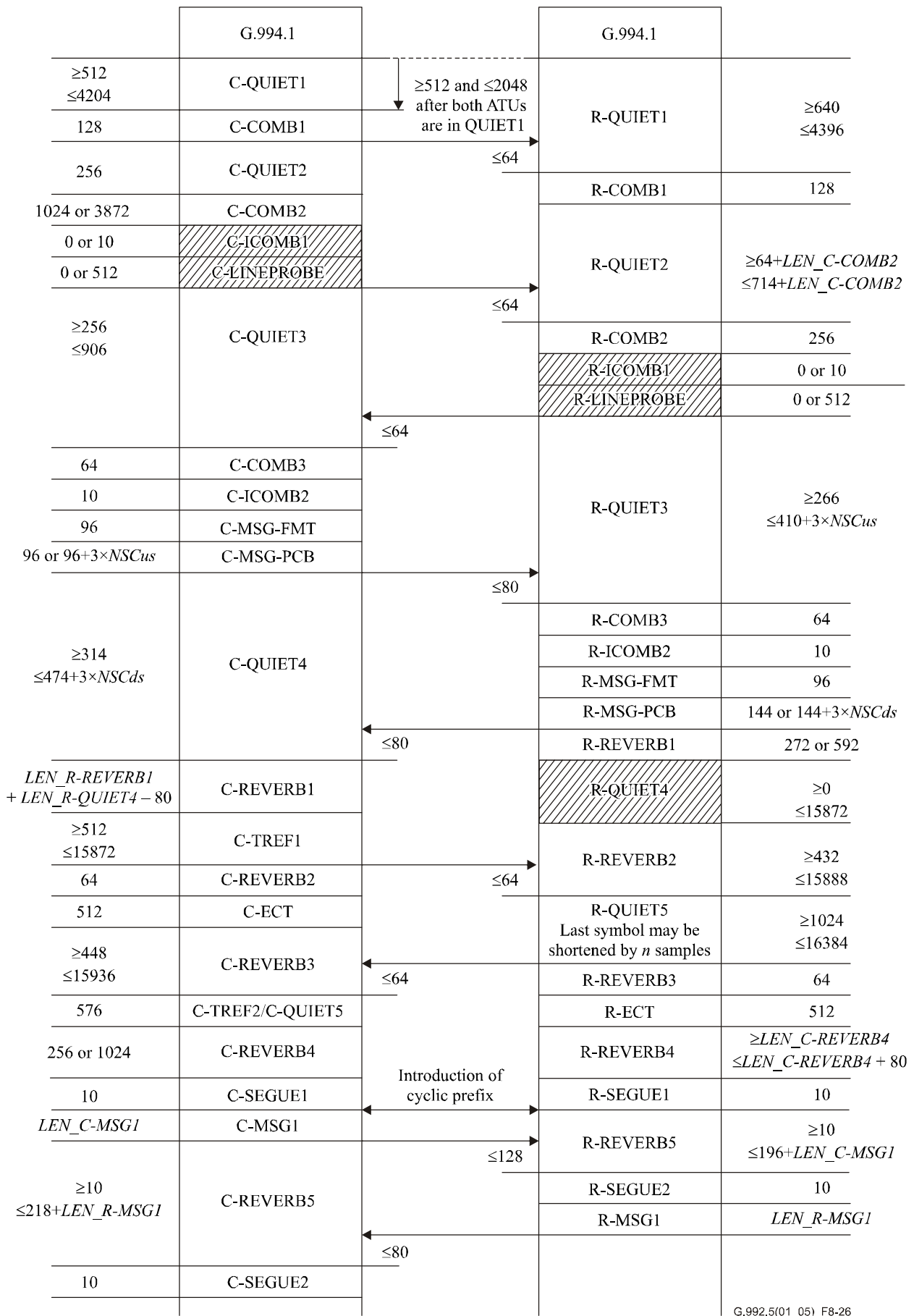
Figure 8-26/G.992.5 – Timing diagram of the initialization procedure (part 1)
