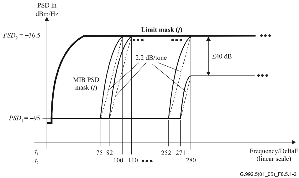
Figure 8.5.1-2/G.992.5 – Illustration of a stopband in the first part of the frequency band
