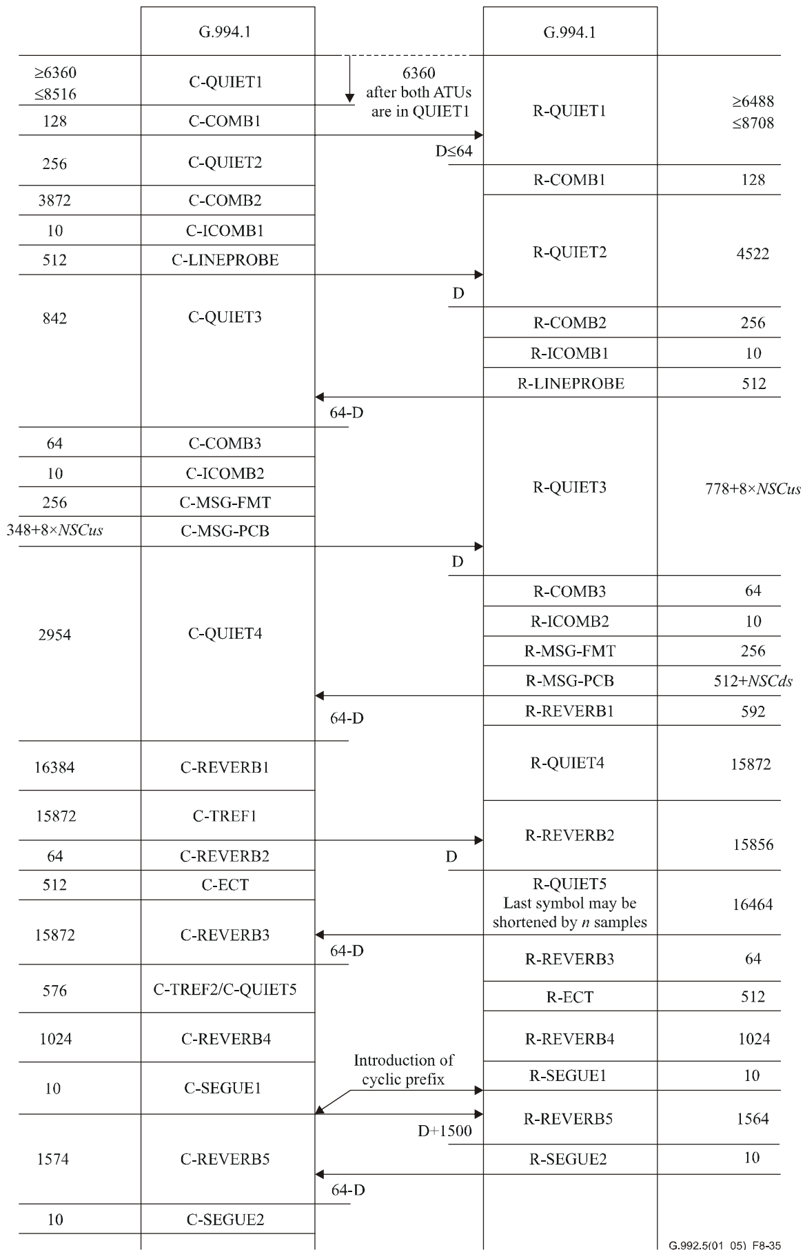
Figure 8-35/G.992.5 – Loop diagnostics timing diagram (part 1)
