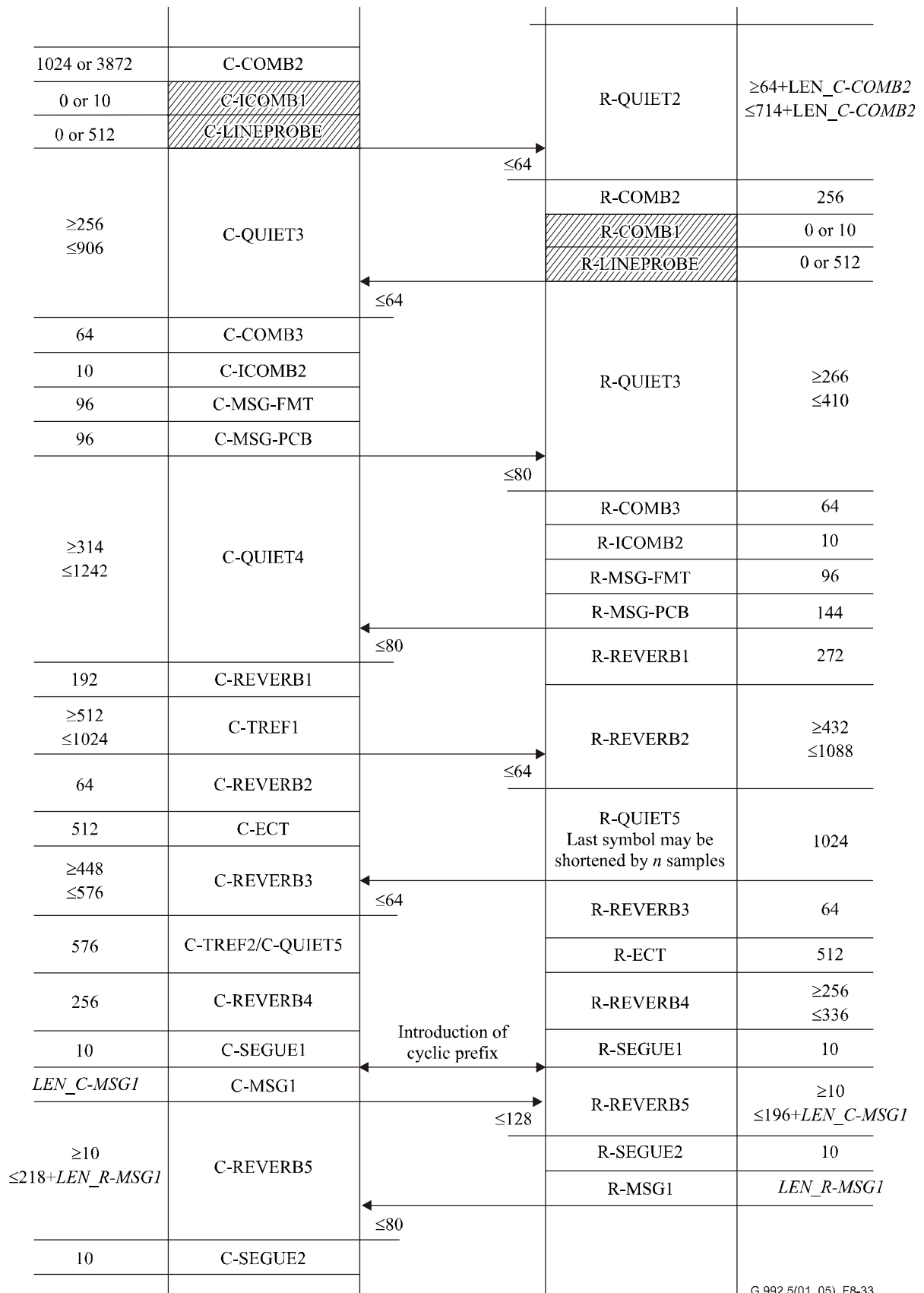
Figure 8-33/G.992.5 – Timing diagram of the short initialization procedure (part 1)
