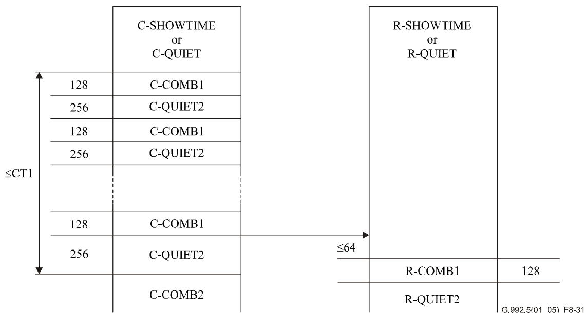
Figure 8-31/G.992.5 – Timing diagram of the entry into the short initialization procedure, ATU-C initiated
