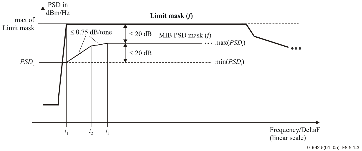
Figure 8.5.1-3/G.992.5 – Illustration of the restrictions on the MIB PSD in-band shaping
