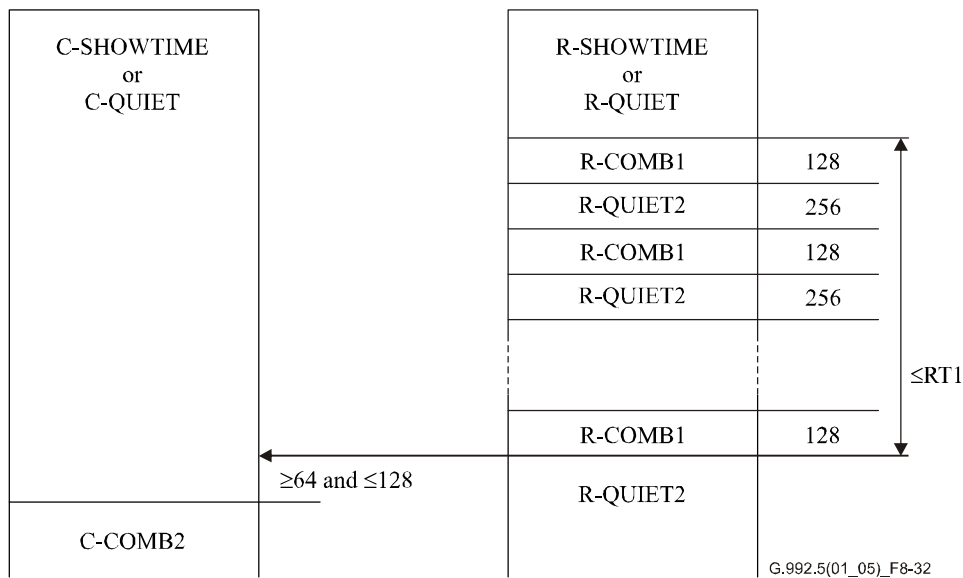
Figure 8-32/G.992.5 – Timing diagram of the entry into the short initialization procedure, ATU-R initiated
