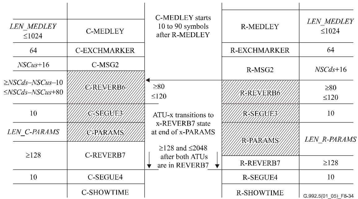
Figure 8-34/G.992.5 – Timing diagram of the short initialization procedure (part 2)
