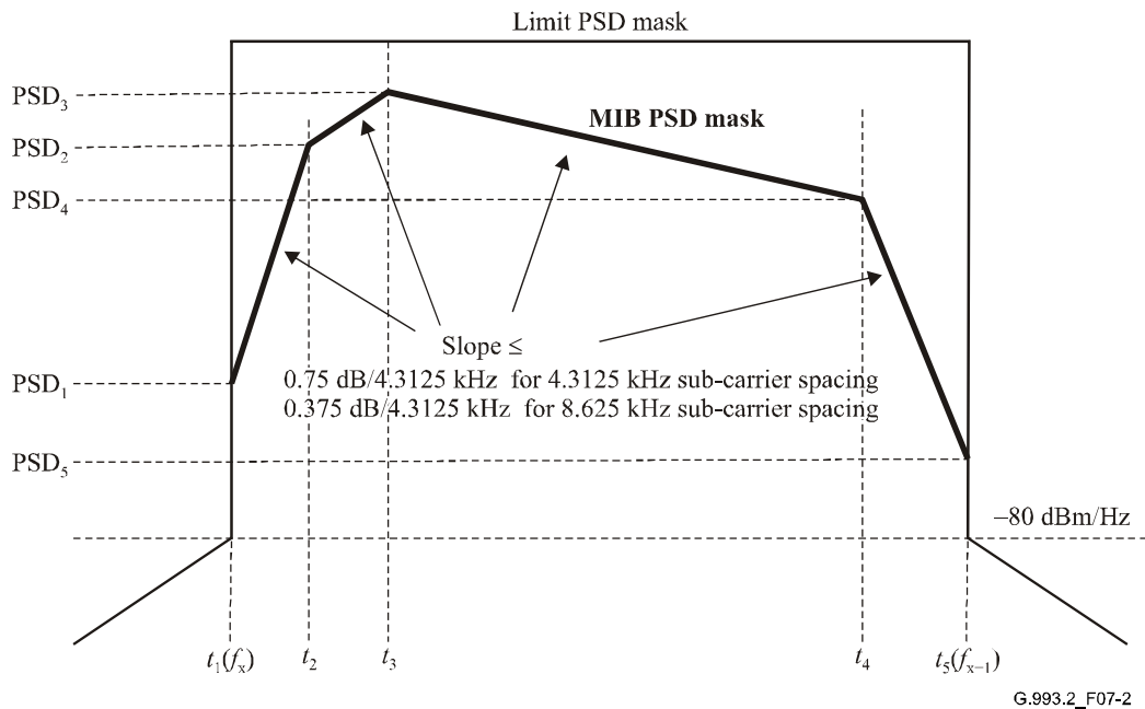
Figure 7-2 – Illustration of a MIB PSD mask in the case all breakpoint \text{PSD}_n values are greater than -80\text{ dBm/Hz}
