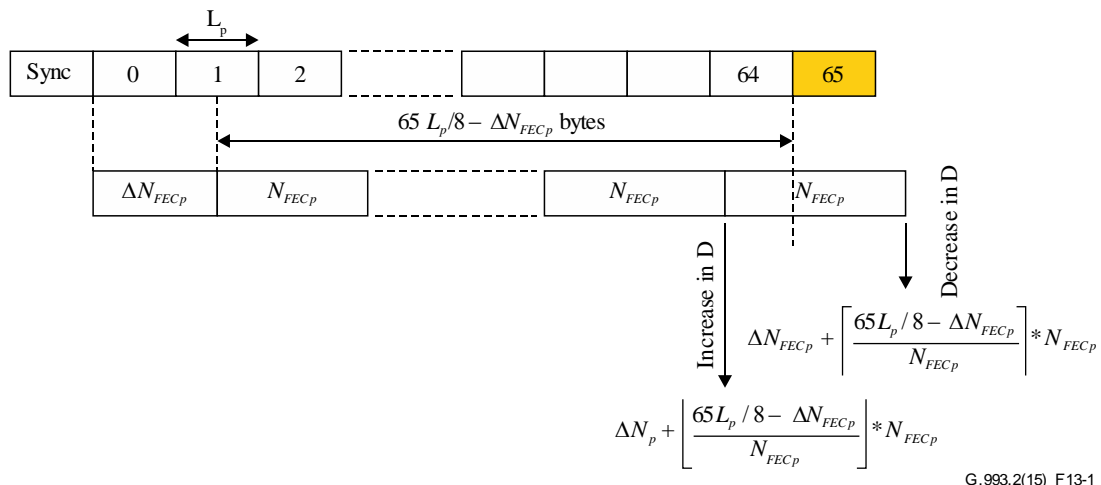
Figure 13-1 – Finding the byte where the change in D_p is activated
