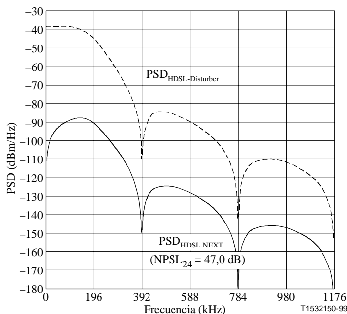
Figura 32/G.996.1 – NEXT de HDSL de 24 perturbadores
