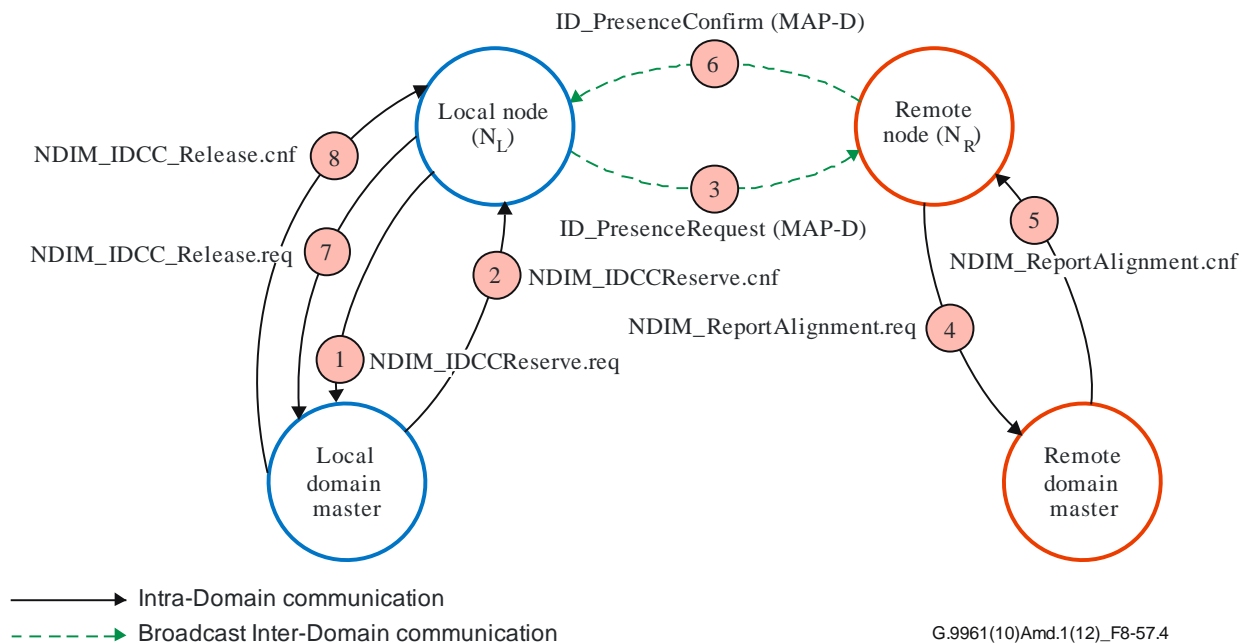
Figure 8-57.4 – Remote MAC cycle alignment procedure
