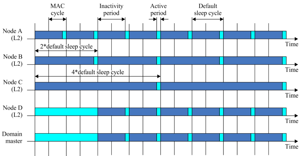
Figure 8-65.1 – Example of domain with nodes in L2 power saving mode
