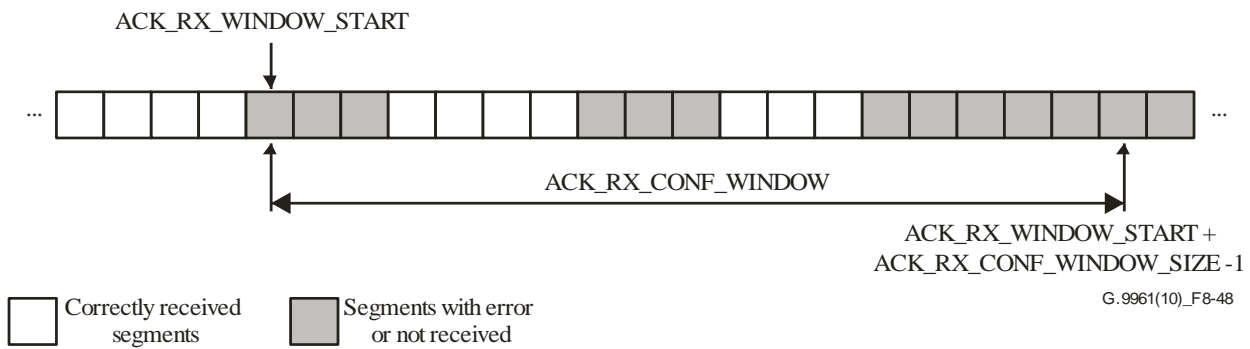
Figure 8-48 – Reception window
