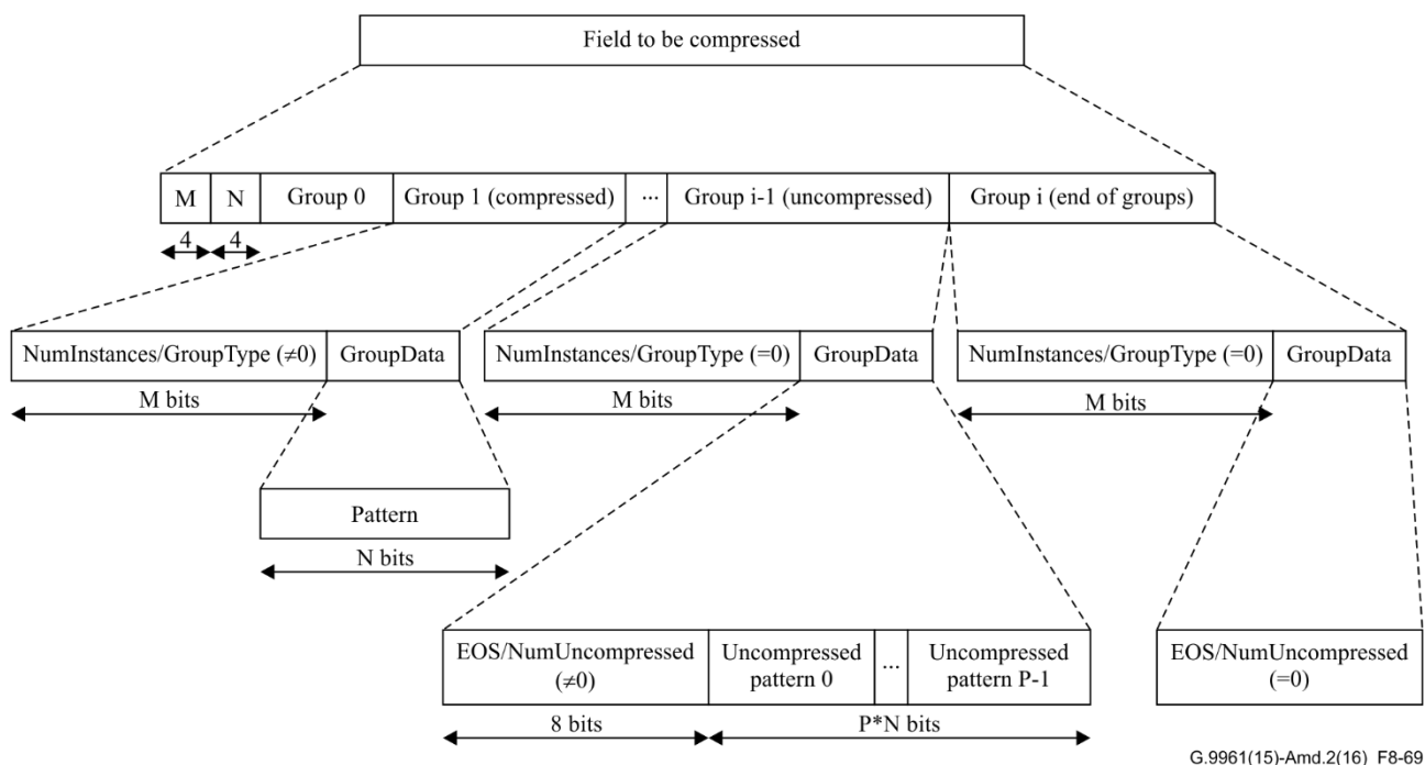
Figure 8-69 – Example of compressing a field of a management message using the run-length compression mechanism
