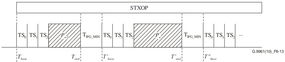
Figure 8-13 – Time slot timing
