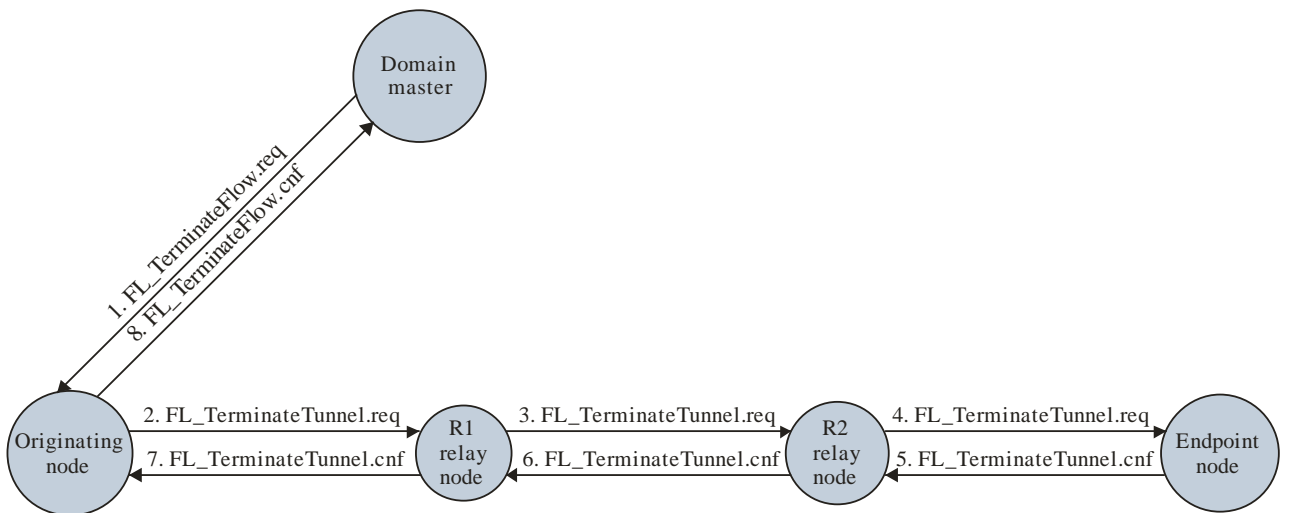
Figure 8-38.9a – Domain master triggers tunnel termination
