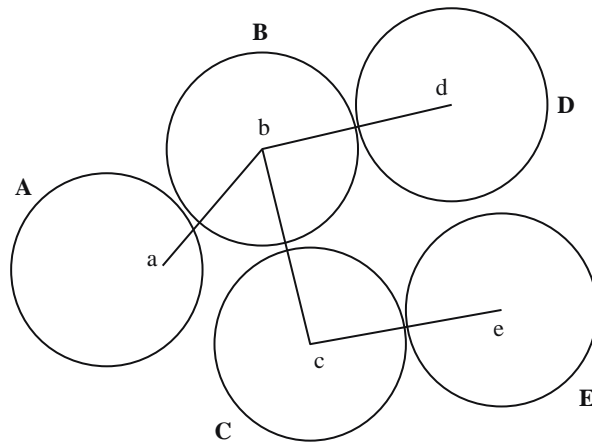
Figure 8-57.10 – Illustration of neighbouring domain coordination
