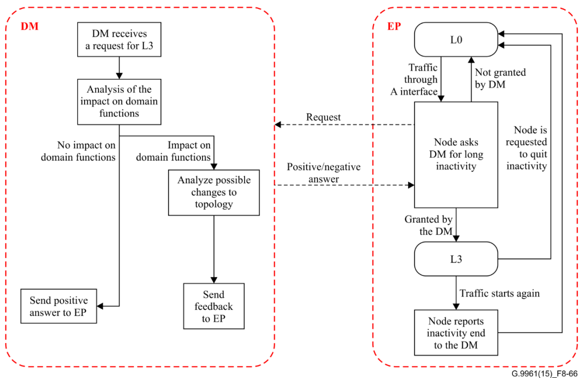
Figure 8-66 – Operation in L3 power saving mode
