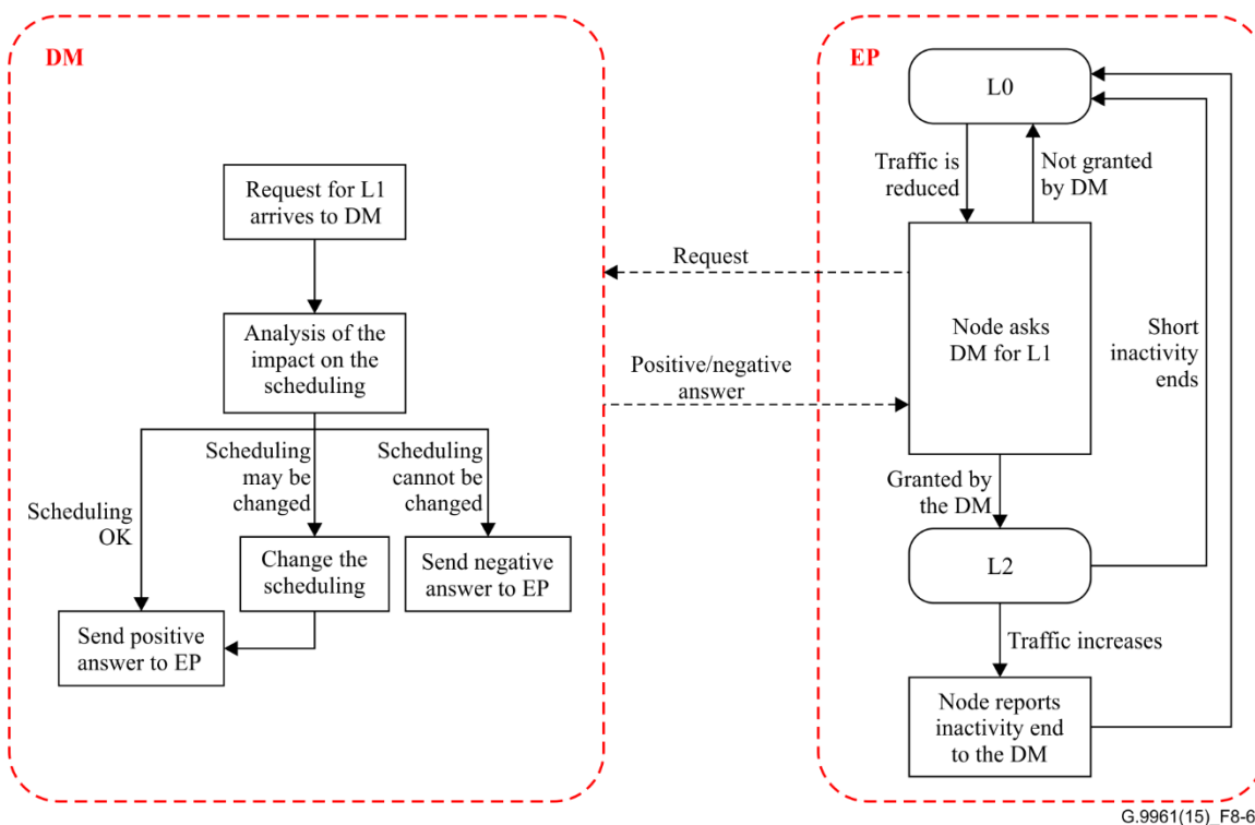
Figure 8-64 – Operation in L1 power saving mode
