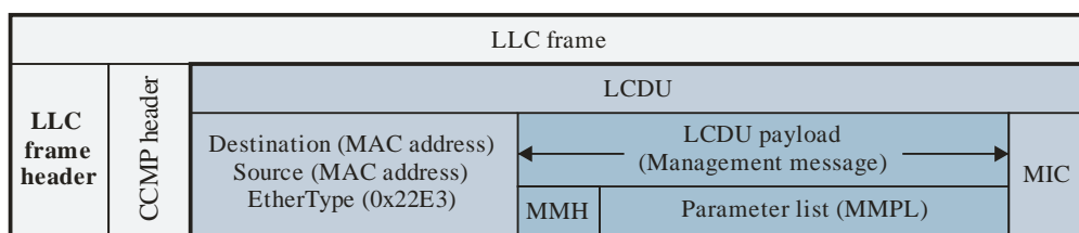
LLC frame with encrypted LCDU
