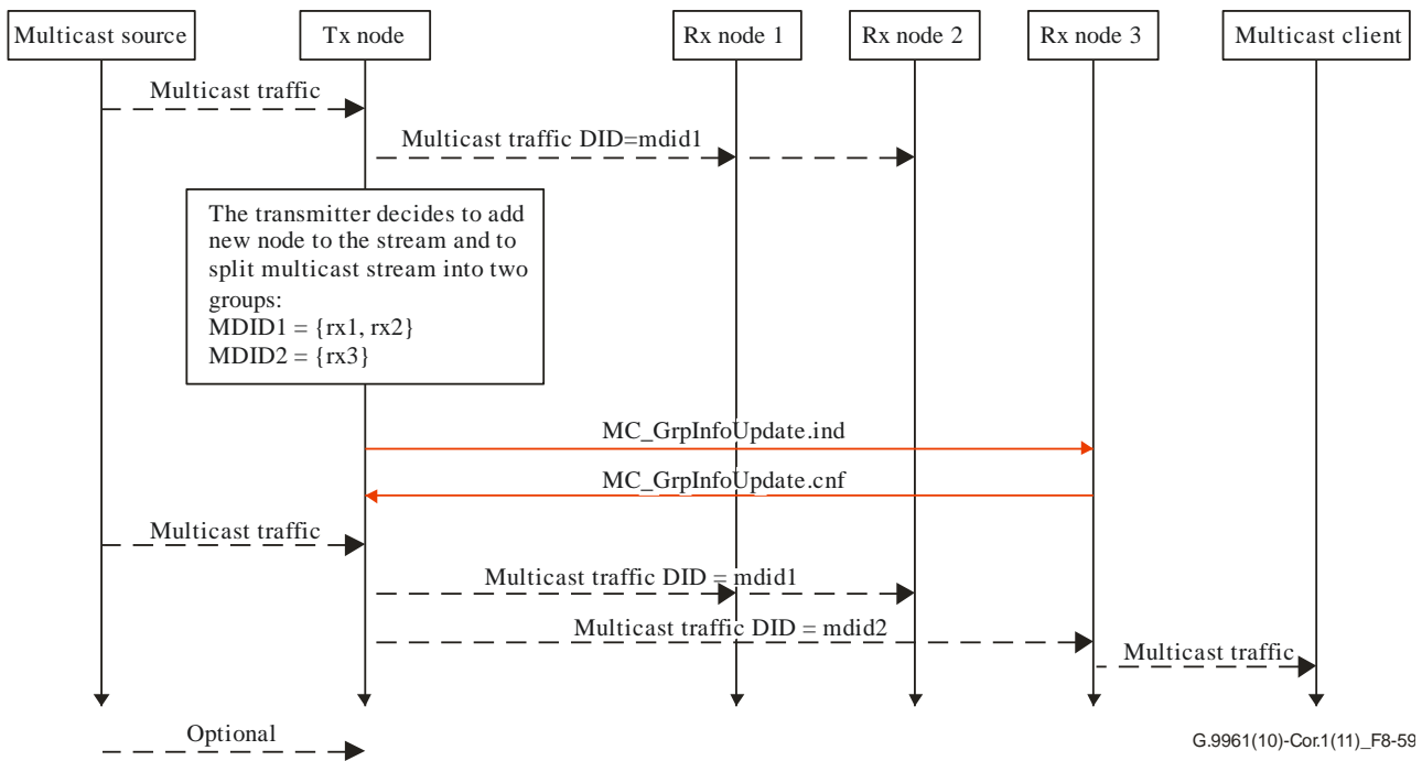
Figure 8-59 – Example of split of a PHY multicast group
