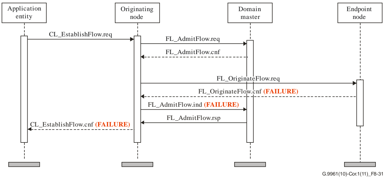
Figure 8-31 – Failure in flow establishment due to rejection by endpoint node
