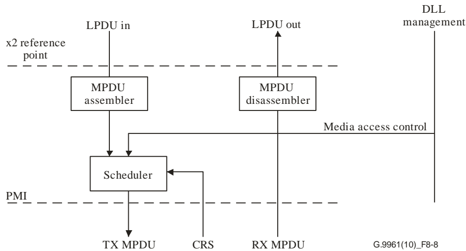
Figure 8-8 – Functional model of MAC
