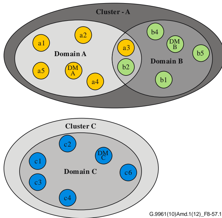
Figure 8-57.1 – Cluster definition
