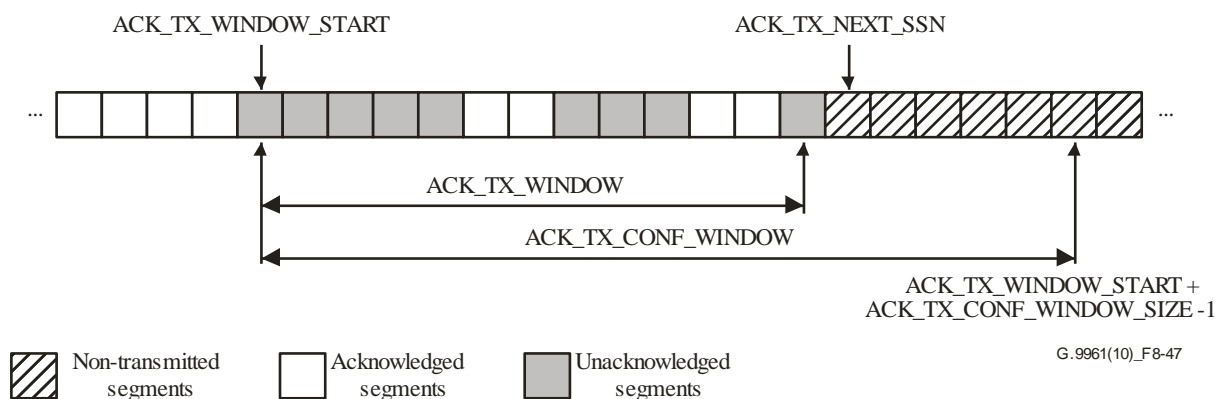
Figure 8-47 – Transmission window
