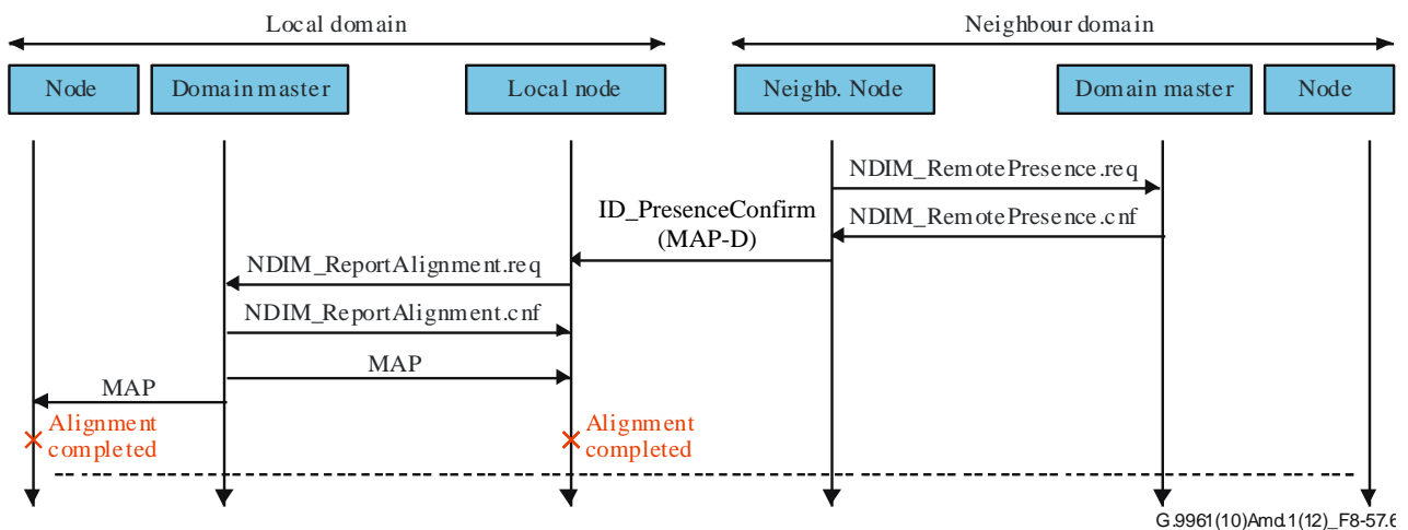
Figure 8-57.6 – Protocol diagram for local MAC cycle alignment
