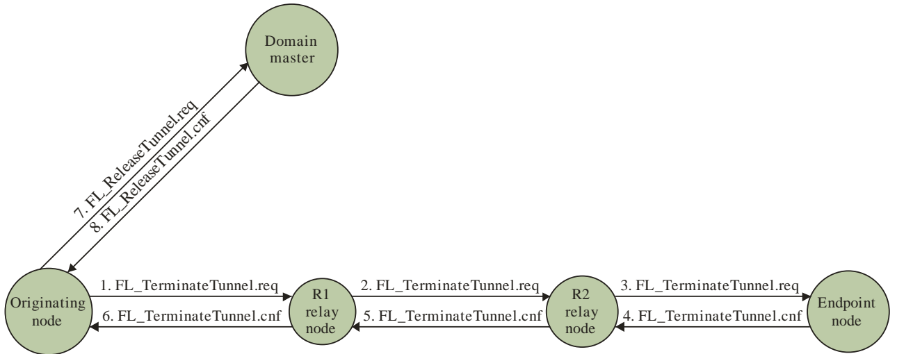
Figure 8-38.1a – Normal tunnel termination
