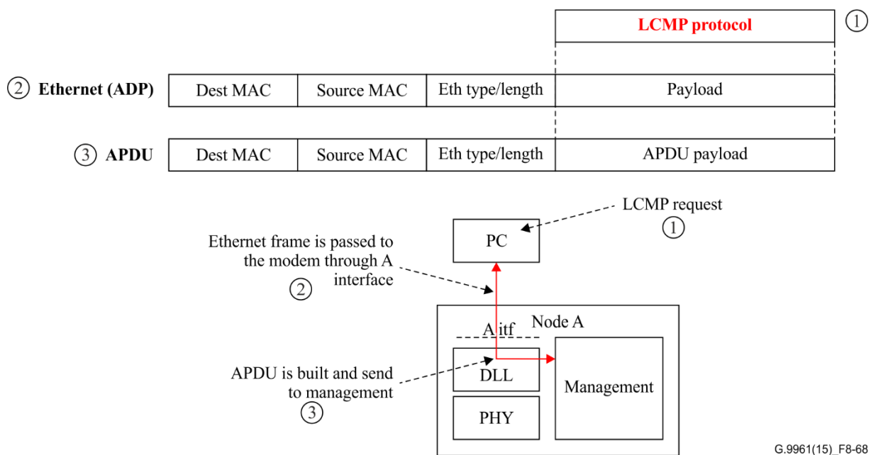
Figure 8-68 – Example of encapsulation of LCMP messages into ITU-T G.hn in-band management messages
