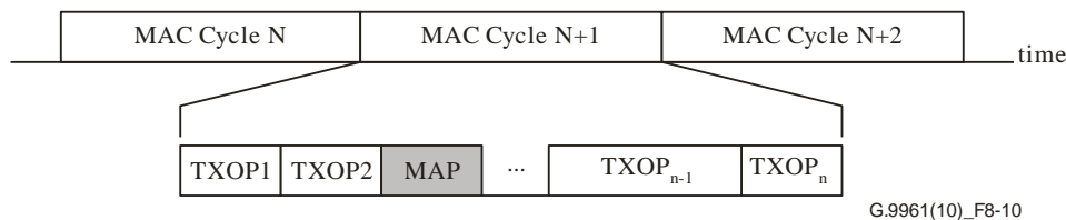
Figure 8-10 – Illustration of MAP controlled medium access
