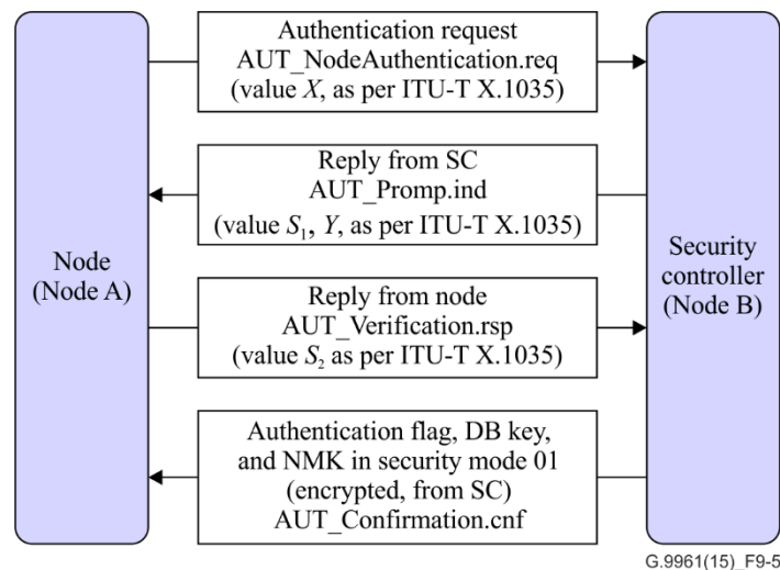
Figure 9-5 – PAK handshake procedure
