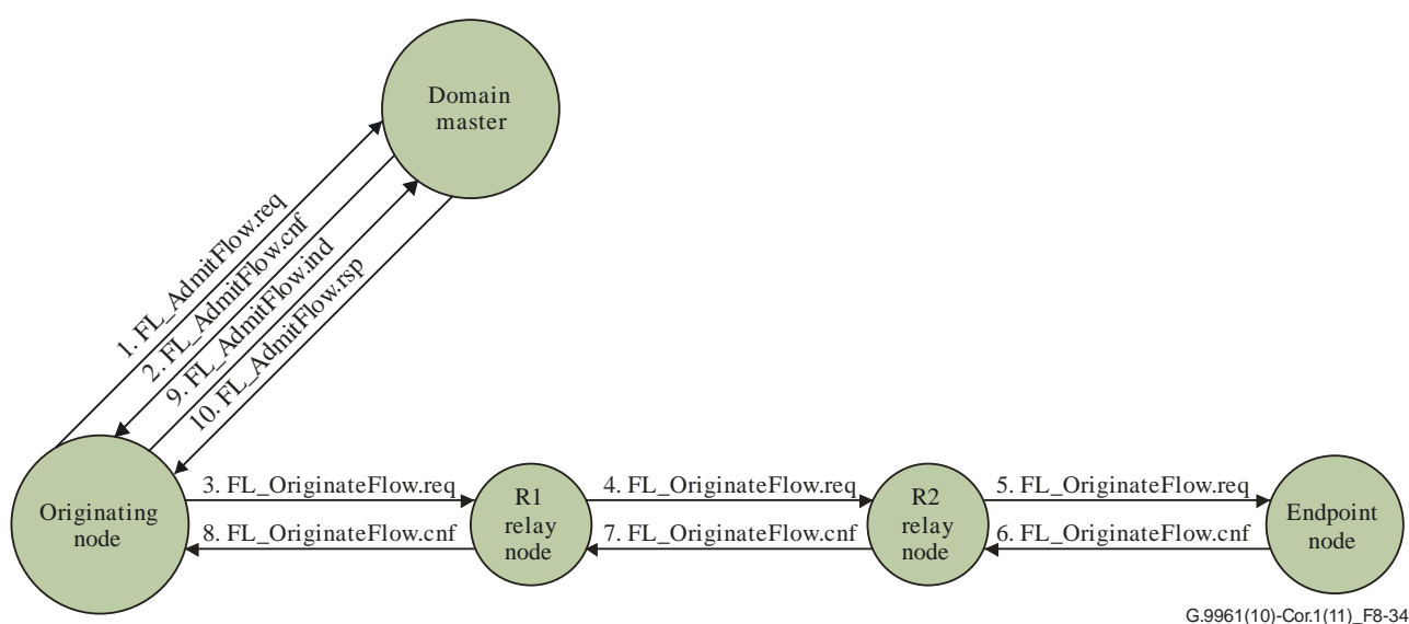
Figure 8-34 – Example of a successful tunnel establishment via two relay nodes
