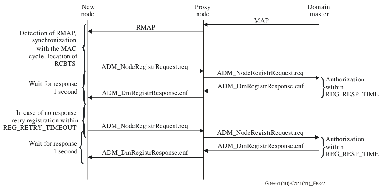
Figure 8-27 – Protocol diagram describing node registration via proxy
