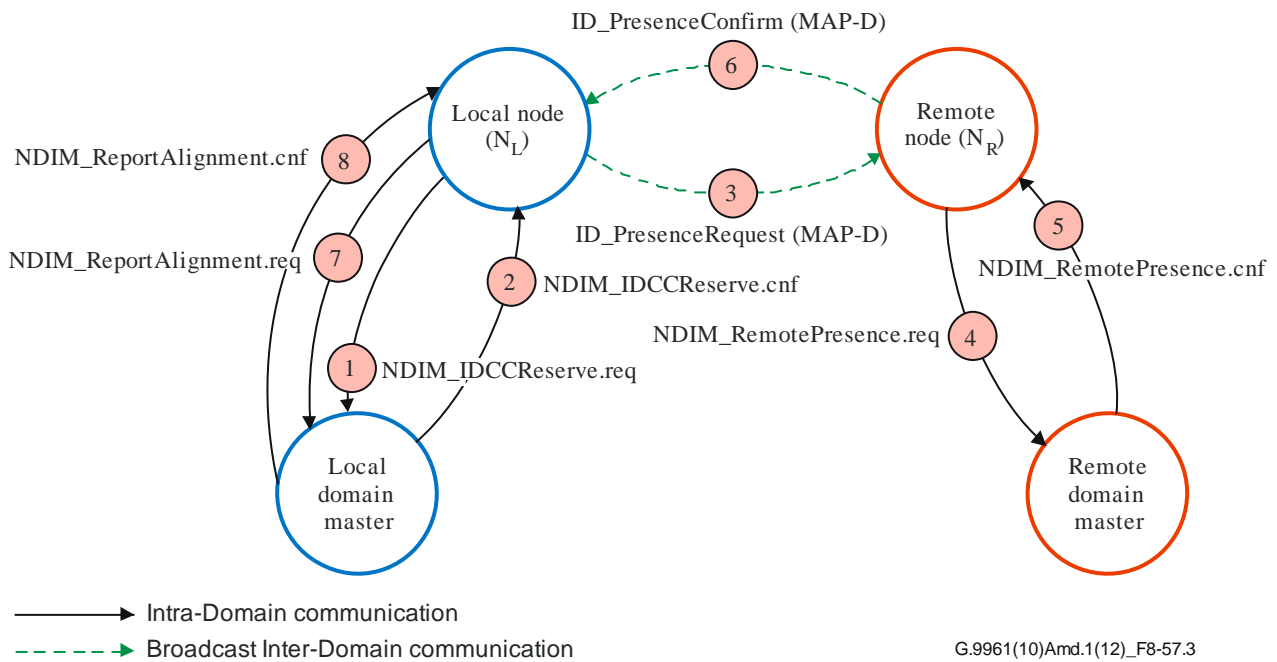
Figure 8-57.3 – Local MAC cycle alignment procedure
