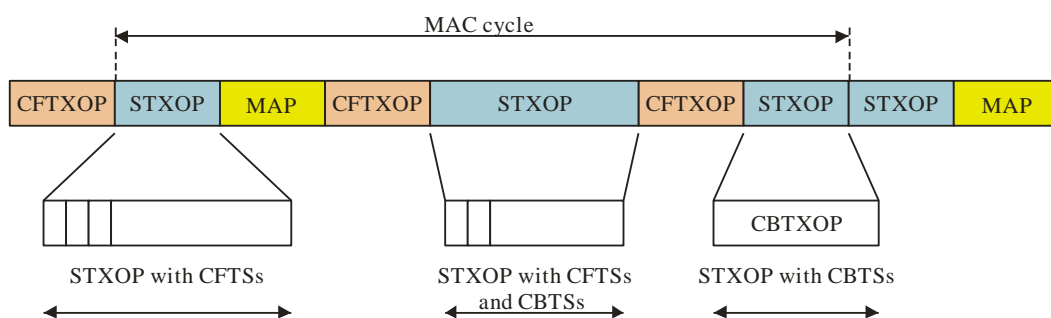
Figure 8-12 – Example of a MAC cycle structure
