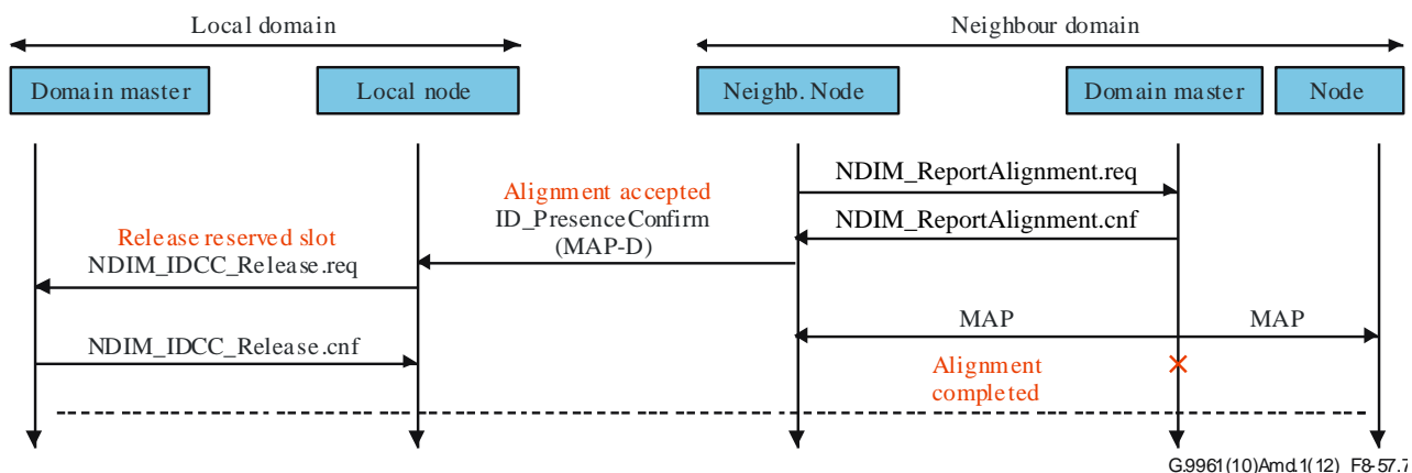
Figure 8-57.7 – Protocol diagram for remote MAC cycle alignment
