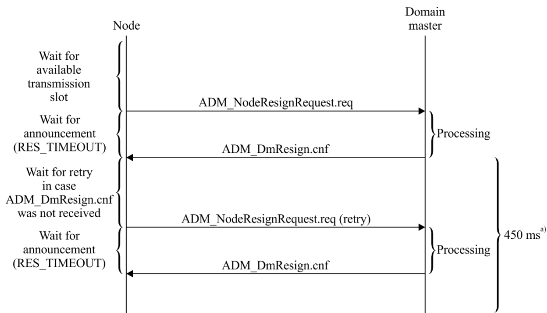
Figure 8-26 – Protocol diagram describing node resignation
