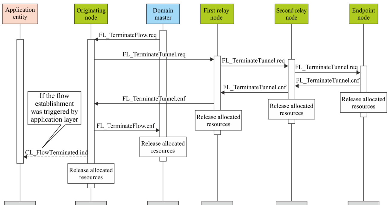
Figure 8-38.9b – MSC for tunnel termination triggered by the domain master
