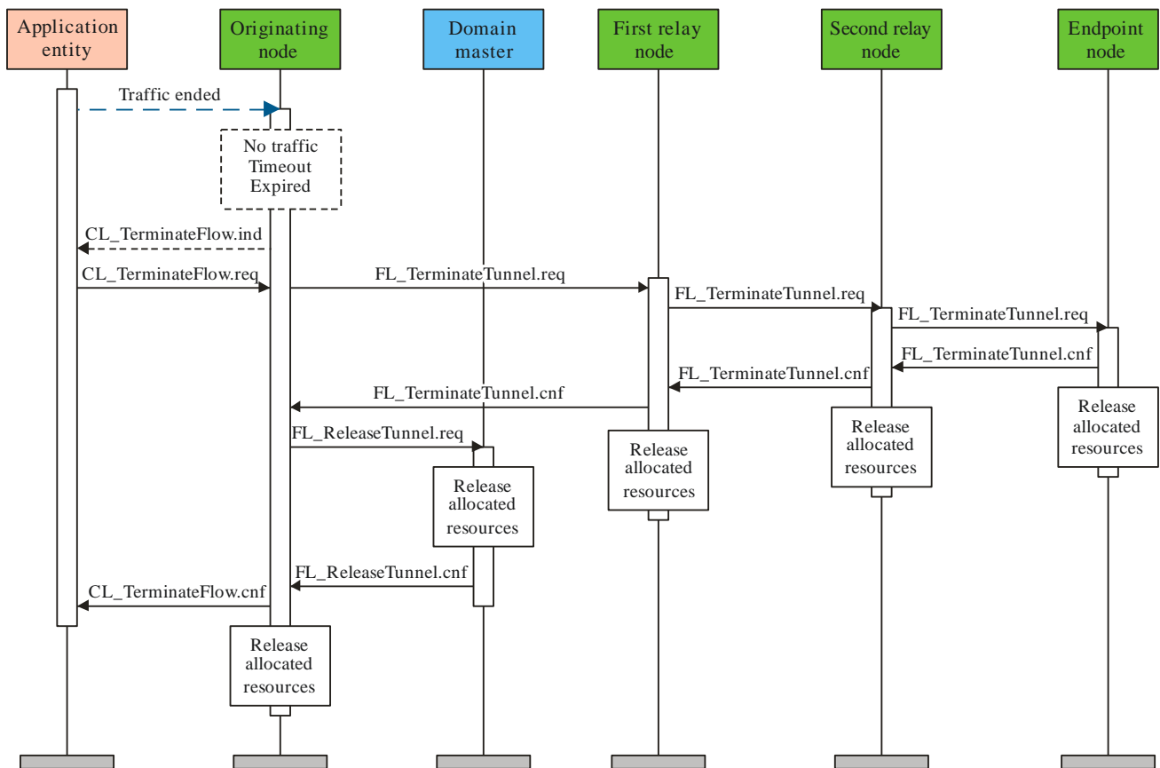
Figure 8-38.1a – Normal tunnel termination
