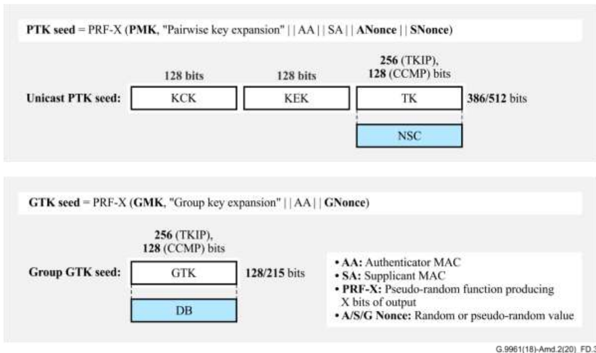
Figure D.3 – NN, DB and NSC key derivation
