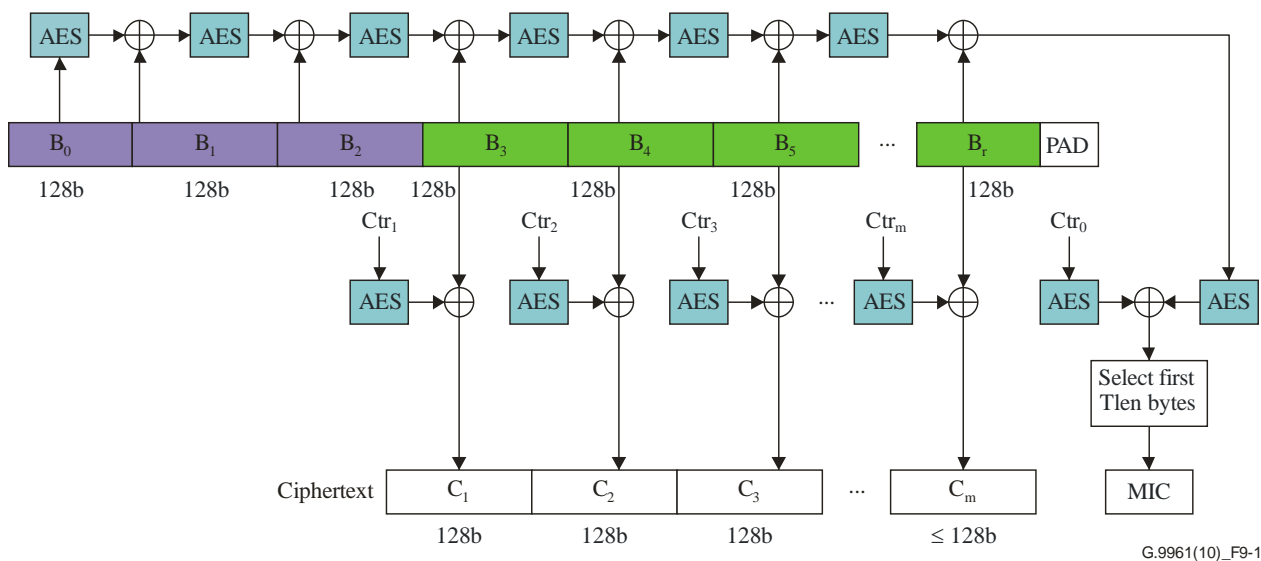
Figure 9-1 – Functional diagram of CCM encryption and message-authentication
