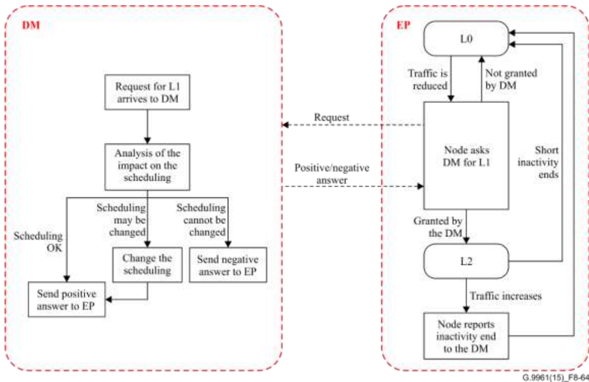
Figure 8-64 – Operation in L1 power saving mode
