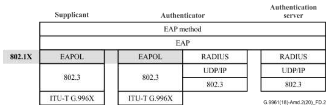
Figure D.2 – IEEE 802.1x port-based network access control over ITU-T G.9960/G.9961 network (Protocol stack)
