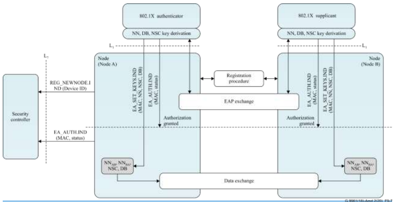
Figure 9-7 – External authentication procedure
