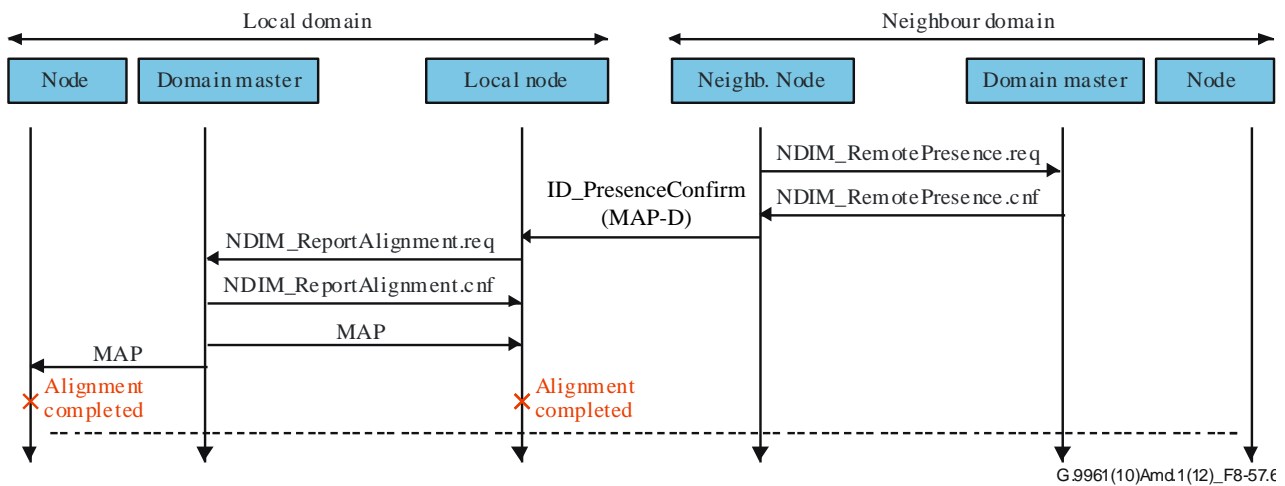
Figure 8-57.6 – Protocol diagram for local MAC cycle alignment
