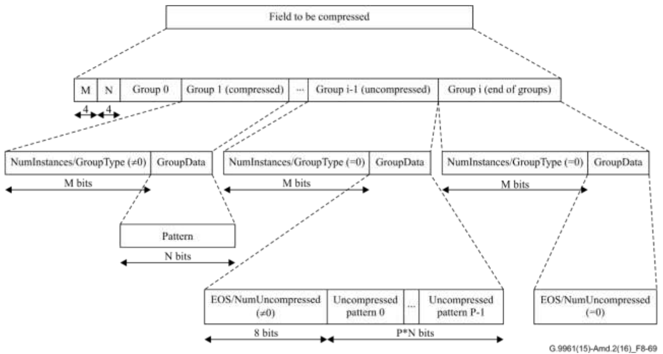
Figure 8-69 – Example of compressing a field of a management message using the run-length compression mechanism
