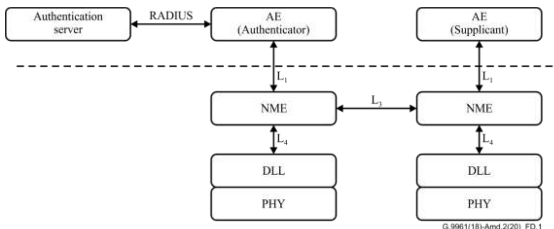
Figure D.1 – IEEE 802.1x port-based network access control over a domain
