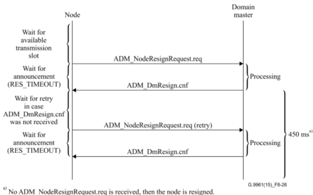
Figure 8-26 – Protocol diagram describing node resignation
