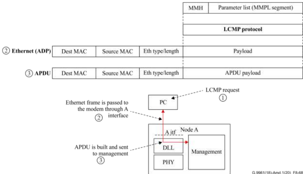
Figure 8-68 – Example of encapsulation of LCMP messages into ITU-T G.hn in-band management messages
