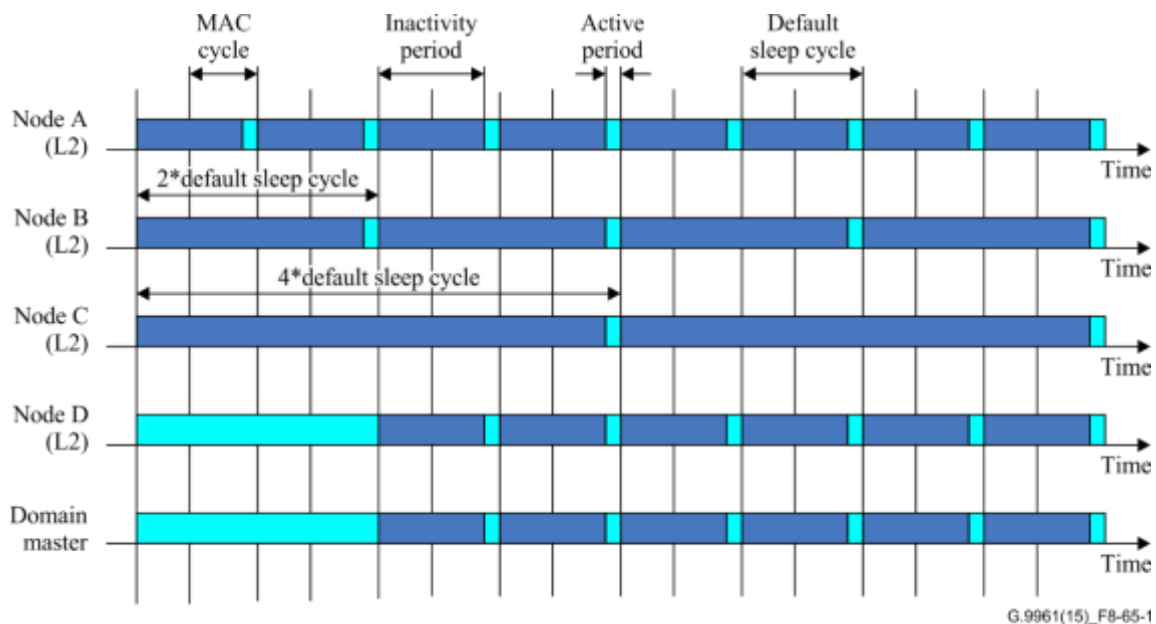
Figure 8-65.1 – Example of domain with nodes in L2 power saving mode
