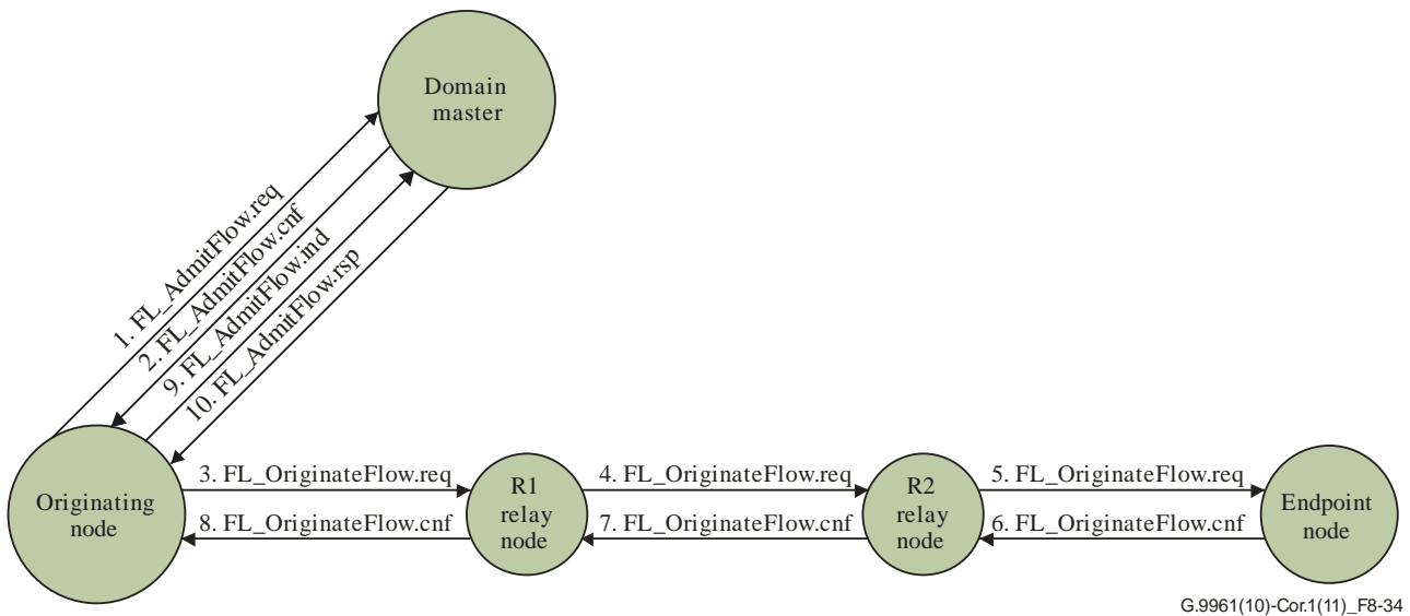
Figure 8-34 – Example of a successful tunnel establishment via two relay nodes
