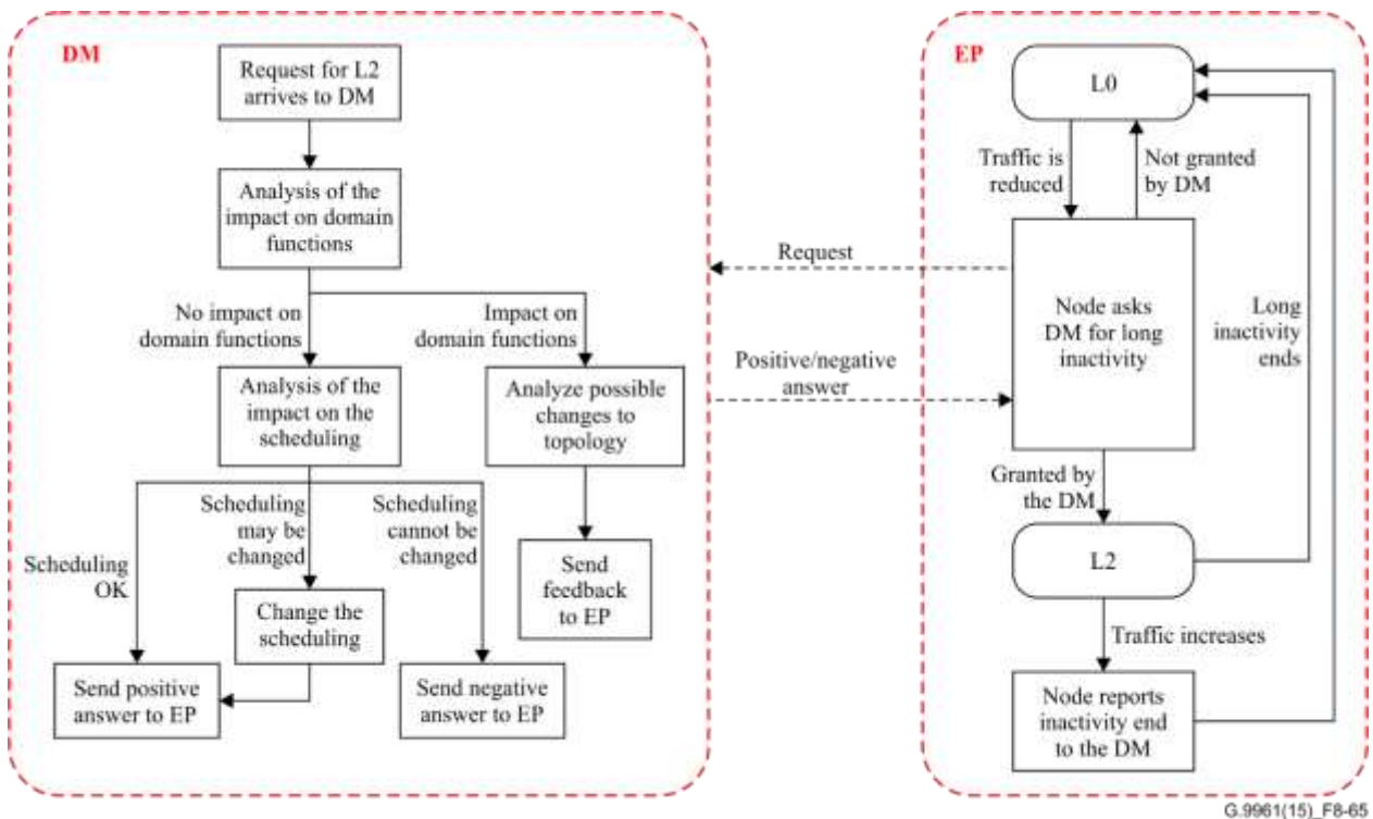
Figure 8-65 – Operation in L2 power saving mode
