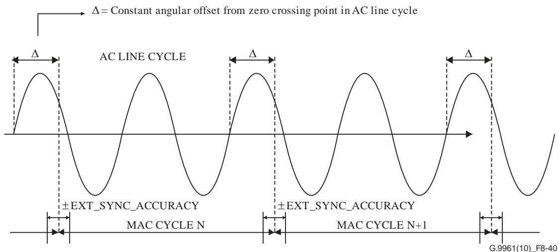
Figure 8-40 – Relationship between the AC line cycle and the MAC cycle when the duration of the MAC cycle is 2 AC cycles
