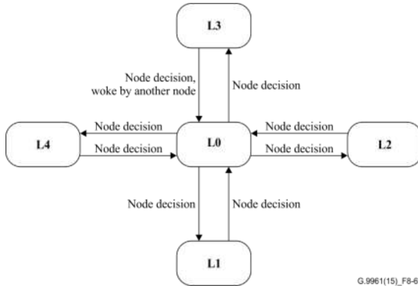
Figure 8-63 – Allowed transitions for node power saving modes
