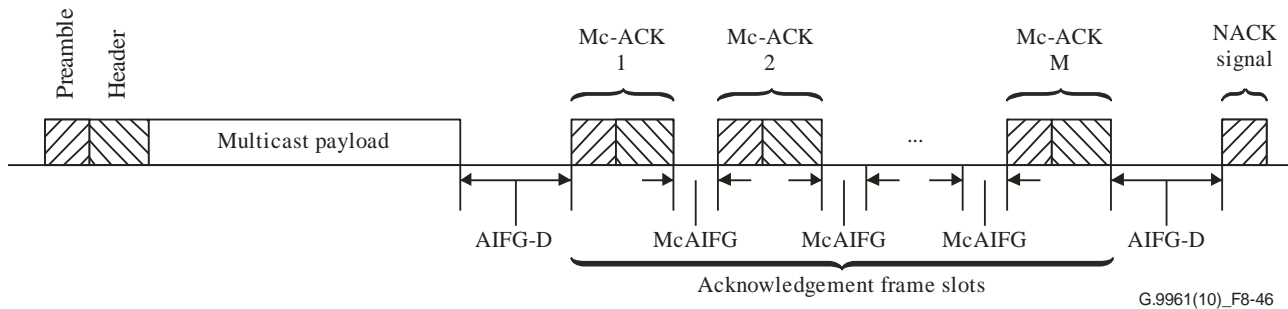
Figure 8-46 – Multicast acknowledgment with NACK signalling
