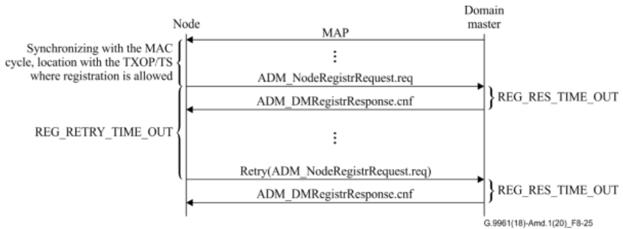
Figure 8-25 – Protocol diagram describing node registration
