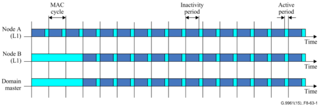
Figure 8-63.1 – Example of domain with nodes in L1 power saving mode
