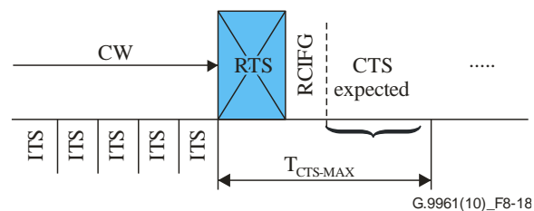
Figure 8-18 – Example of CTS not detected when RTS/CTS is used
