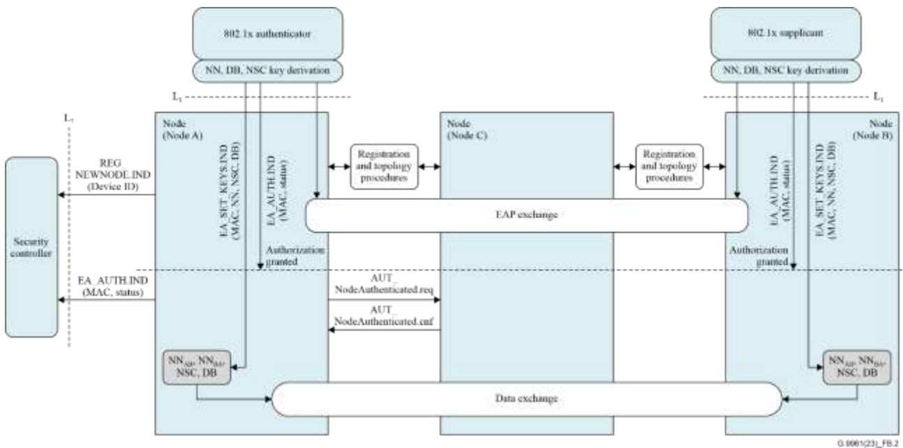
Figure B.2 – External authentication procedure via proxy for smart grid
