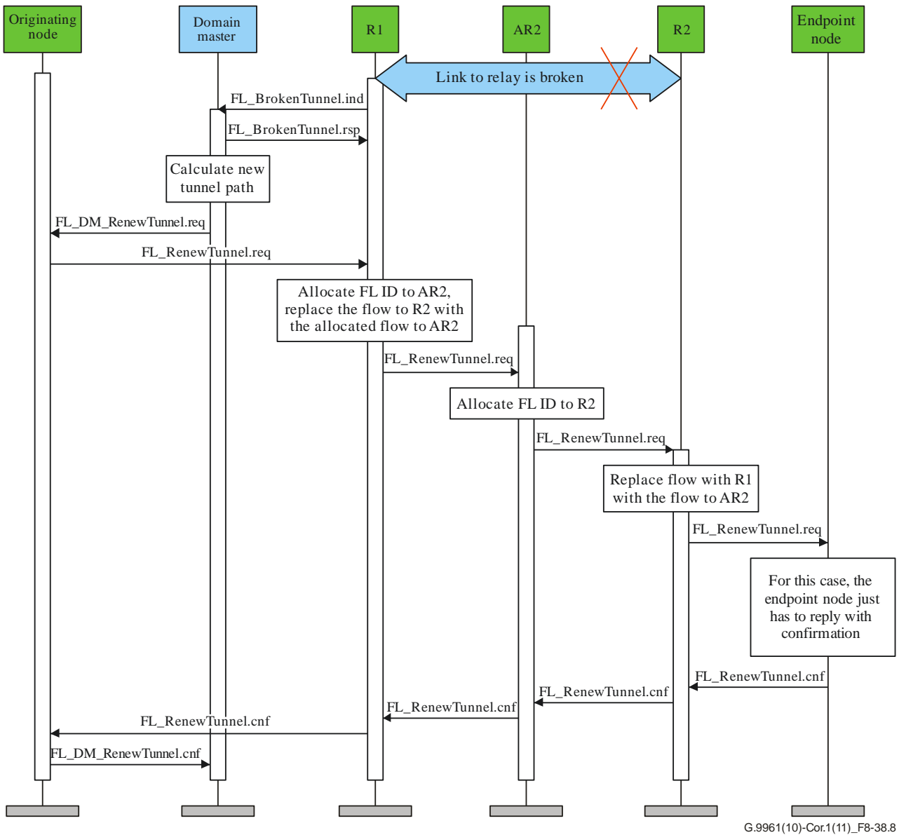
Figure 8-38.8 – MSC of tunnel renewal due to a broken link case 4
