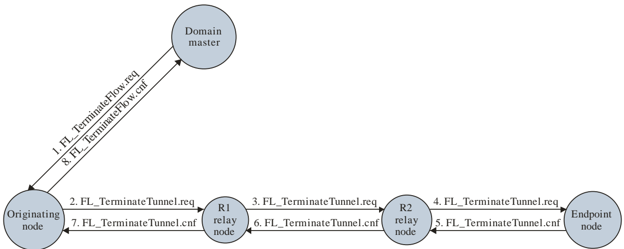
Figure 8-38.9a – Domain master triggers tunnel termination
