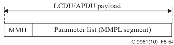
Figure 8-54 – Format of a management message
