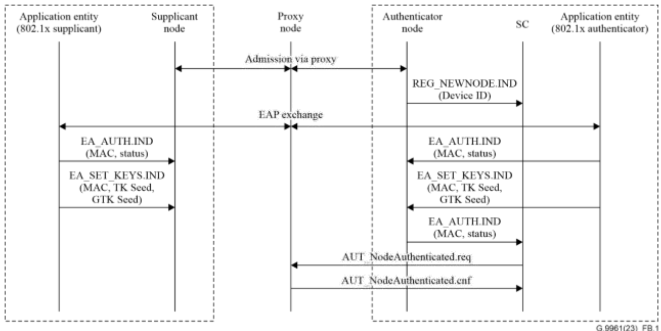
Figure B.1 – Flow diagram for the external authentication procedure via proxy for smart grid
