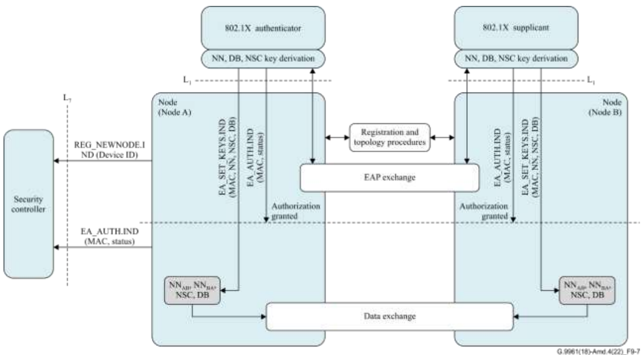
Figure 9-7 – External authentication procedure
