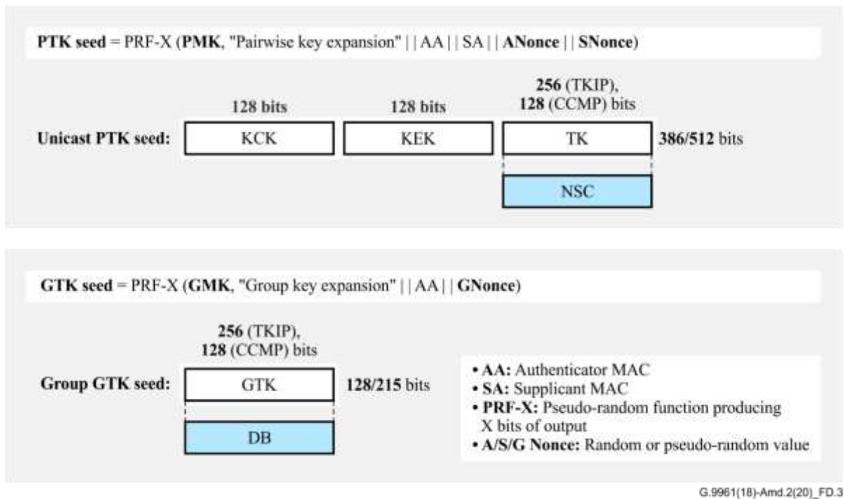
Figure D.3 – NN, DB and NSC key derivation
