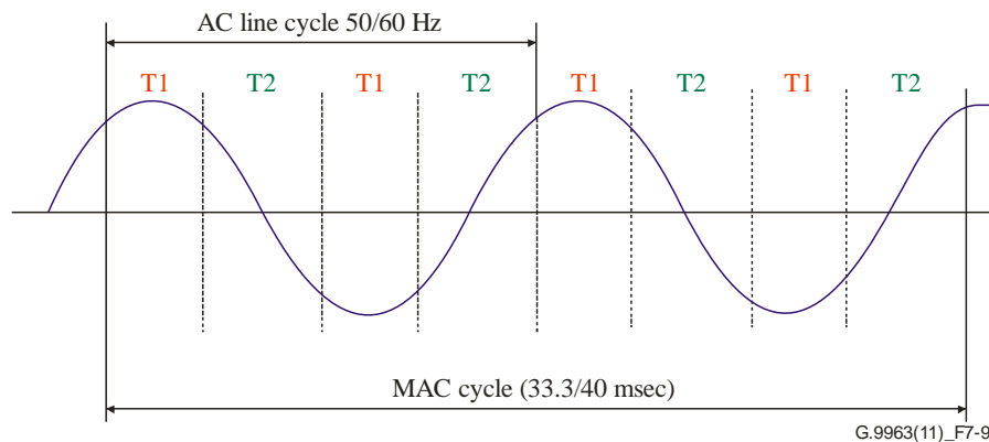
Figure 7-9 – An example of BMAT regions in a MAC cycle for a power line
