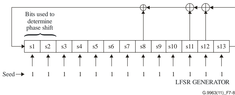
Figure 7-8 – Constellation scrambler
