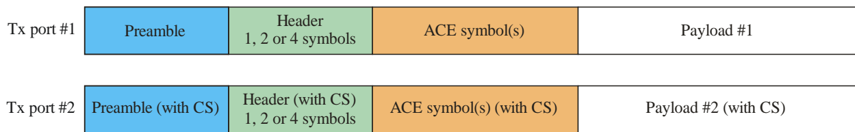
Figure 7-3 – Format of the PHY frame in a MIMO transmission
