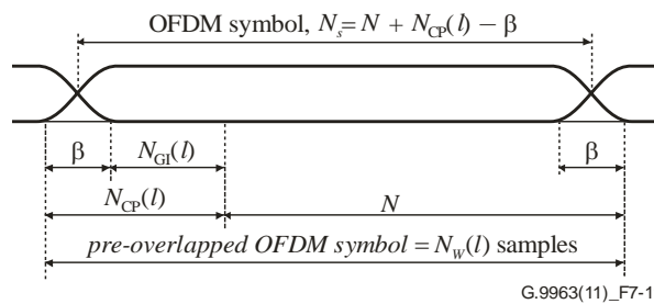
Figure 7-11 – Structure of an OFDM symbol with cyclic extension and overlapped windowing
