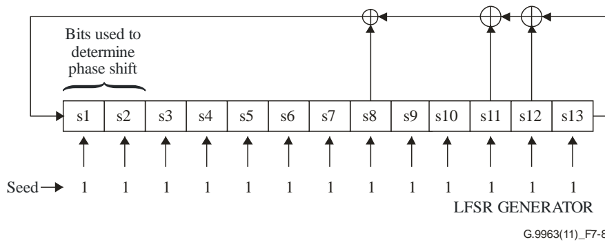
Figure 7-8 – Constellation scrambler
