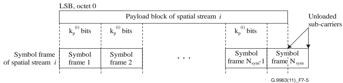
Figure 7-5 – Payload segmentation of the payload block of spatial stream i ( i = 1,2 )
