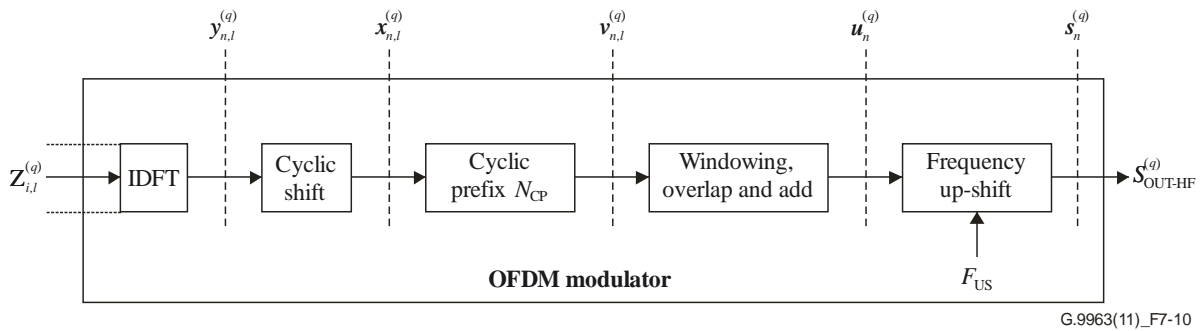
Figure 7-10 – Functional model of the OFDM modulator
