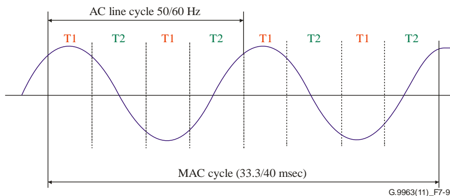
Figure 7-9 – An example of BMAT regions in a MAC cycle for a power line
