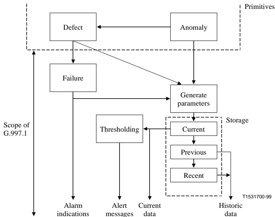
Figure 10/G.997.1 – In-service performance monitoring process
