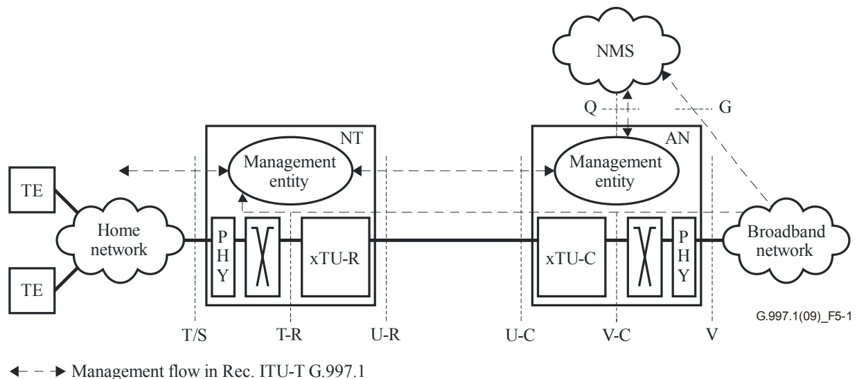
Figure 5-1 – System reference model
