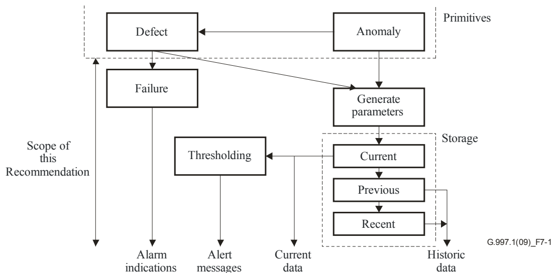
Figure 7-1 – In-service performance monitoring process
