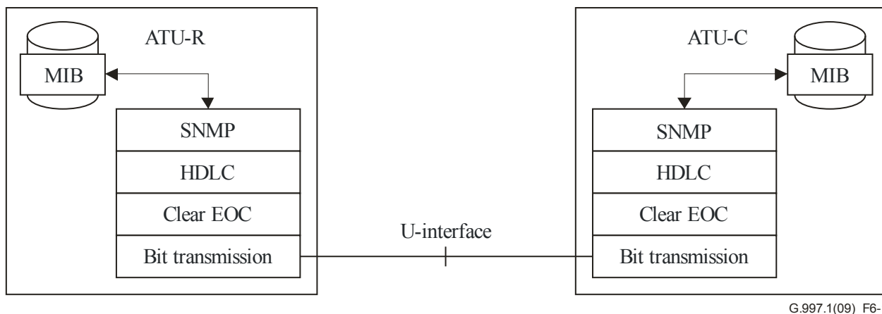
Figure 6-1 – OAM communication channel layers for bit-oriented clear EOC
