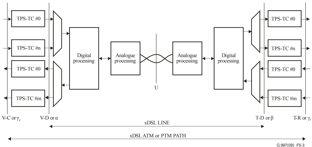
Figure 5-3 – xDSL LINE and xDSL ATM or PTM PATH definition
