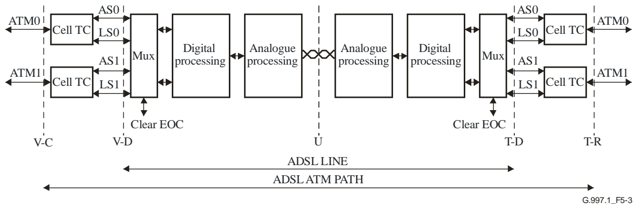
Figure 5-3 – xDSL LINE and xDSL ATM or PTM PATH definition
